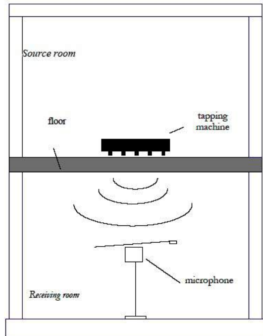
Figure 2.13: Laboratory measurement of impact sound insulation.
