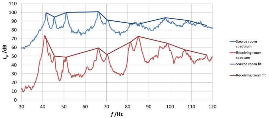
Figure 4.9: Envelope of source room resonant frequencies.
