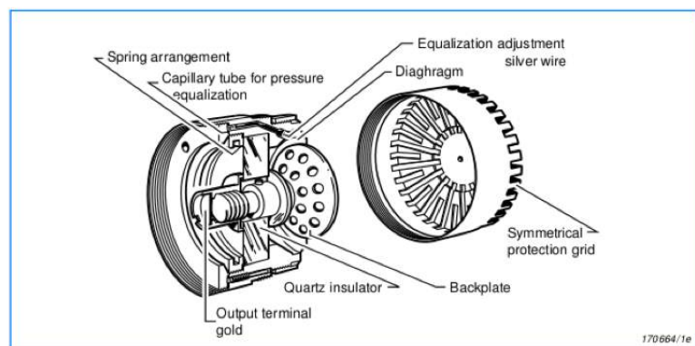
Figure 3.1: Microphone B&K 4165.
