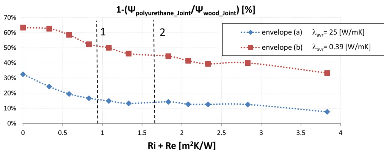
Figure 9. Difference between \psi values for wood and polyurethane joints considering (a) and (b) envelopes (1000 mm × 600 mm VIP panel).
