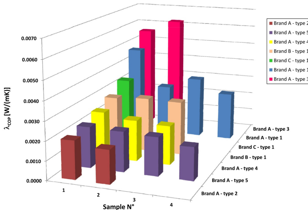
Figure 2. Measured values of the \lambda_{\text{COP}} for various samples.
