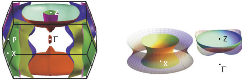
Figure 5.4: The Fermi surface of Ca(Fe_{1-x}Co_x)_2As_2 with x=0.06 as evaluated by first principle calculations and the the representation of the analytical expression used in the 3D-BTK model to fit the experimental conductance curves ( solid surfaces ) with the amplitude of the corresponding energy gap ( gridded surfaces ).
