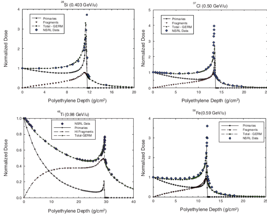
Figure 1.12: Comparisons of the GERMCODE with QMSFRG cross sections to NSRL measurements for the depth dose in polyethylene for nearly monoenergetic 56 Fe (0.59 GeV/n), 48 Ti (0.98 GeV/n), 37 Cl (0.5 GeV/n) and 28 Si (0.403 GeV/n) nuclei [96].
