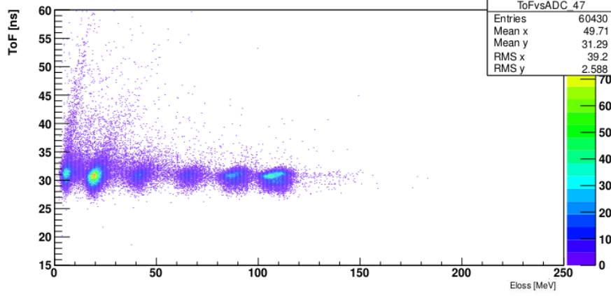
Figure 3.19: ToF vs E_{lost} plot for a central slat. The 6 spots, corresponding to different ions, are clearly distinguishable.
