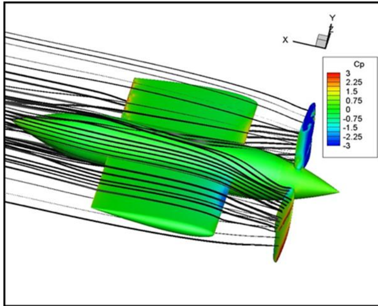
Figure 28: Slipstream around the propeller for J=1.43
