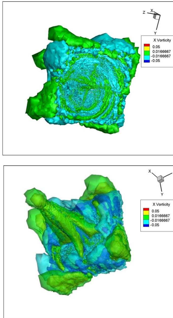
Figure 22: X-vorticity around the propeller for J=1.8
