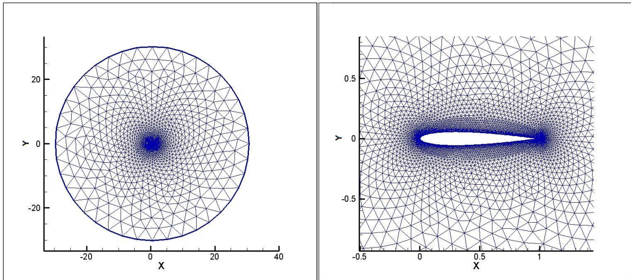
Figure 4: Mesh: a) wide- view, b) close- view
