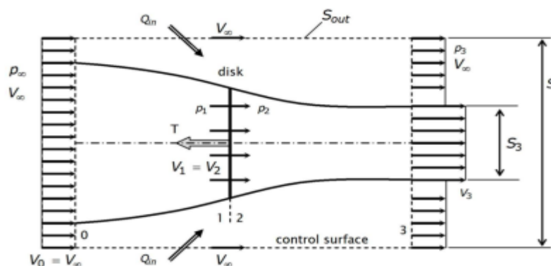
Figure A.2: Actuator disk model with control volume for the application of the momentum equation
