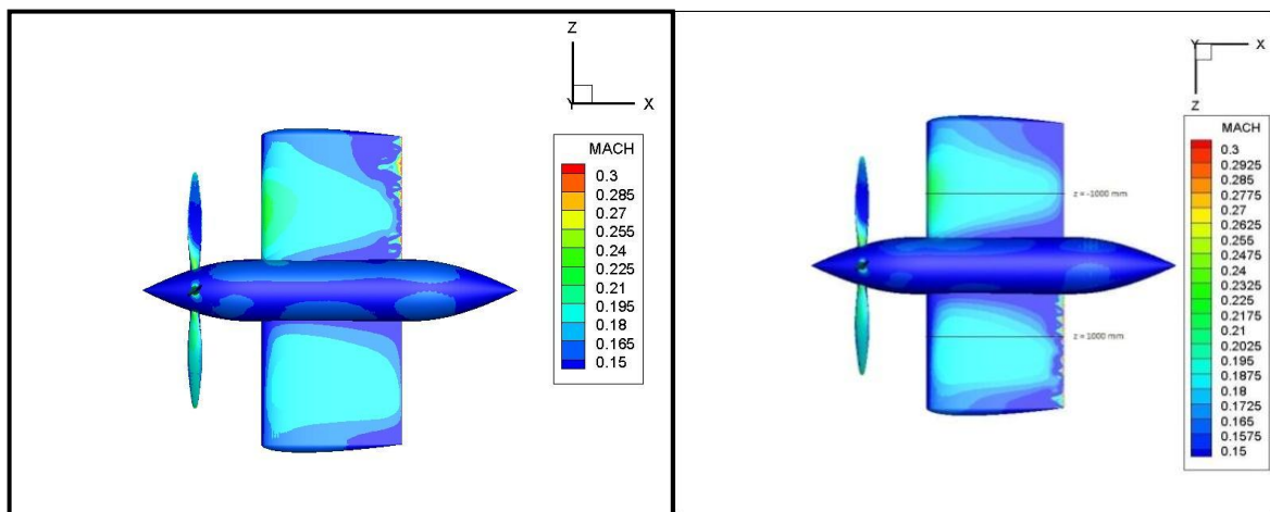
Figure 28: Slipstream around the propeller for J=1.43
