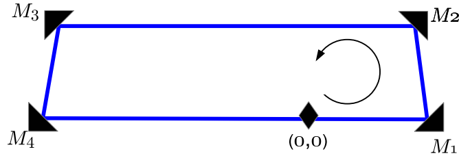
FIG. 7: CCW rays path, as seen in the observer's frame: both emission and reception take place at the origin (0,0) . To draw the figure, we chose \beta = 20/101 , so that \gamma = 101/99 , and b = a/4 .
