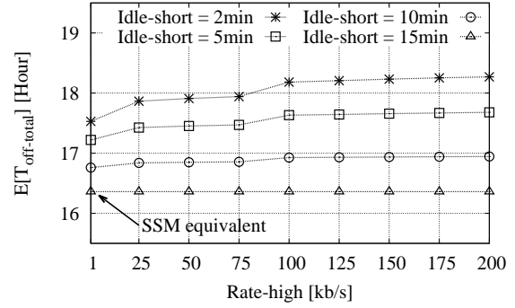
Figure 22: Comparison of the average duration of total silent time T_{off-total} using the 2SM policy with Rate-low = 1 kb/s and T_{active} = 2 min.
