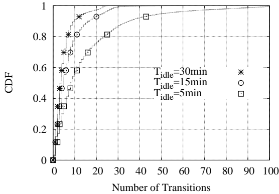
Figure 21: CDF of the number of transitions N_{trans} from sleep to ON state using the SSM policy with MinRate = 1 kb/s and different settings of Idle .
