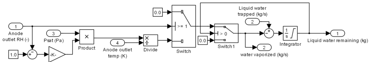
Figure 3.13 Liquid water accumulation block diagram
