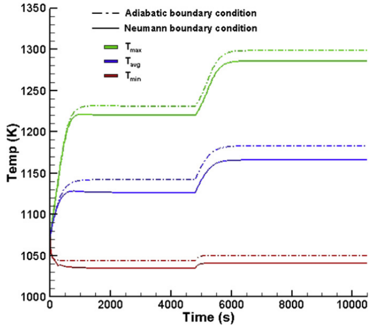
Figure 3.2 SOFC thermal response under a step current density variation. Different boundary conditions and temperatures are shown.
