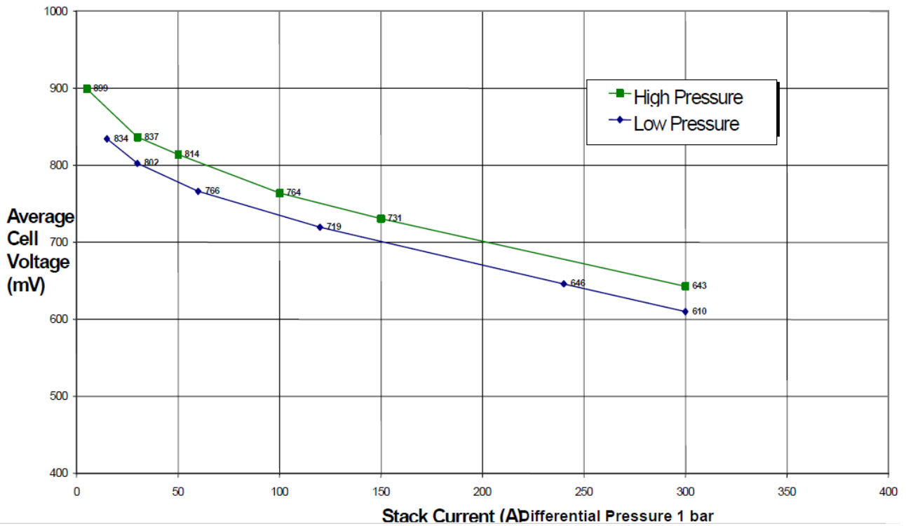
Figure 4.3 Ballard Mark 9 TM SSL polarization curve
