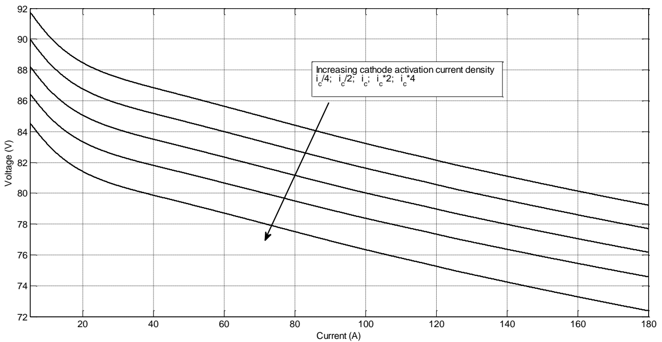
Figure 4.47 Stack voltage vs. current. i_{0c} variation. Multiplication and division by 2 and 4
