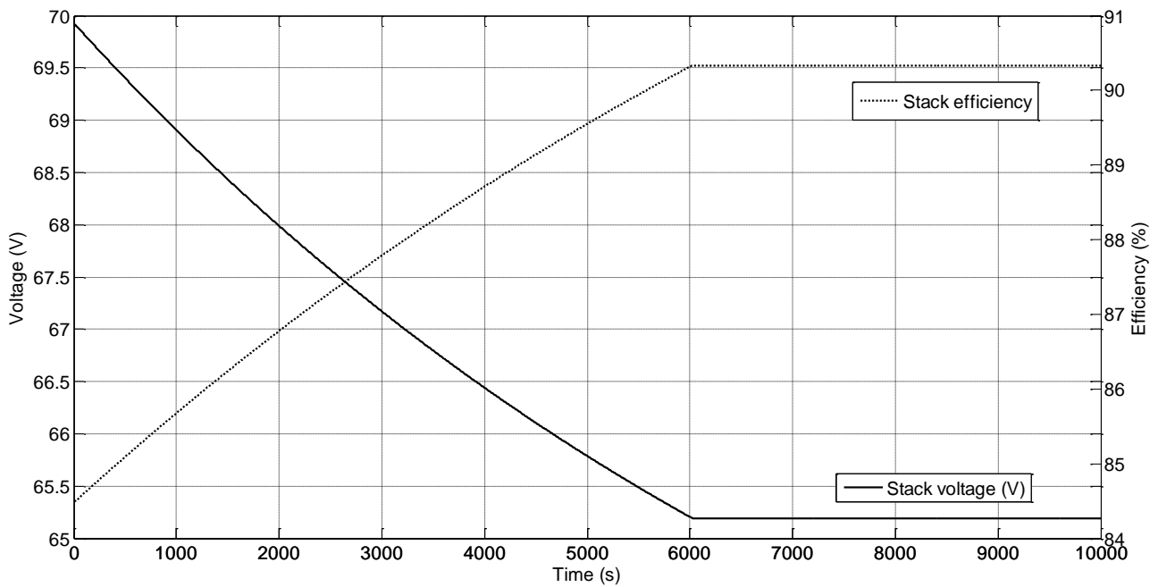
Figure 4.57 Stack voltage and efficiency. Current = 375 A. T = 80°C. P = 1.01325 bar. Initial temperature set at 51.6°C
