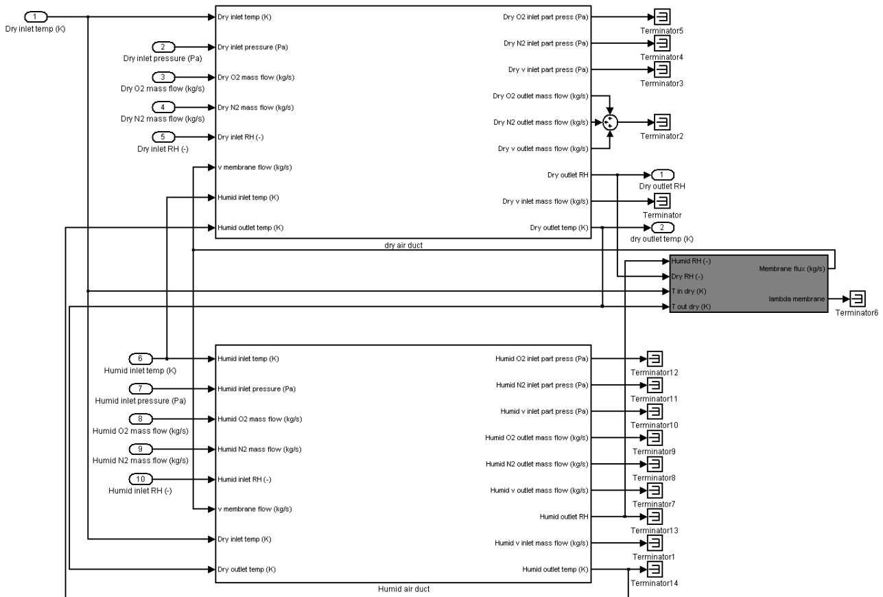
Figure 3.39 Cathode humidifier layout
