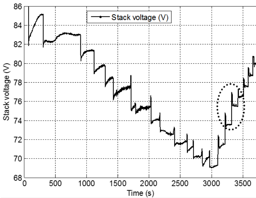
Figure 4.6 Ballard Mark9 SSL experimental stack output voltage
