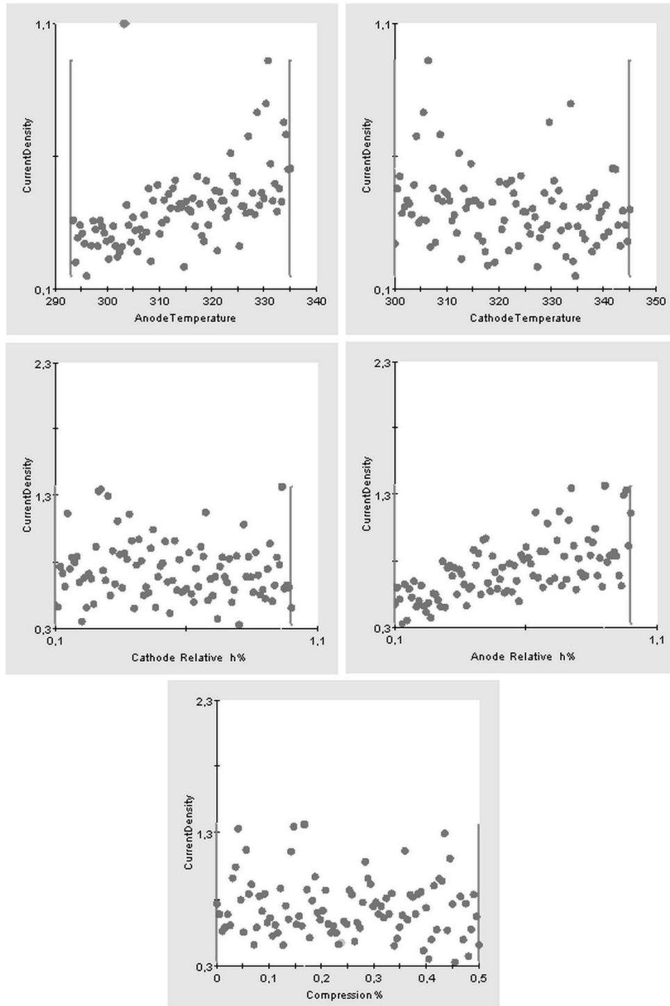
Figure 5.3 Scatter plots obtained for the sensitivity analysis of the control factors
