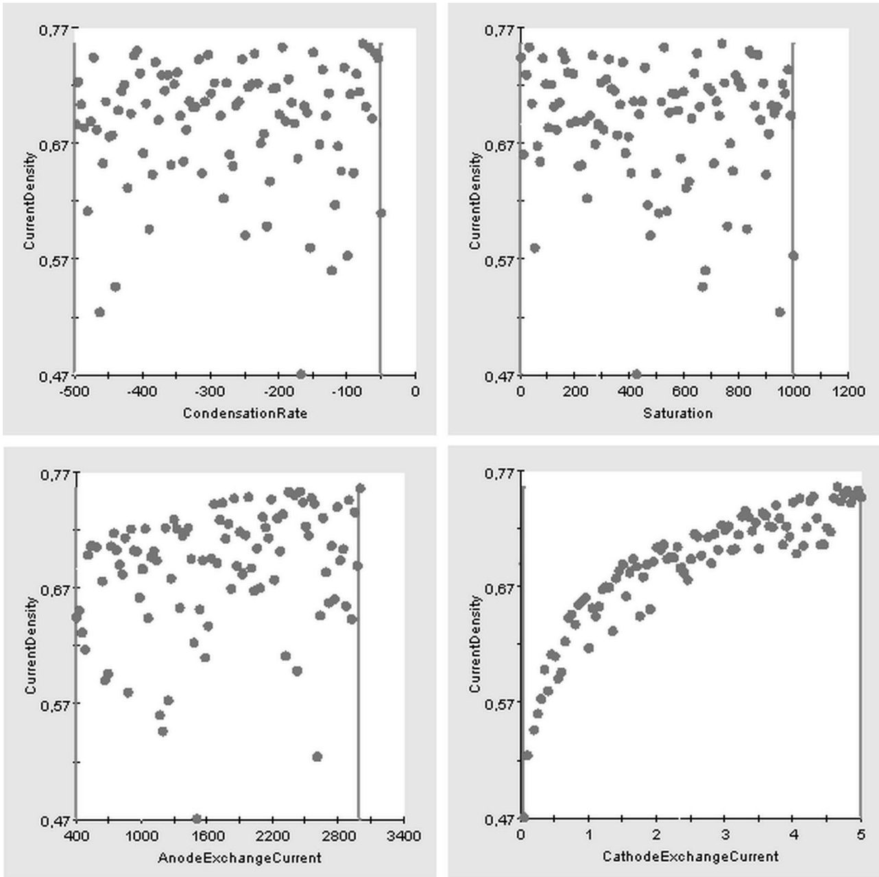
Figure 5.5 Scatter plots obtained for the sensitivity analysis of the noise factors
