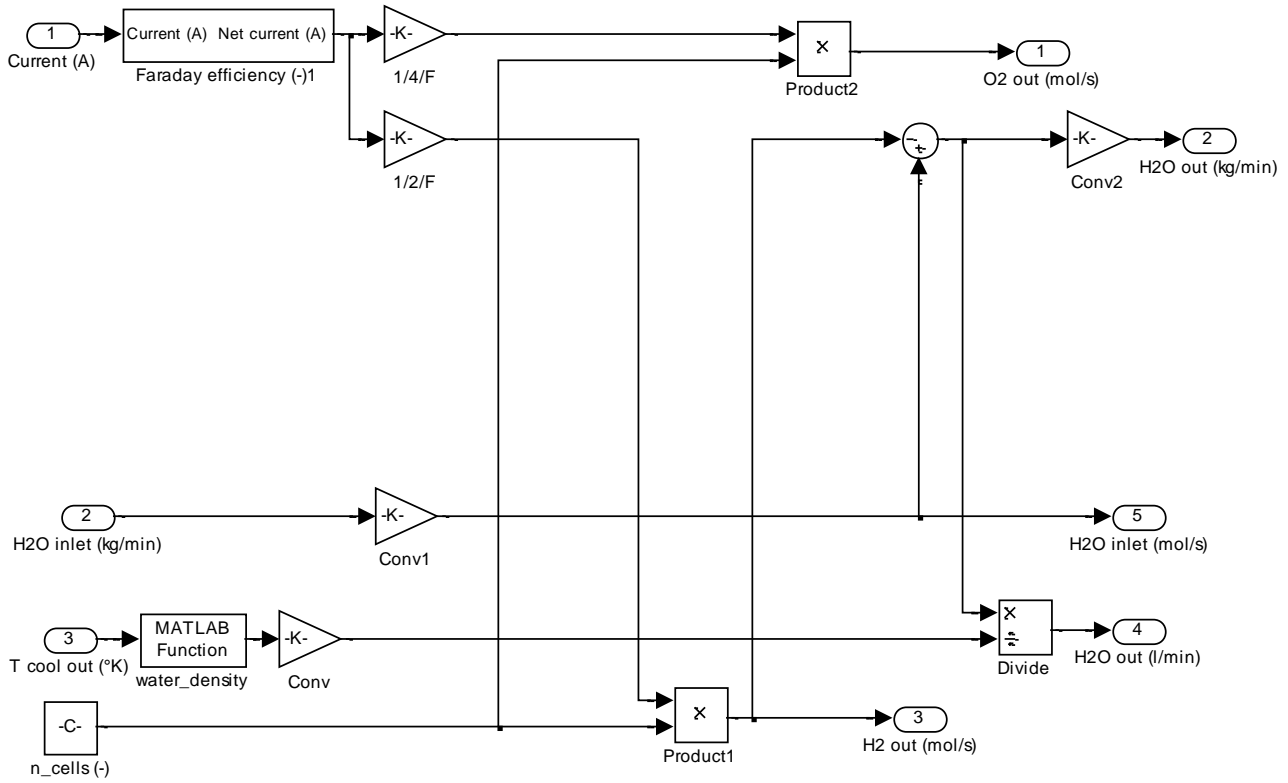
Figure 2.2 Inlet data block in Simulink
