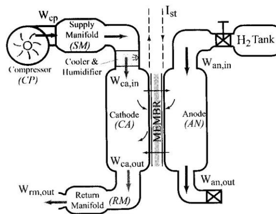
Figure 3.4 System layout modeled in Pukrushpan et al. (2004)
