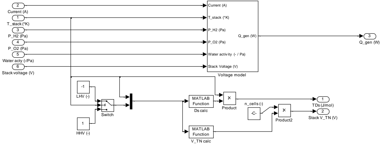
Figure 2.3 Stack voltage / efficiency model block in Simulink
