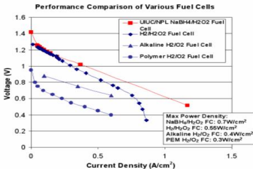
Figure 1.4 \text{H}_2\text{O}_2 fuel cell performance (Luo et al. 2008)
