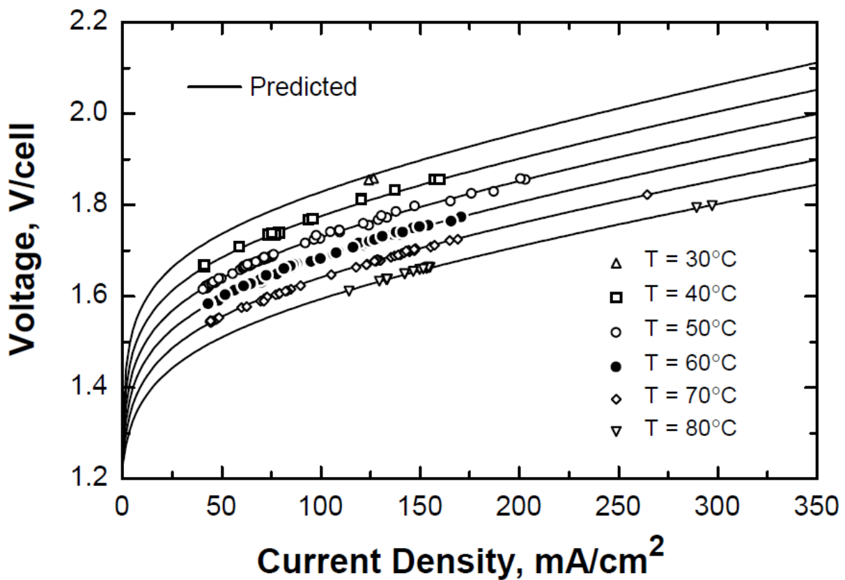
Figure 4.50 Experimental electrolyser polarization curve. Cell voltage vs. current density
