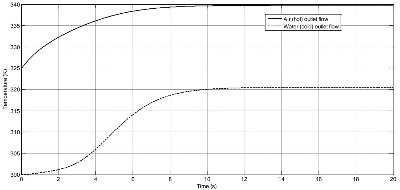
Figure 3.32 Intercooler outlet temperatures. Baseline values
