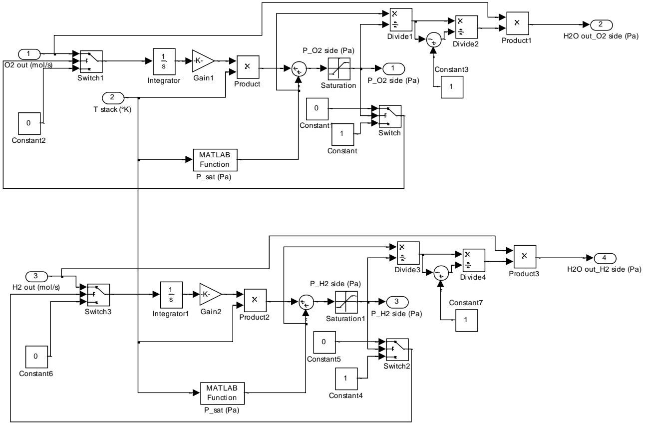
Figure 2.5 Pressure model block in Simulink
