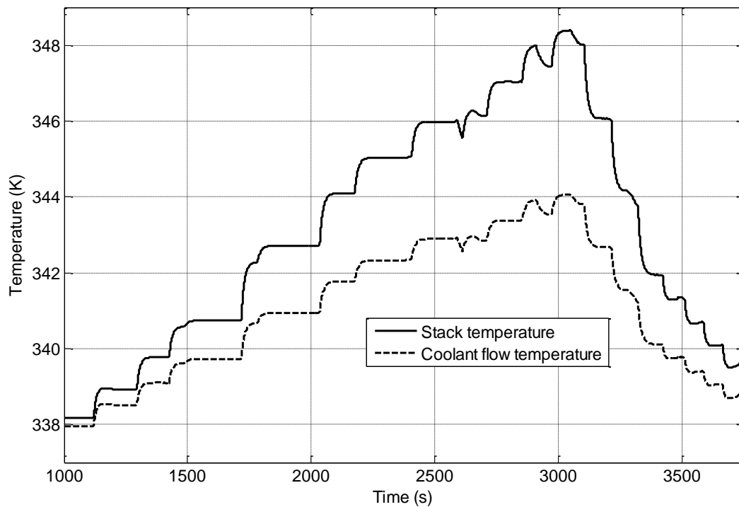
Figure 4.11 Stack and coolant flow outlet temperature vs. time
