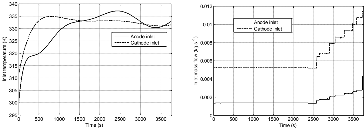
Figure 4.8 Stack inlet temperatures and mass flows for the anode and cathode sides. Anode inlet flow x 10
