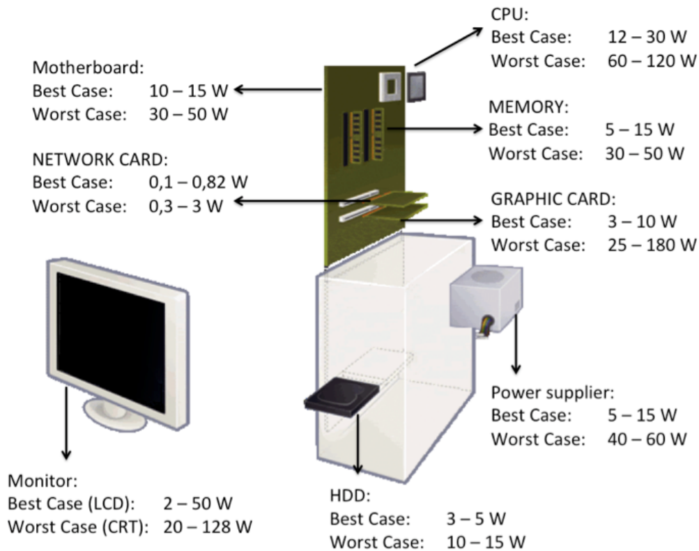
Fig. 12. Typical energy consumption of PC components based on [Moshnyaga 2009]
