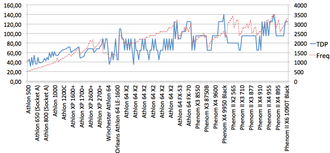
Fig. 14. CPU Frequency and TDP trend
