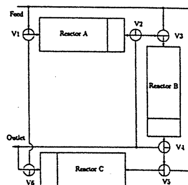
Fig. 1 - Scheme of the network of reactors.
