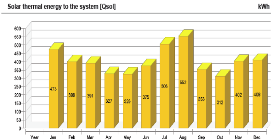
Figure 66 Solar thermal energy to the reference system for each month of year
