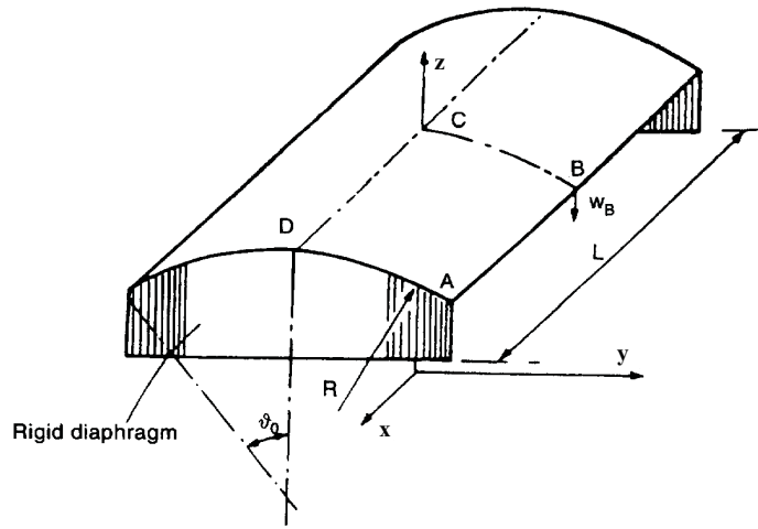
Figure 4: Scordelis-Lo roof.
