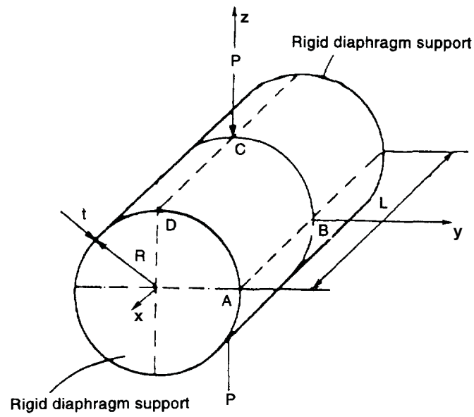
Figure 3: Pinched shell.
