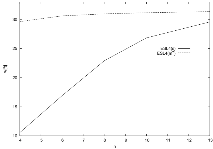
Figure 7: Scordelis-Lo problem. Thickness ratio t/R = 0.001 . Transversal displacement w [ft] at the point B of the midsurface S by varying the mesh n \times n .
