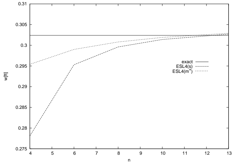
Figure 6: Scordelis-Lo problem. Thickness ratio t/R = 0.01 . Transversal displacement w [ft] at the point B of the midsurface S by varying the mesh n \times n .
