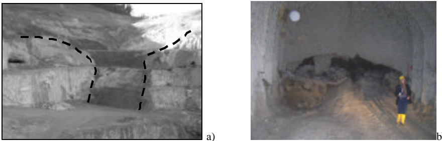
Figure 2. a) Transpressive structure observed in the Moncuoco quarry (Asti), probably related to diapirism phenomena. b) Karst void in a mining drift excavated by roadheader.
