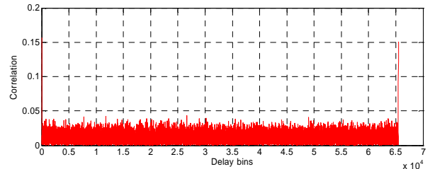
Figure 6: Curves extracted from the CAF envelope evaluated with the two steps acquisition method with bit transition.
