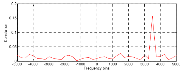
Figure 5: CAF envelope of the Galileo OS signal evaluated by the two steps method for a C/N_o of 45 dBHz with bit transition.
