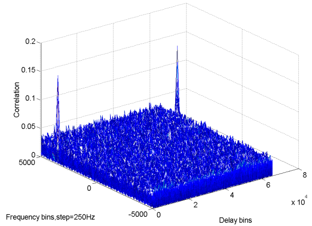
Figure 5: CAF envelope of the Galileo OS signal evaluated by the two steps method for a C/N_o of 45 dBHz with bit transition.
