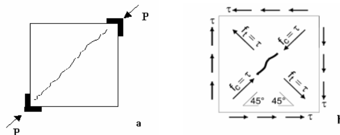
Figure 2. Loading scheme (a). Homogeneous element subjected to pure shear crack (b).
