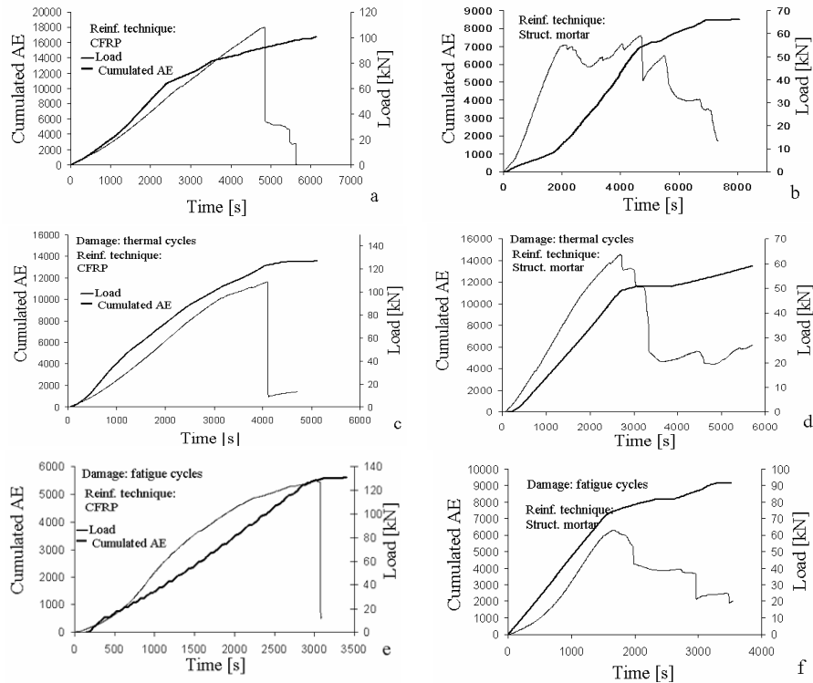
Figure 3. Load vs. time and cumulated AE number for both the reinforcement techniques: CFRP reinforcement (a). Structural mortar reinforcement (b). CFRP (c) and structural mortar reinforcement (d) after thermal cycles. CFRP (e) and structural mortar reinforcement (f) after fatigue cycles.
