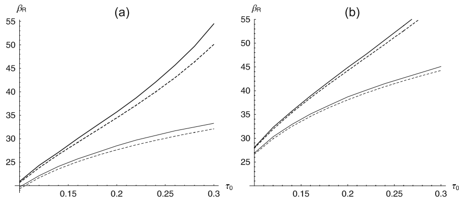
Figure 5. Behavior of \beta_R versus t_0^* for (a) d_s = 0.01 and (b) d_s = 0.001 . The bold lines refer to the ZS approach, while the thin lines refer to the JP approach (fourth-order models (solid lines) and second-order models (dotted lines)).
