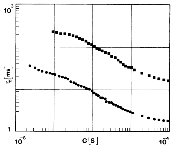
FIG. 13. The average decay time \tau_d of the photocurrent at \lambda=490 nm (●) and at \lambda=510 nm (■) versus conductance G . The curves were obtained from a set of measurements of the type reported in Fig. 11, as described in the text. Estimated errors are approximately represented by the dots' dimensions. The conductance G has been varied by changing the intensity of the background monochromatic light.
