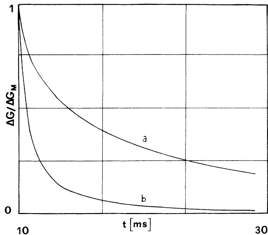
FIG. 11. Normalized phototransient decay curves obtained after a light pulse about 10^{-5} s long, superimposed to a background light source, at \lambda=510 nm (a) and at \lambda=490 nm (b). The curves are not simple exponential functions and are interpreted as a superposition of exponential decays related to the different lifetimes of the ionized centers or trapped holes (according to the \lambda value) which control the barrier height. The average conductance G is the same for the two curves and corresponds to 10^{-6} S.
