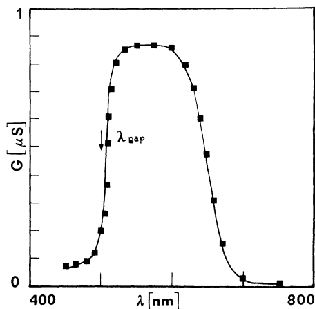
FIG. 9. The electrical conductance G versus light wavelength \lambda at a fixed value of photon flux n_f ( n_f \approx 10^{11} photons s^{-1} ). According to the barrier model, the rapid increase of the conductance with \lambda in correspondence of \lambda_{\text{gap}} is mostly related to a corresponding rapid increase of the lifetime of the positive trapped charge (see Fig. 13) which controls the barrier height (trapped holes for \lambda < \lambda_{\text{gap}} , deep donor centers for \lambda > \lambda_{\text{gap}} ).
