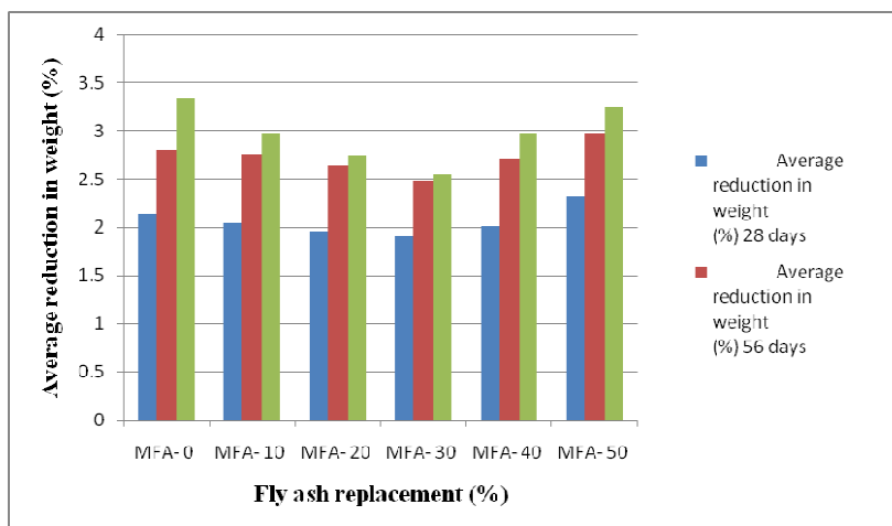
Figure 8: Sulphate Attack
