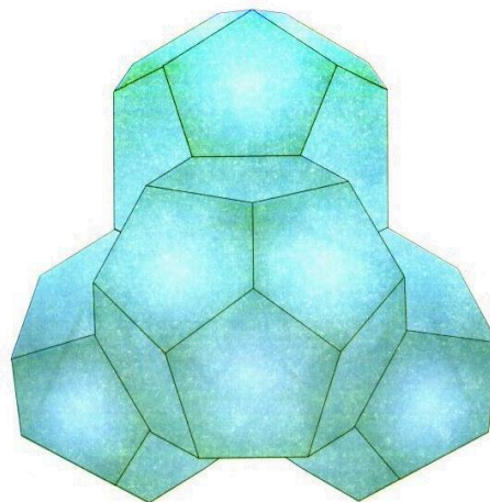
Figure 12. Model of water associate from 57 \text{H}_2\text{O} molecules. Tetrahedron of four dodecahedron
