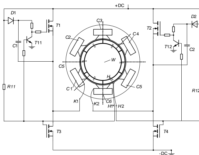
Fig. 1. Schematic diagram of control circuit of PM BLDC single coil motor.
