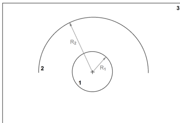
Fig. 7. View factors of a tube – half-tube setup.
