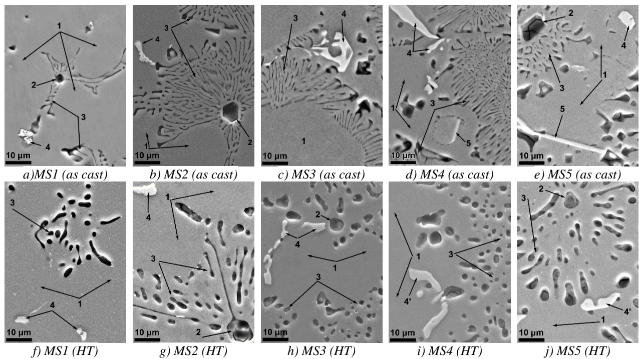
Fig. 1. Microstructure of Al-7Mg-XSi-0,6Mn alloys: a) - e) as cast, f) - j) after heat treatment.
