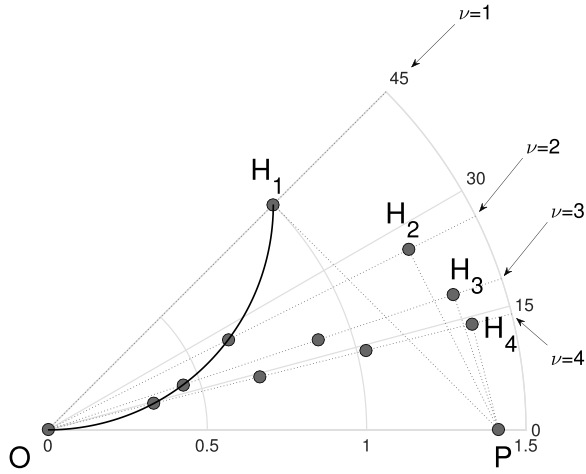
Fig. 3. Stencil of graphs G(\nu = \{1, 4\}; \Delta x = \overline{OP}/\sqrt{1+\nu^2}) of constant path resolution \Delta P = \overline{OP} . For a given \nu , the gridpoints are aligned along the angle \Delta\theta defined by (5) and their spacing \Delta x/\overline{OH}_1 as a function of \Delta\theta is the solid line per O and H_1 . Angles \overline{OH}_\nu P = 90^\circ \forall \nu correspond upon axes tilting to \overline{OH}_\nu P_\nu of Fig. 2.
