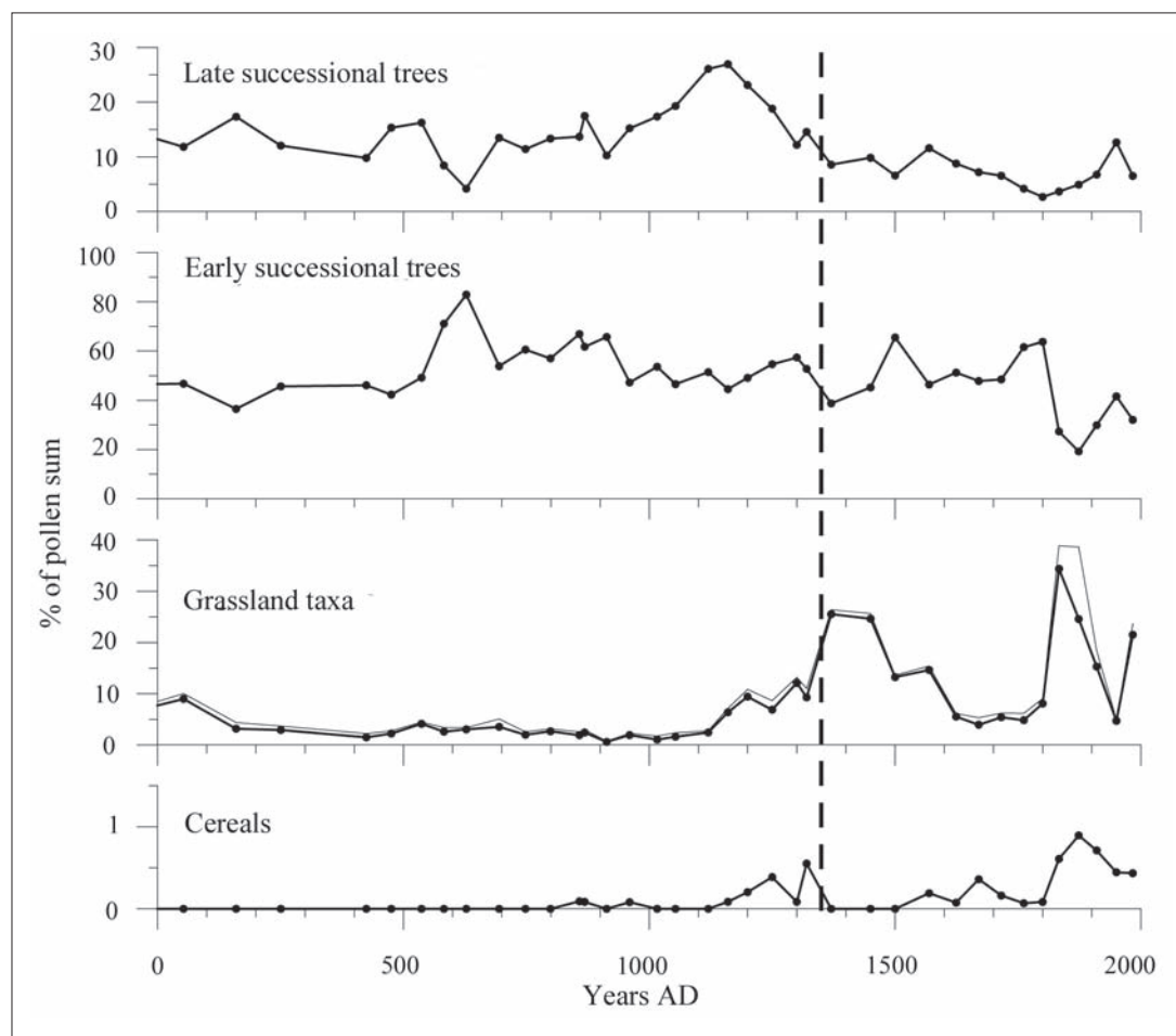
Fig. 7. Pollen graphs from the Värnsjö Utmark site. For an explanation, see captions to Figs. 2 and 6 (based on pollen data from Lagerås 2007).
