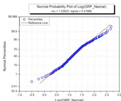
Figure 1B. Normal probability plot of logarithmic values of GRPs in Croatia
