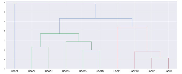
Fig. 16: Hierarchical clustering of user sequences.
