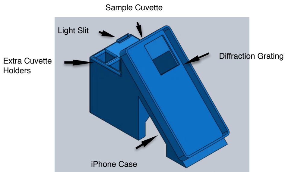
Figure 3: Assembly of the spectrophotometer. There are positions for an adjustable light slit, cuvette sample holder, two extra cuvette holders, a diffraction grating, and iPhone case aperture. The drawing and image was created using SolidWorks version 64, 2014.
