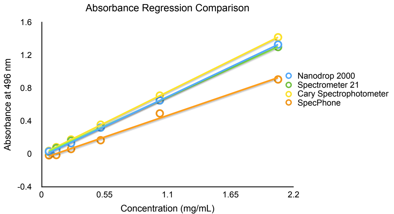
Chart 1: Linear Regressions of Commercial Spectrophotometers and the Cell Phone Spectrophotometer for an Absorbance at 496 nm versus Concentration of Cherry Kool-aid Solutions
