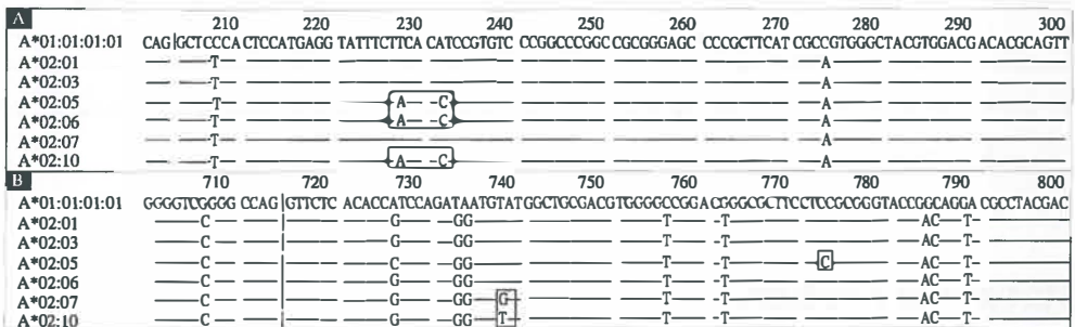
Figure 1 Alignment of the HLA-A*02 gene fragments that are amplified and sequenced to discriminate between common and well defined HLA-A*02 allele. The four SNPs that are able to discriminate between the major HLA-A*02 subtypes (IMGT/HLA database, http://www.ebi.ac.uk/imgt/hla/ ) are indicated by boxes. (A) Two SNPs located at position 228 and 231 are specific for HLA-A*02:05, A*02:06 and A*02:10. (B) Another SNP located at position 773 is specific for HLA-A*02:05 only and one SNP at position 739 can differentiate both HLA-A*02:07 and A*02:10 from others. Numbers above the sequences indicate nucleotide positions. Nucleotide sequences were aligned to the HLA-A*01:01 allele. Dashes indicate identity with the reference sequence. The intron1-exon 2 (A) and exon2-exon3 (B) junctions are denoted by vertical bars.
