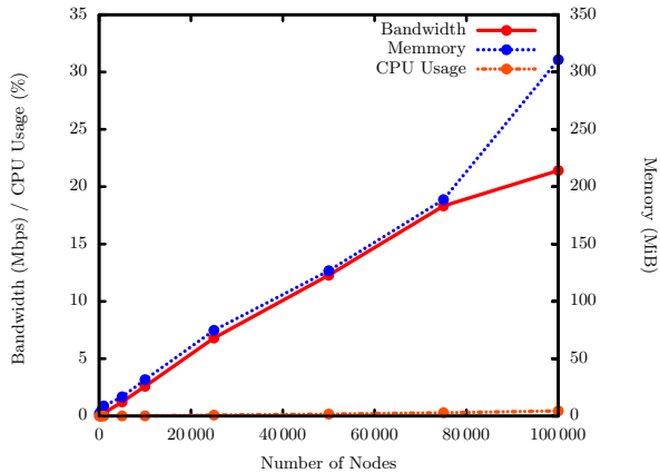
Figure 10: The resources required of Panopticon’s top aggregation node — they are well within the limits of current hardware.
