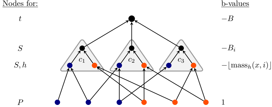
■ Figure 1 Example for the graph G used in the rounding of the x -variables. B_i = \lfloor \text{mass}(x, i) \rfloor - \sum_{h \in \text{Col}} \lfloor \text{mass}_h(x, i) \rfloor and B = |P| - \sum_{i \in S} \lfloor \text{mass}(x, i) \rfloor .
