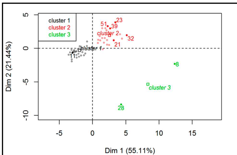
Figure 5. Hierarchical classification of the samples (red and white wines; n = 52 ).
