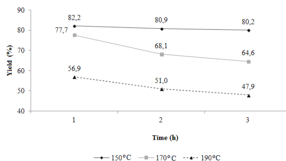
FIGURE 1: Organosolv bamboo pulping process yield at temperatures of 150, 170 e 190°C, for 1, 2 and 3 h.
