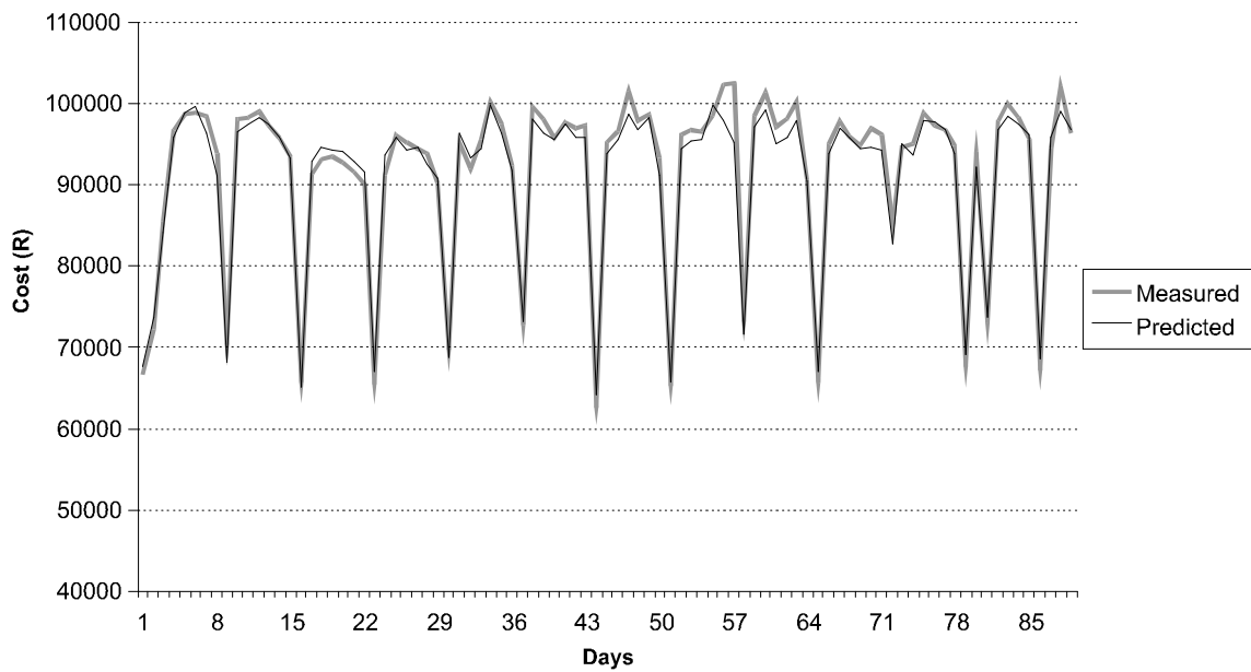
Figure 5: Load prediction model verification at Kopanang
