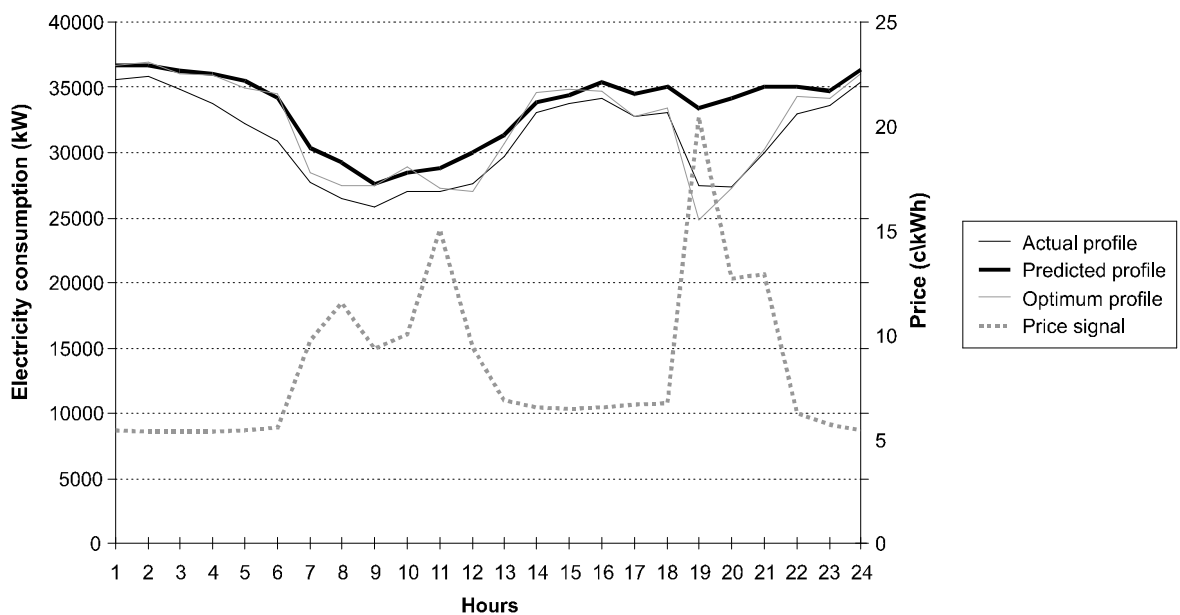
Figure 6: Average weekday demand profiles during September 2001 at Kopanang
