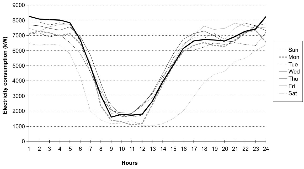
Figure 3: Summer pumping CBL's for Kopanang
