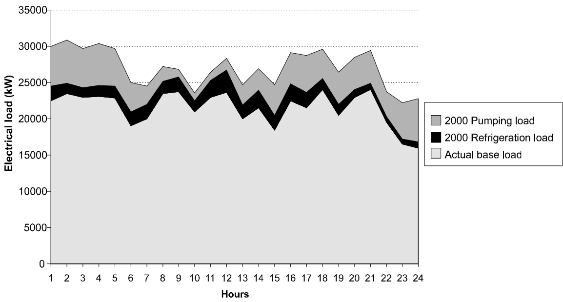
Figure 4: The composition of the predicted total load profile at Kopanang
