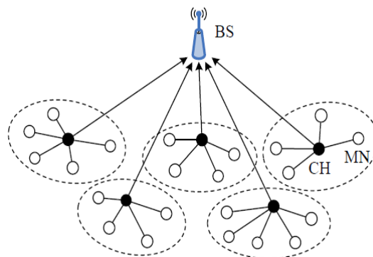
Figure 6. Basic Topology of LEACH
