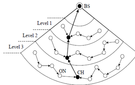
Figure 9. Data Transmission scheme in PEGASIS
