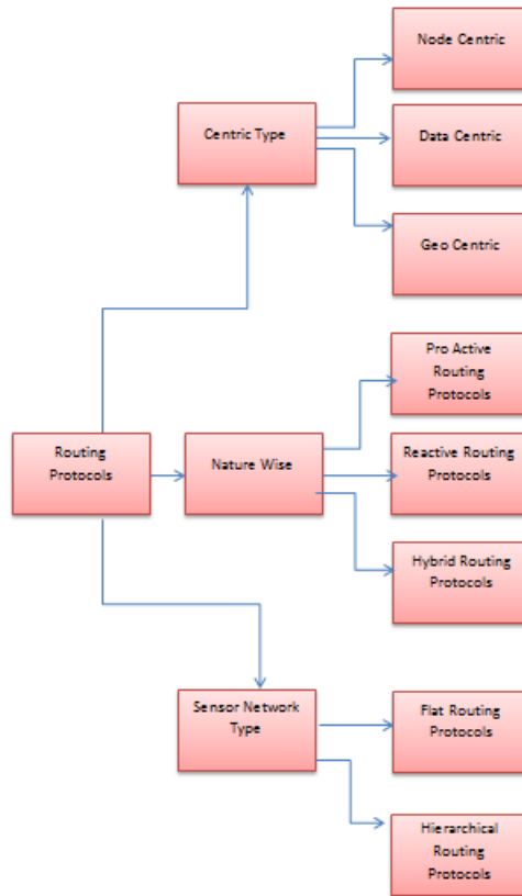
Figure 2. Classification of Routing Protocol
