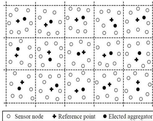
Figure 7. Illustration of Geographical clustering in PANEL
