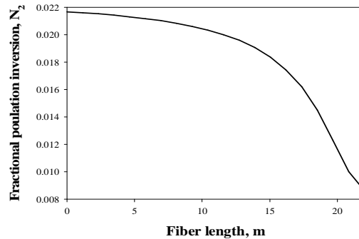
Fig. 6. Evolution of population inversion along the fiber length.
