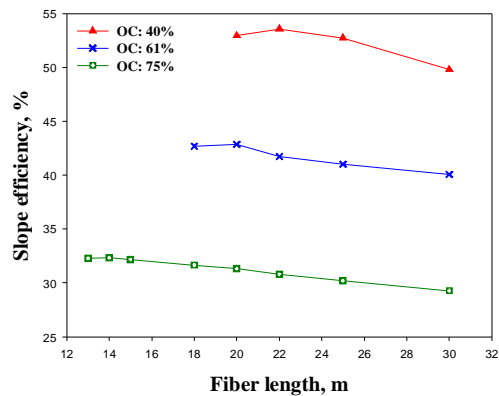
Fig. 5. Slope efficiency vs. active fiber length for different output coupler reflectivity.
