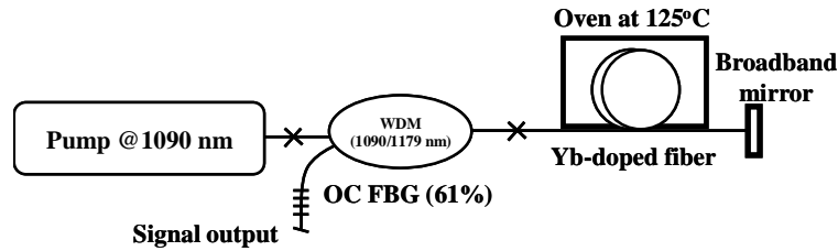
Fig. 1. Experimental setup of the 1179 nm fiber laser.
