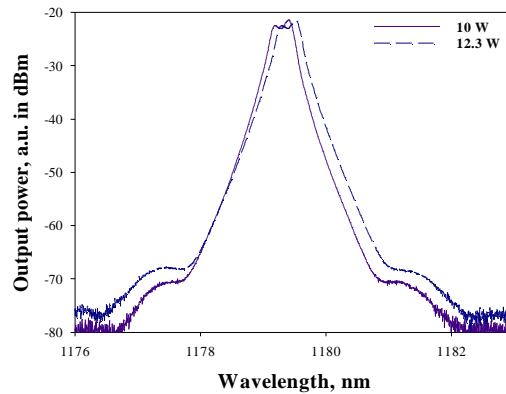
Fig. 3. Output spectrum of the fiber laser at different signal power (optical spectrum analyzer resolution 0.02 nm).
