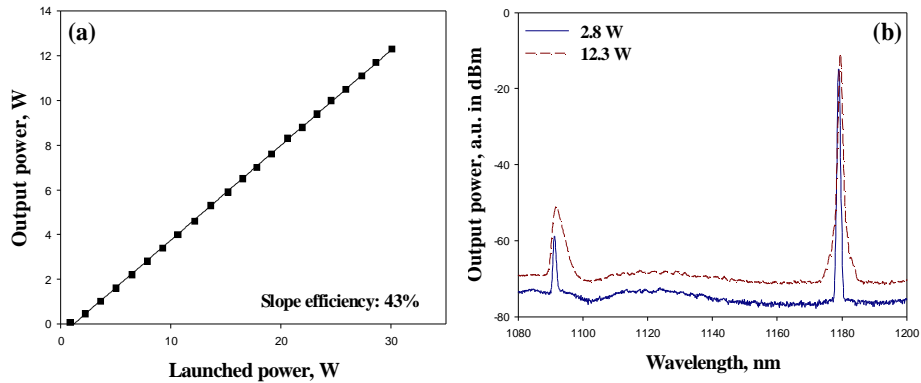
Fig. 2. (a). Output power and (b) output spectrum (taken with an optical spectrum analyzer with 0.5 nm resolution) of Yb-doped fiber laser operating at 1179 nm.
