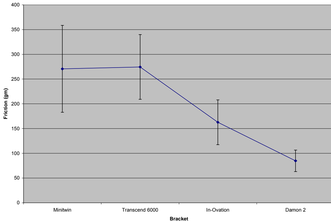
Figure 21. The static, kinetic and dynamic friction with the standard deviation of the 6 archwires were averaged to obtain the friction for each bracket.
