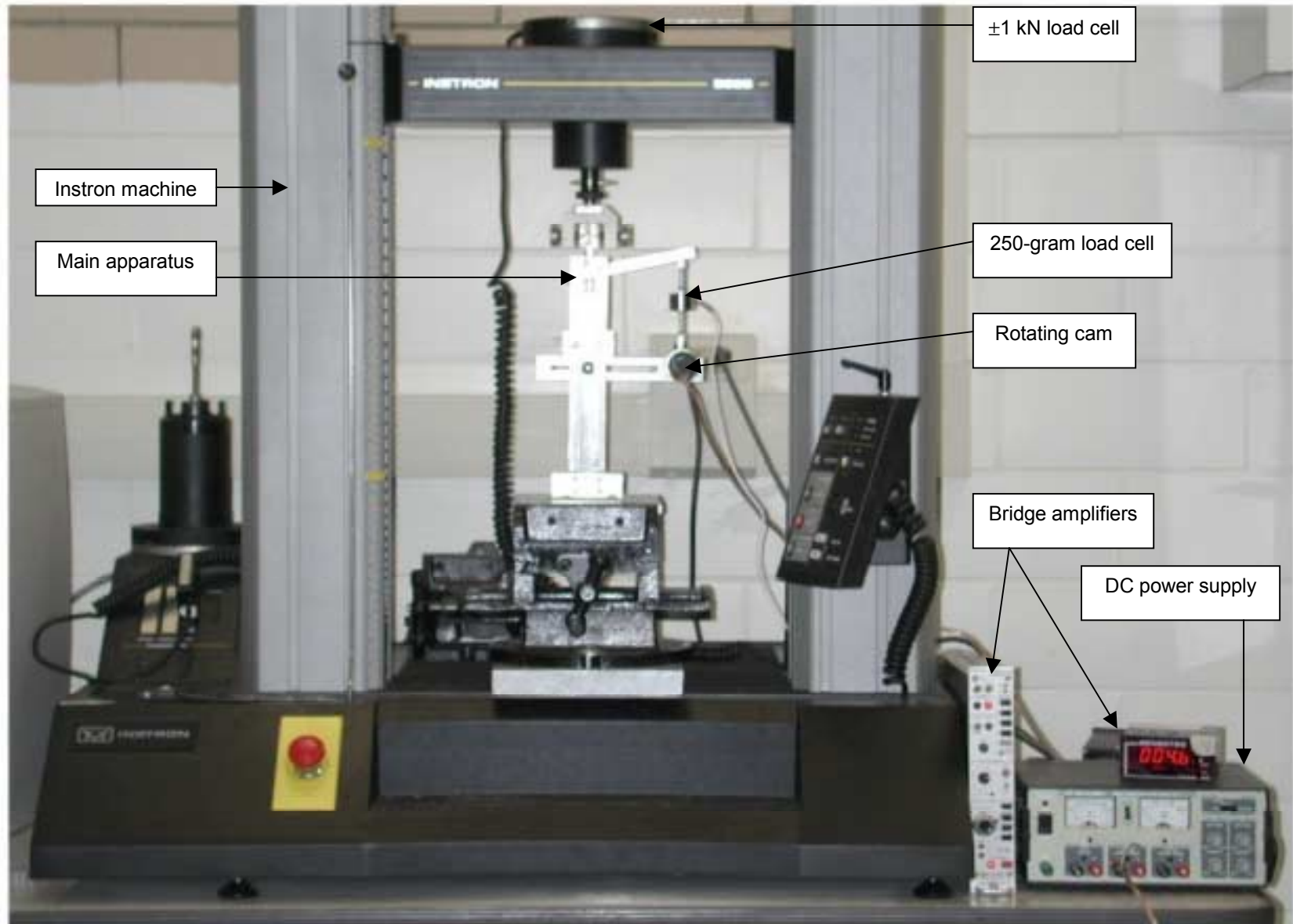
Figure 2. Friction-testing apparatus.
