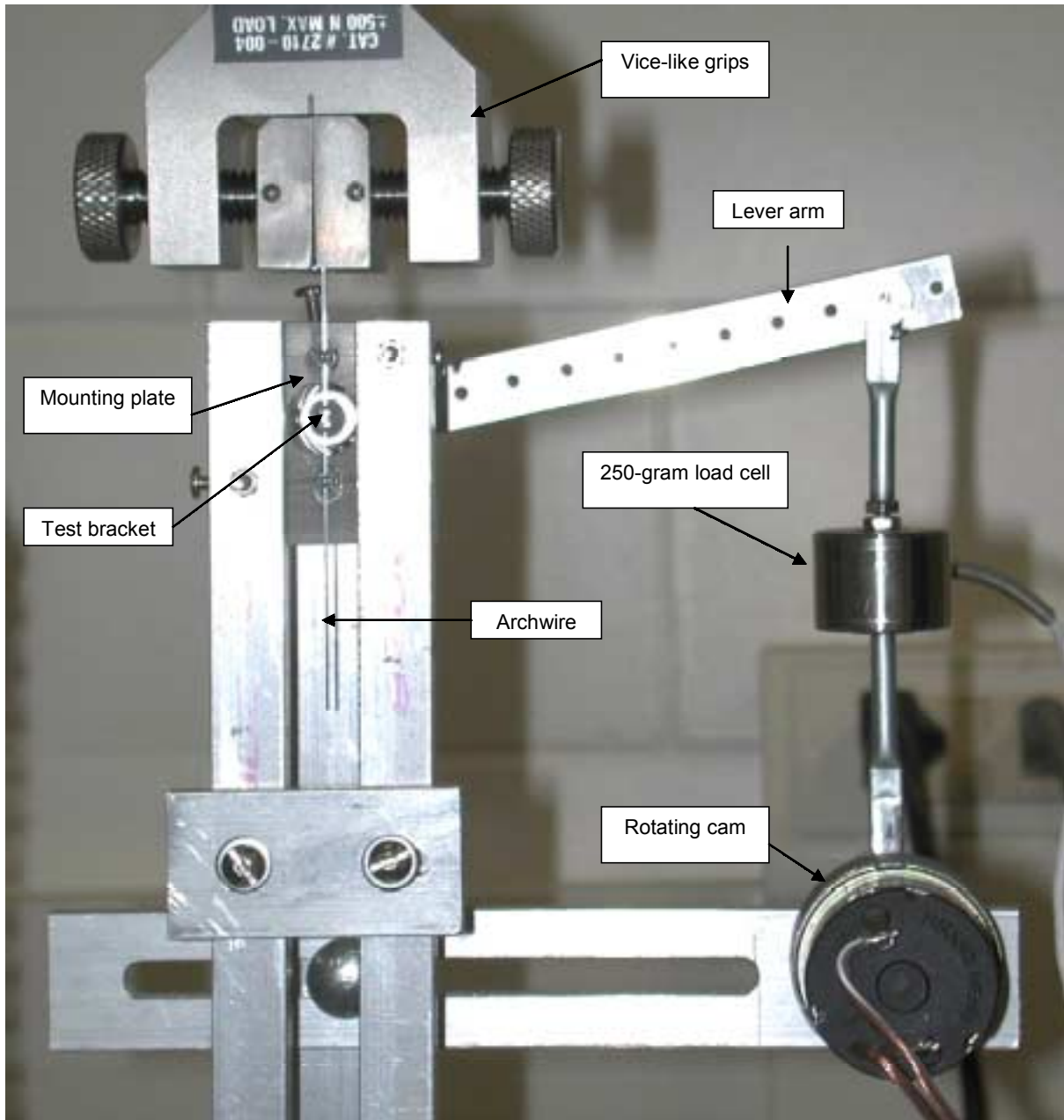
Figure 9. Photograph showing main part of the apparatus consisting of vice-like grips, mounting plate, test bracket, archwire, lever arm, 250-gram load cell and rotating cam.
