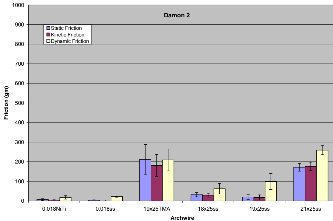
Figure 18. Bar graph with the standard deviation of friction type for the Damon 2 bracket grouped by archwires.
