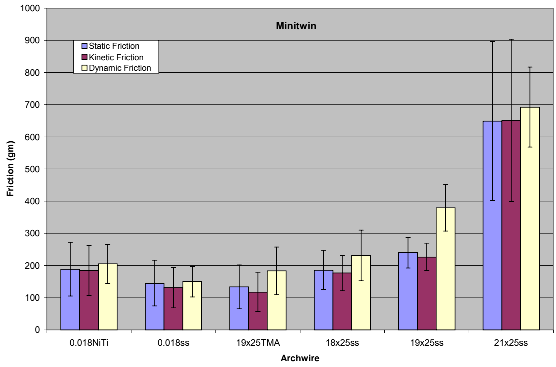
Figure 15. Bar graph with the standard deviation of friction type for the Minitwin bracket grouped by archwires.
