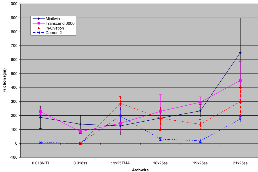
Figure 23. Static and kinetic friction averaged with the standard deviation for each bracket-archwire combination.
