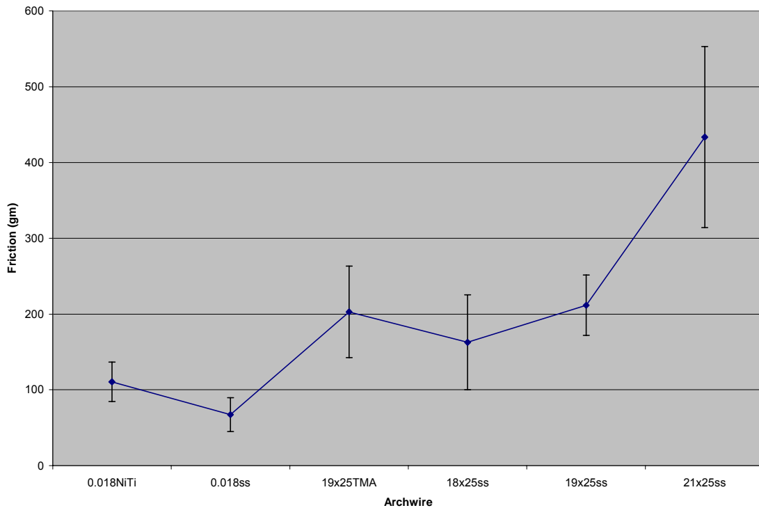
Figure 19. The static, kinetic and dynamic friction with the standard deviation of the 4 brackets were averaged to obtain the friction for each archwire.
