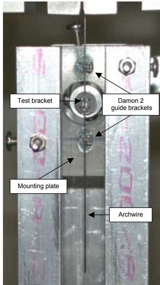
Figure 10. Close-up view of archwire alignment through Damon 2 brackets, on mounting plate, and test bracket.
