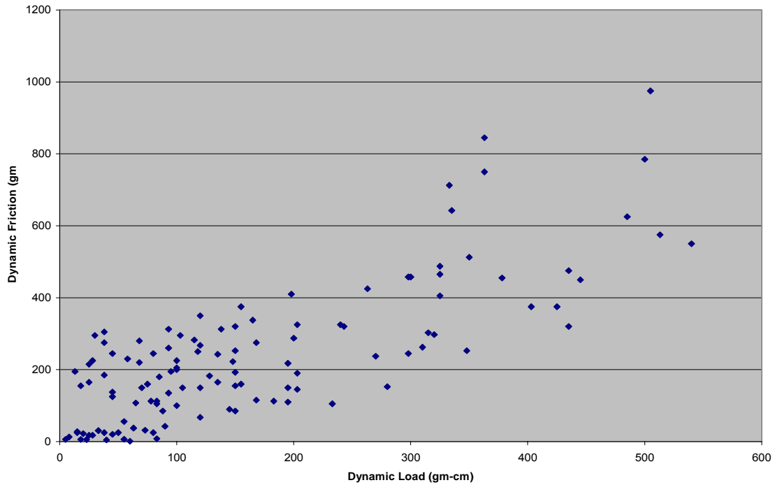
Figure 25. Dynamic load is proportional to dynamic friction.
