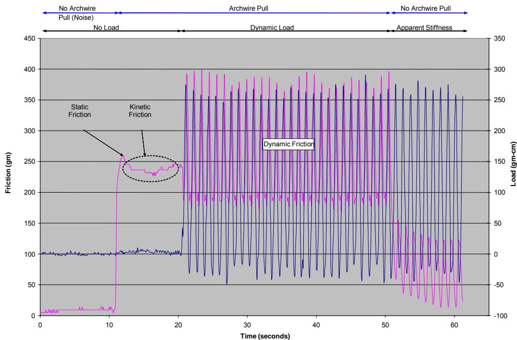
Figure 13. Sample graph of raw data with labels.
