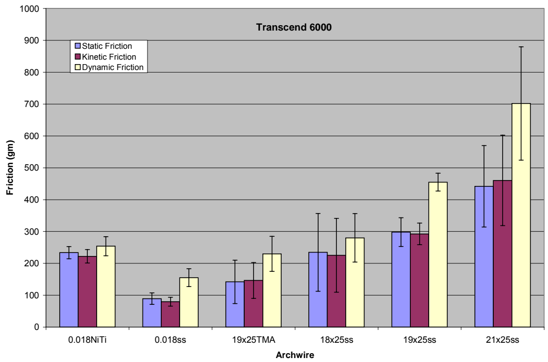
Figure 16. Bar graph with the standard deviation of friction type for the Transcend 6000 bracket grouped by archwires.
