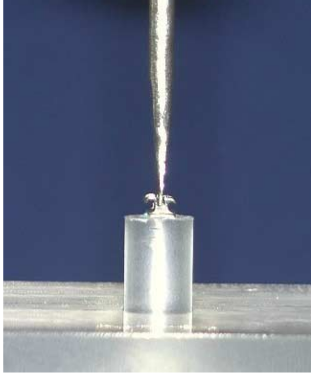
Figure 8. Close-up view of surveyor pin aligning test bracket mounted on acrylic rod.
