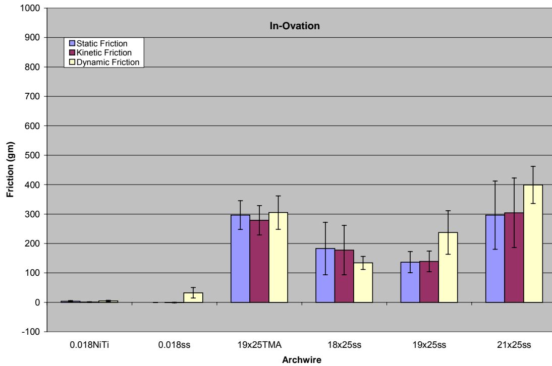
Figure 17. Bar graph with the standard deviation of friction type for the In-Ovation bracket grouped by archwires.
