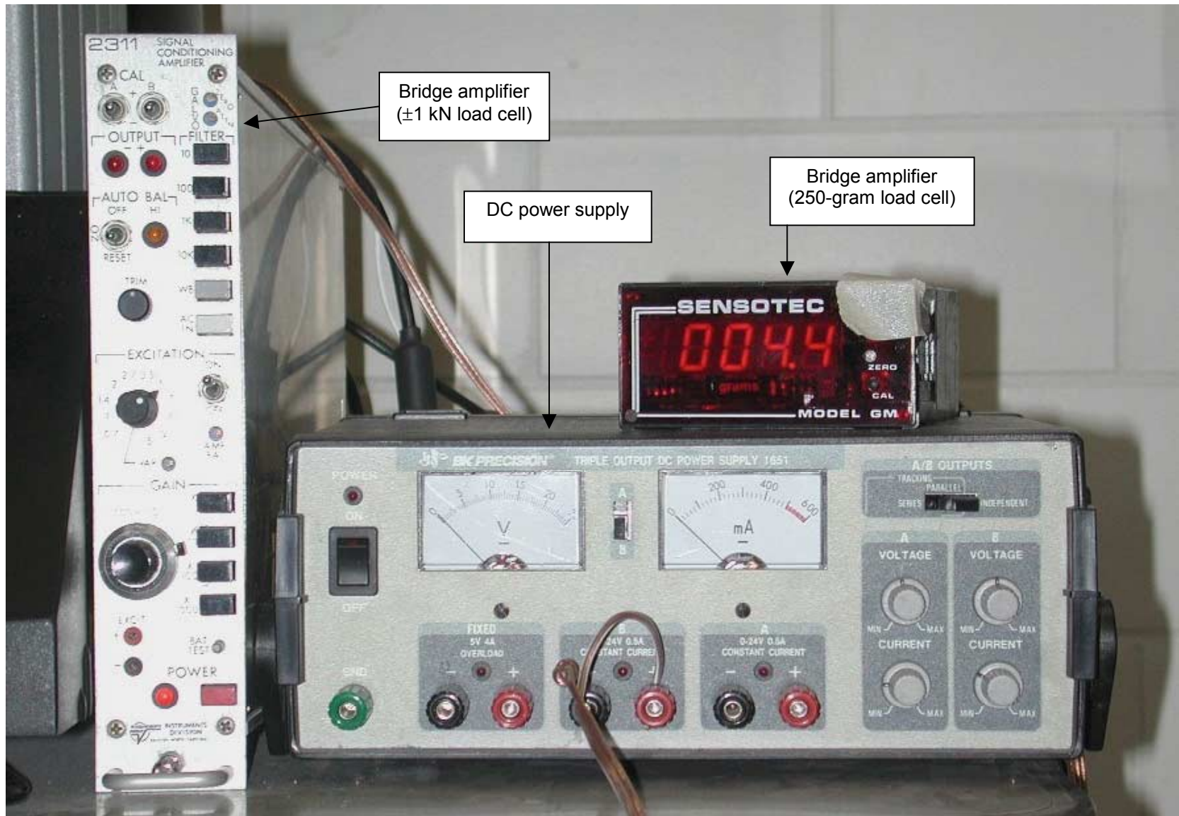
Figure 11. DC power supply and two bridge amplifiers.
