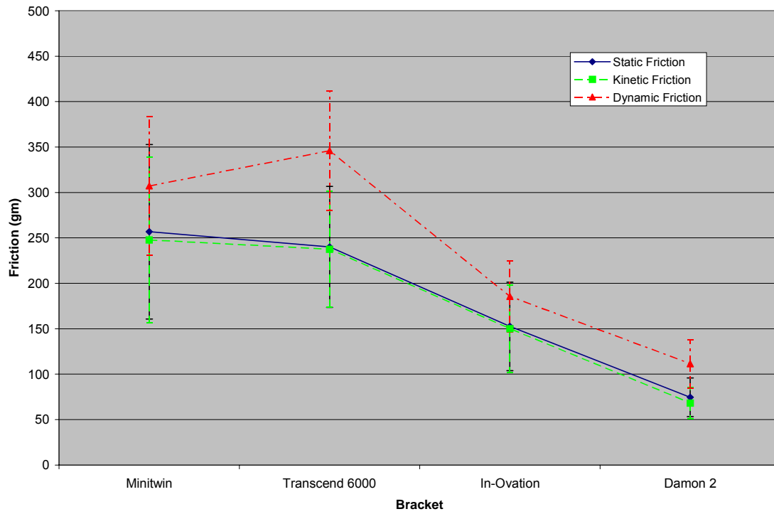
Figure 14. An average of the static, kinetic and dynamic friction with the standard deviation of all wires for each bracket was calculated. The line graph shows the similarity between static friction and kinetic friction, while dynamic friction was statistically significant.
