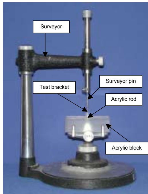
Figure 7. Dental surveyor with acrylic block and acrylic rod utilized to mount test brackets.
