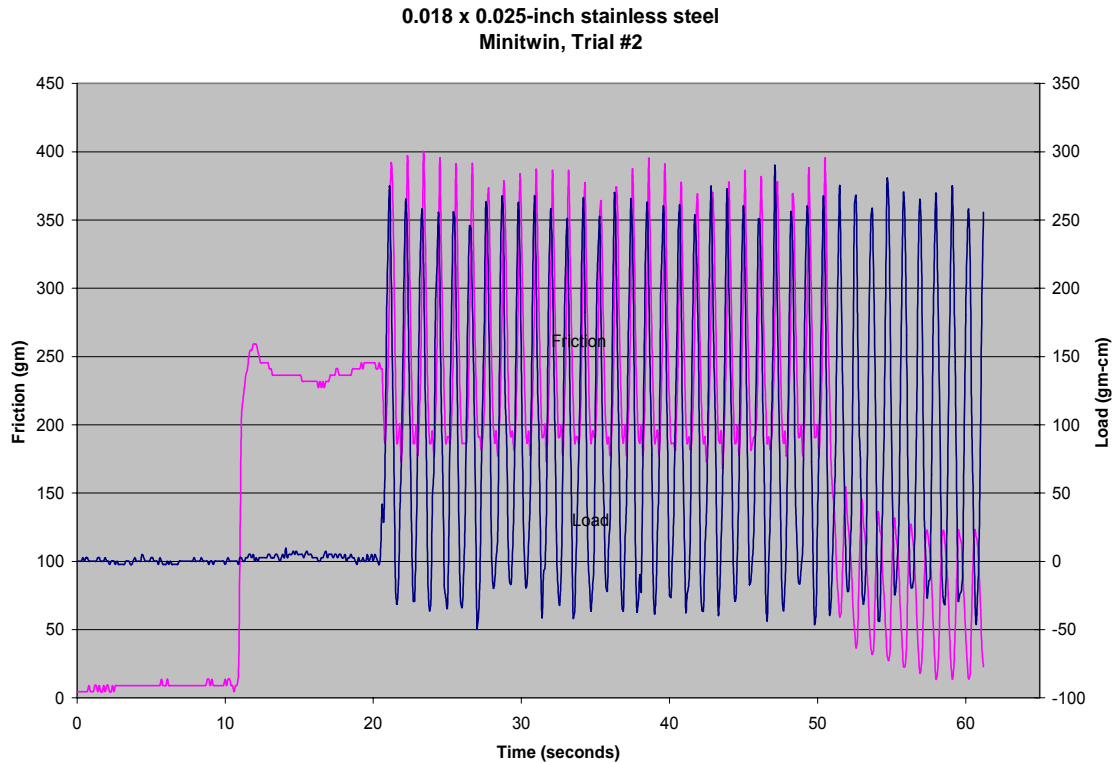
Figure 12. Sample graph of raw data.
