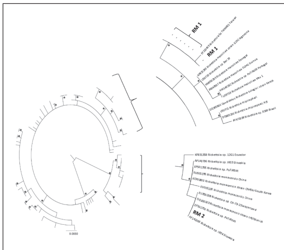
Figure 3 Maximum likelihood phylogenetic analysis of Rickettsia partial gltA gene sequences (second dataset). Branch lengths were estimated with the best fitting nucleotide substitution model according to a hierarchical likelihood ratio test and were drawn in scale with the bar at the bottom indicating 0.0050 nucleotide substitutions per site. The * along the branch represents significant statistical support for the clade subtending that branch (bootstrap support > 75%). The tree is midpoint rooted. The Italian isolates (collected in Rome) are shown in bold. The figure is also available online as supplementary material in an enlarged version.
