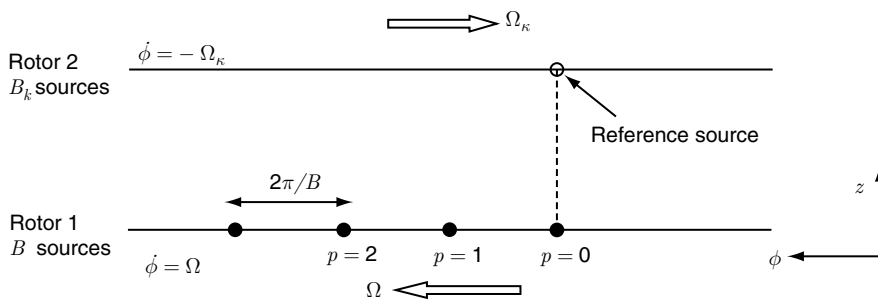
Figure 4: Illustration showing set-up for modelling rotor-rotor interaction tones.
