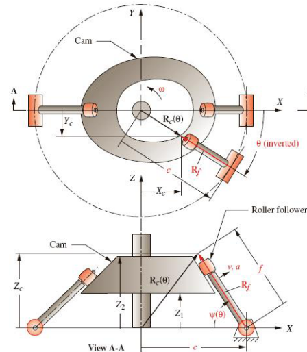
Figure 5. Globoidal Cam (Norton, 2008).
