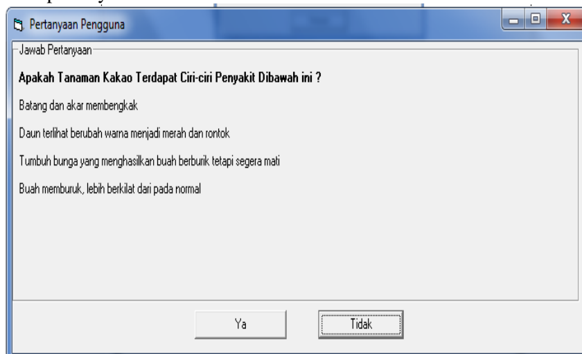
Gambar 8 Form Pertanyaan
