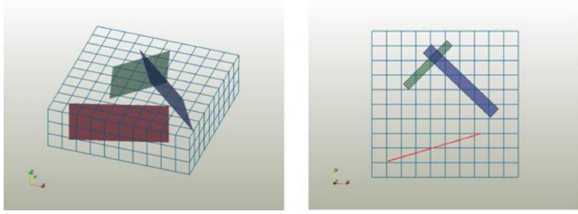
Fig. 3. Schematic representation of reservoir model using EDFM: oblique view (left), and top view (right) (Shakiba and Sepehrnoori, 2015).
