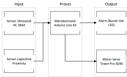
Gambar 1 Blok Diagram
