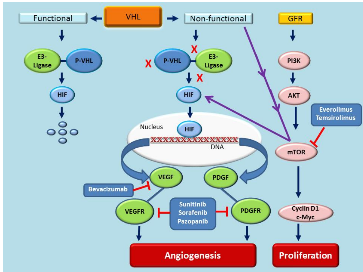
Figure 1. The role of VHL and mTOR in angiogenesis and proliferation of RCC. A non-functional VHL is the major risk factor for the development and progression of RCC. The functional protein of VHL, pVHL, complexes with E3-ligase and degrades HIF. When the VHL is non-functional, HIF is stabilized and translocated to nucleus where it binds with HIF responsive elements of the DNA and activates many pro-angiogenic factors including VEGF and PDGF. They interact with their respective tyrosine kinase receptors VEGFR (mostly at endothelial cells) and PDGFR (mostly at vascular smooth muscle cells and pericytes) and promote angiogenesis. The PI3K/AKT/mTOR pathway is activated by many factors including growth factor receptors. mTOR in turn activates cyclin D1 and cMyc and promotes cell proliferation and survival. Furthermore, VHL inactivation also activates mTOR, which in turn up-regulates HIF and subsequent angiogenesis. GFR, growth factor receptor; HIF, hypoxia-inducible factor; PDGF platelet-derived growth factor; PDGFR, receptor for PDGF; VEGF, vascular endothelial growth factor; VEGFR, receptor for VEGF; VHL, von Hippel Lindau gene.
