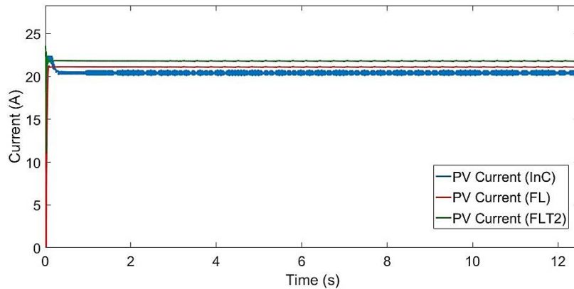
Fig. 14 The PV Current with InC, FL, and FLT2 MPPT algorithms
