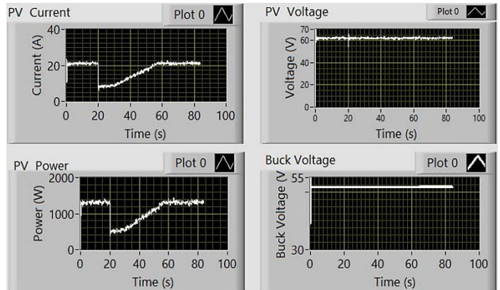
Fig. 28 Experimental results of FLT2 MPPT Algorithm at variable irradiation
