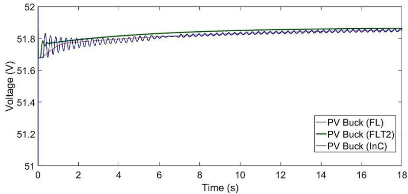
Fig. 16 The Output Voltage of Buck Converter with InC, FL, and FLT2 MPPT algorithms
