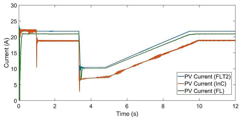
Fig. 18 The PV Current with InC, FL, and FLT2 MPPT algorithms
