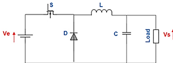
Fig. 3 DC/DC Buck Converter
