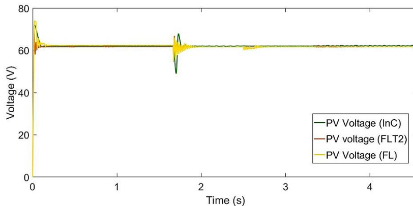
Fig. 17 The PV Voltage with InC, FL, and FLT2 MPPT algorithms
