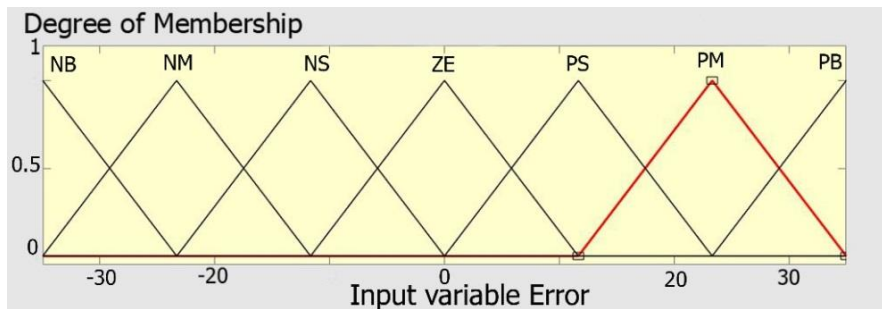
Fig. 4 The input of Fuzzy Logic Controller (Error)
