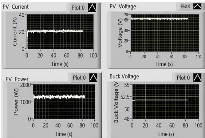
Fig. 24 Experimental results of FL MPPT Algorithm at stable climatic conditions
