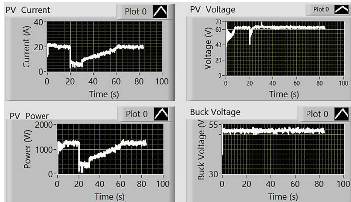
Fig. 26 Experimental results of InC MPPT Algorithm at variable irradiation
