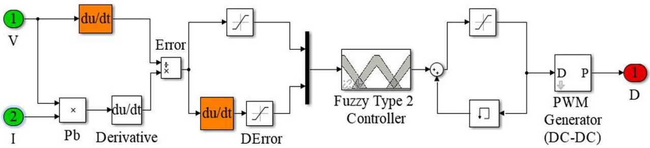
Fig. 12 FLT2 algorithm in Matlab/Simulink
