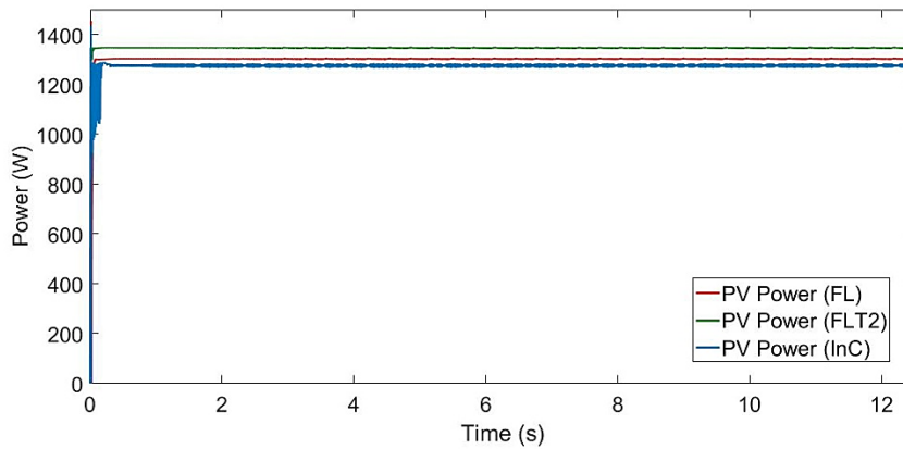
Fig. 15 The PV Power with InC, FL, and FLT2 MPPT algorithms
