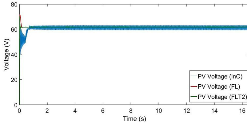
Fig. 13 The PV Voltage with InC, FL, and FLT2 MPPT algorithms
