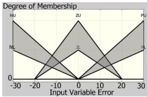
Fig. 8 Membership function for Error
