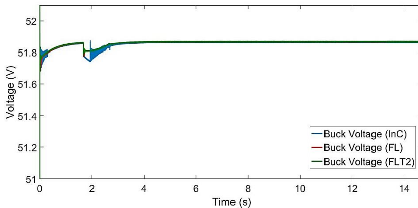
Fig. 20 The output voltage of buck converter with InC, FL, and FLT2 MPPT algorithms
