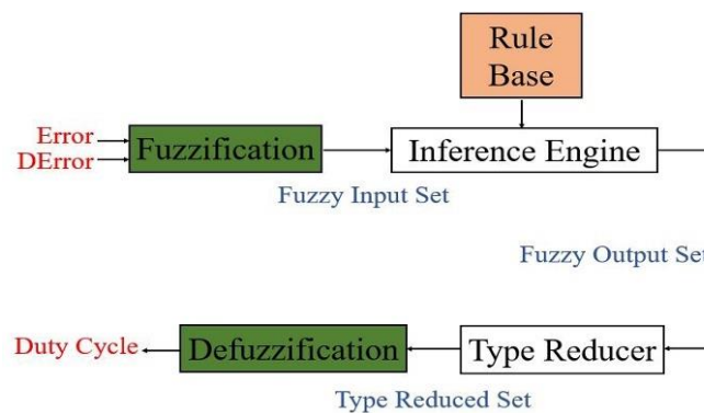
Fig. 7 The Fuzzy Logic Type 2 Controller diagram
