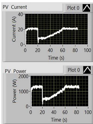
Fig. 27 Experimental results of FL MPPT Algorithm at variable irradiation
