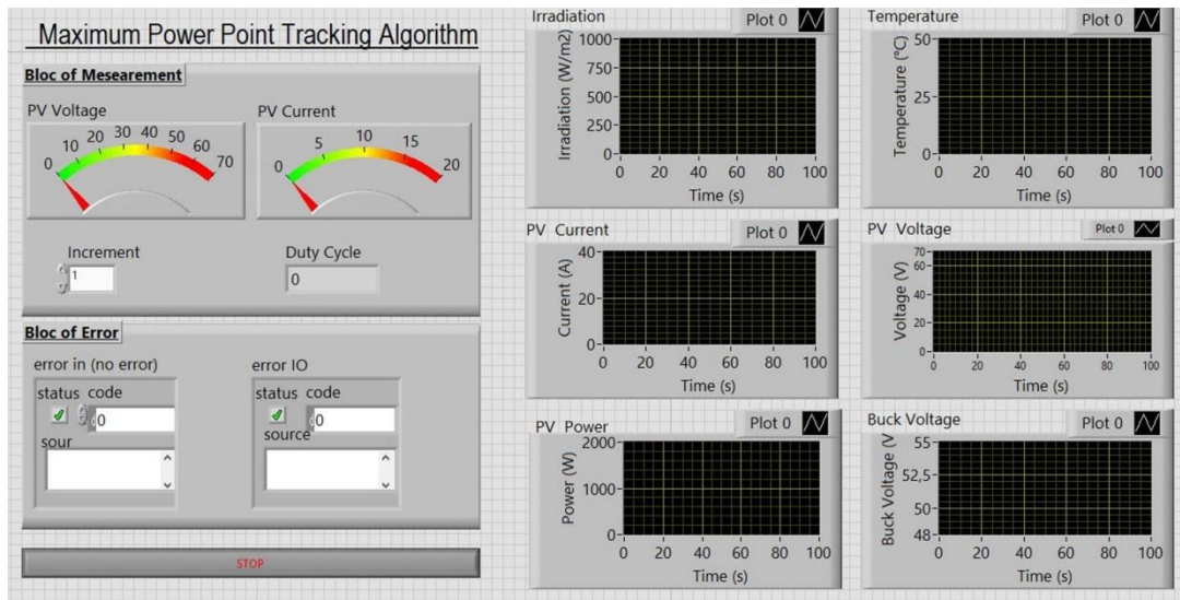
Fig. 22 LabVIEW Front Panel of the MPPT Algorithms
