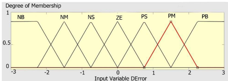
Fig. 5 The input of Fuzzy Logic Controller (DError)
