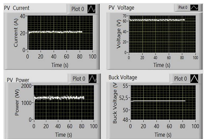
Fig. 25 Experimental results of FLT2 MPPT Algorithms at stable climatic conditions
