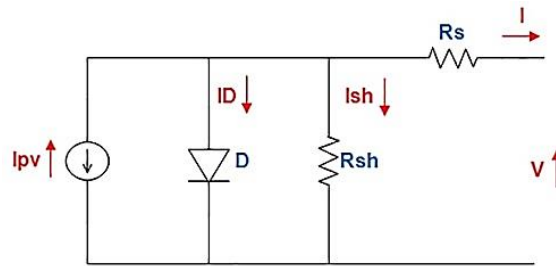
Fig. 1 Electric circuit of PV cell
