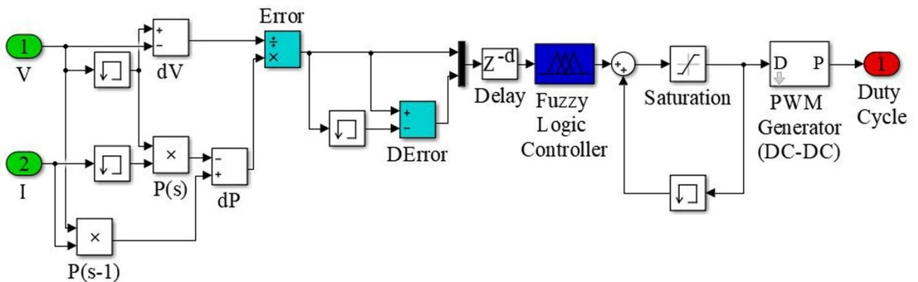
Fig. 11 FL algorithm in Matlab/Simulink
