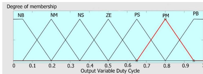
Fig. 6 The output of Fuzzy Logic Controller (Duty Cycle)
