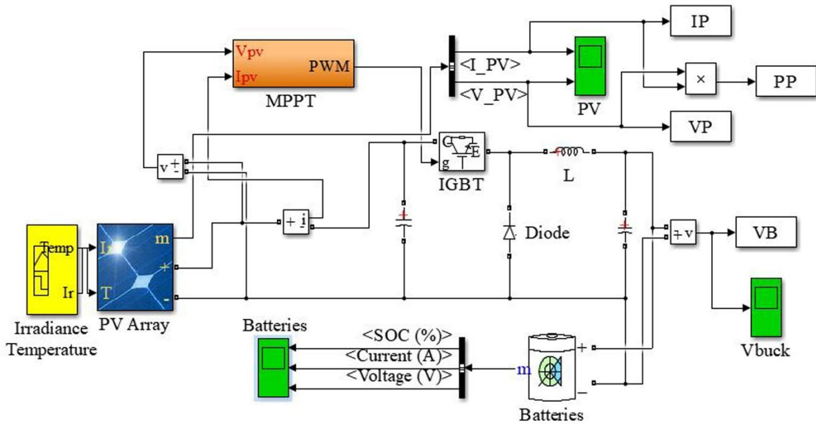
Fig. 10 The global system in Matlab/Simulink
