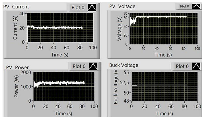
Fig. 23 Experimental results of InC MPPT Algorithm at stable climatic conditions
