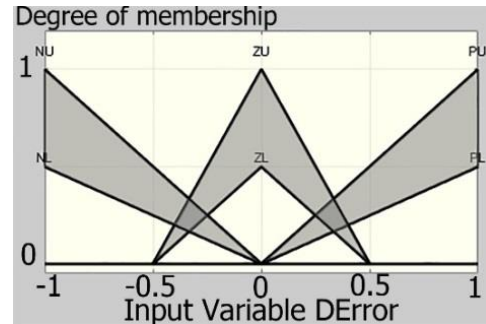
Fig. 9 Membership function for DError
