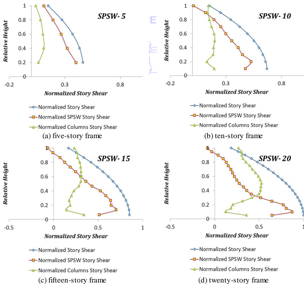
Fig. 2 Normalized story shear force, the shear force absorbed by walls, and also the force in the columns
