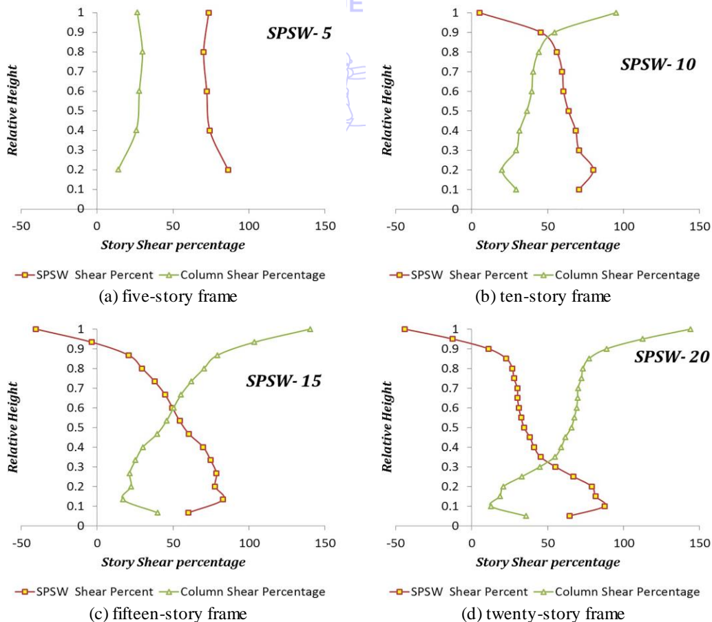
Fig. 3 Percentage of story shears absorption by steel plate shear walls and columns
