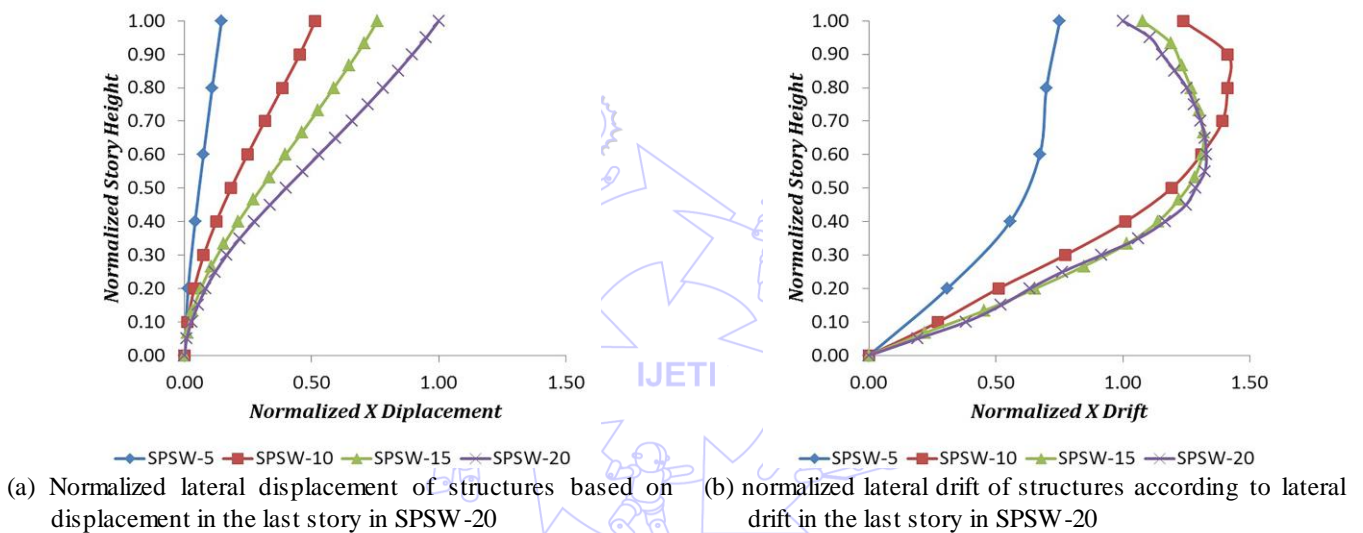
Fig. 5 Normalized lateral displacement and drift
