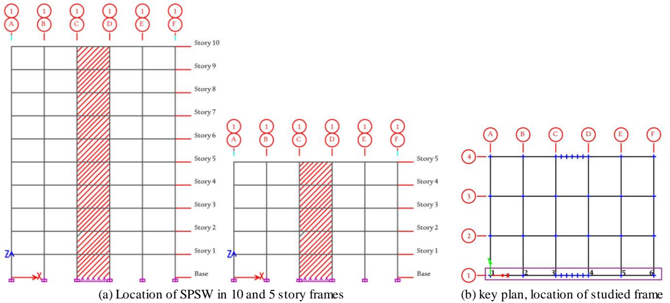
Fig. 1 Elevation and plan of modeled structures
