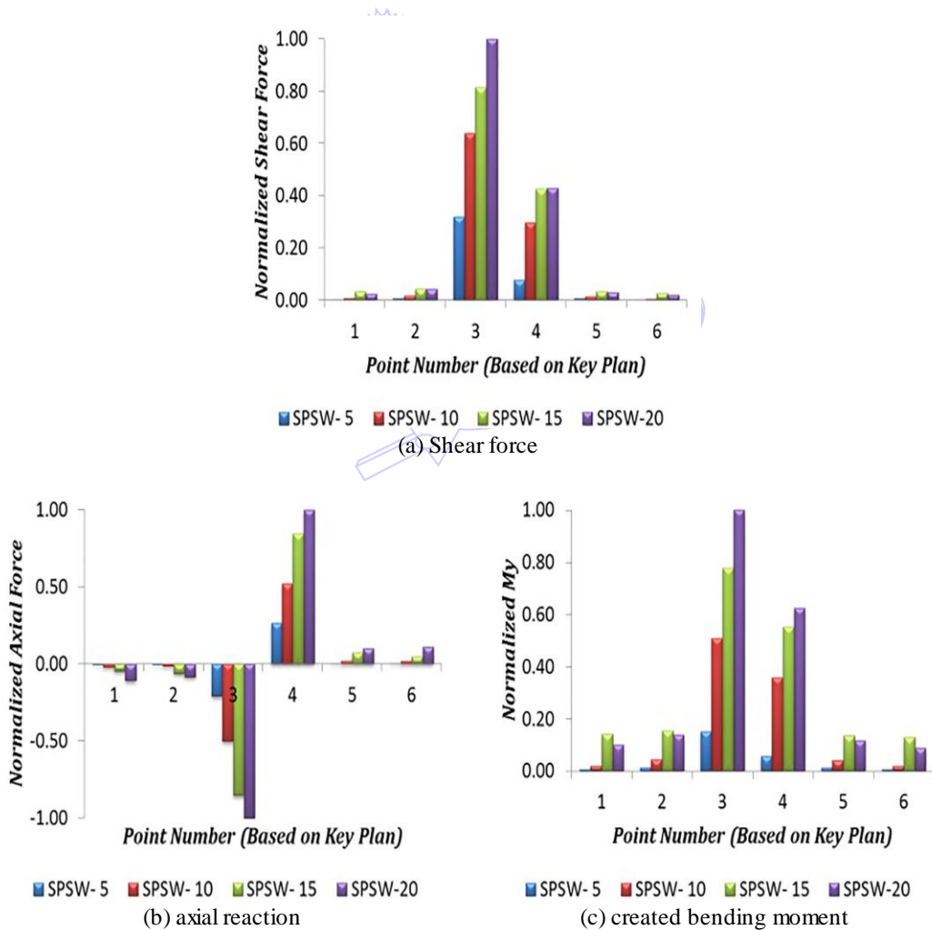
Fig. 4 Internal force in supports 1 to 6 in frame 1
