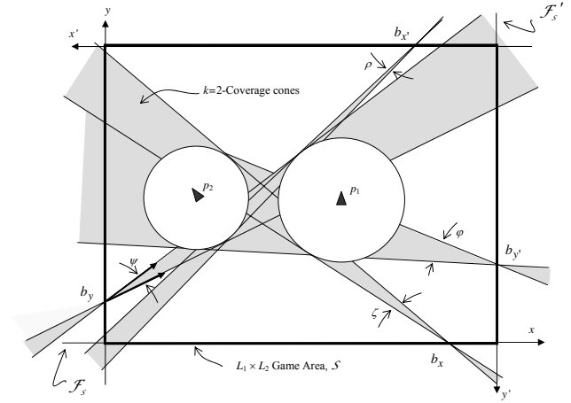
Fig. 2. Coverage cone definition illustrated for two sensors with fields of view centered at p_1 and p_2 , and a rectangular area of interest \mathcal{S} , with perimeter \partial\mathcal{S} shown in bold.
