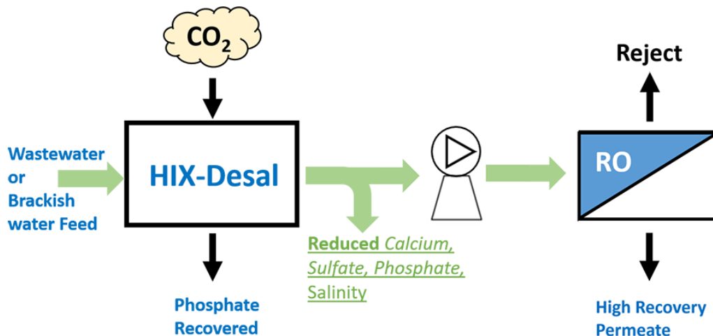
Figure 6-1. A schematic of HIX-Desal pretreatment system for RO.
