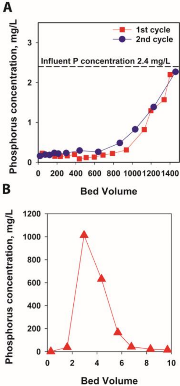
Figure 4-5. (A) Selective removal of phosphate. Influent composition and operation conditions: 100 mg/L \text{Ca}^{2+} , 300 mg/L \text{Na}^{+} , 62 mg/L \text{NO}_3^{-} , 200 mg/L \text{Cl}^{-} , 80 mg/L \text{SO}_4^{2-} , balanced \text{HCO}_3^{-} , 2.4 mg/L P, TDS 1250 mg/L, pH 7, SLV 1.4 m/h, EBCT 3.3 min. (B) Elution of phosphate with 2% KOH.
