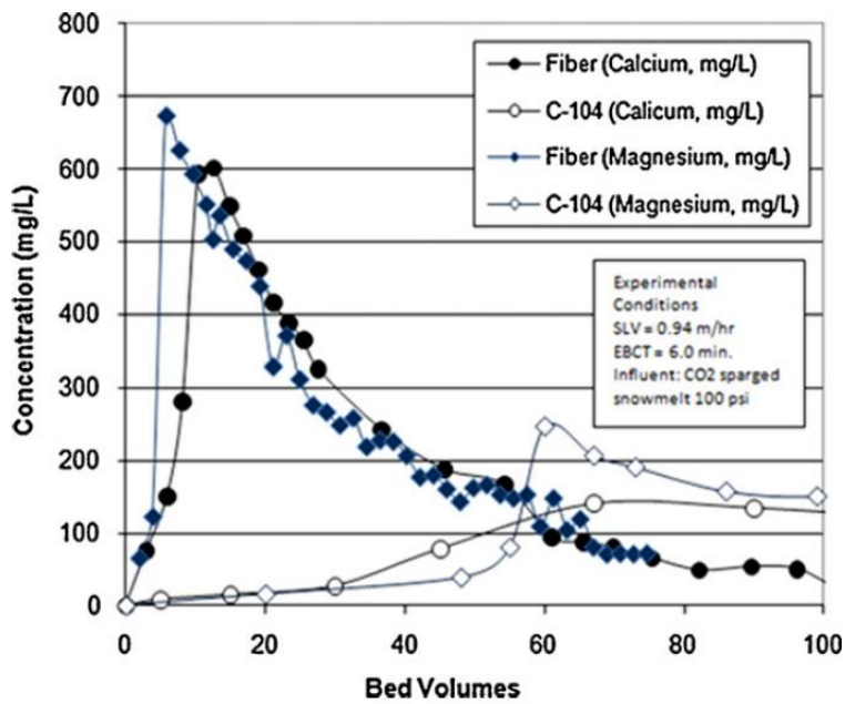
Figure 3-6. Regeneration comparison between virgin weak acid fibers and resins loaded with divalent cations using carbon dioxide under 100 psi. (Padunghon et al., 2011)
