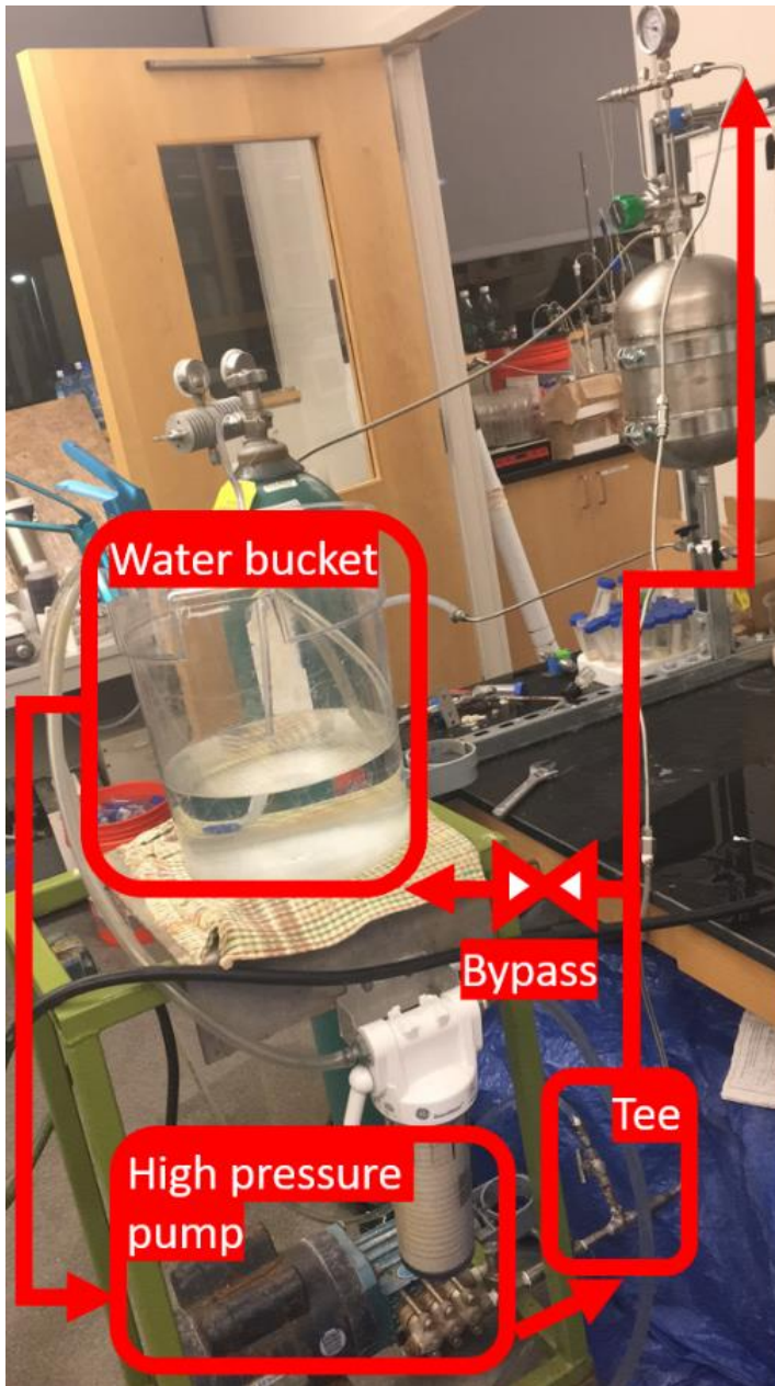
Figure 3-3. Continuous water supply system to pump water into pressurized regeneration tank at small flowrate.
