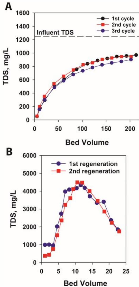
Figure 4-4. (A) Desalination performance over three consecutive service cycles using Bethlehem secondary wastewater. Influent composition and operation conditions: 100 mg/L \text{Ca}^{2+} , 300 mg/L \text{Na}^{+} , 62 mg/L \text{NO}_3^{-} , 200 mg/L \text{Cl}^{-} , 80 mg/L \text{SO}_4^{2-} , balanced \text{HCO}_3^{-} , 2.4 mg/L P, TDS 1250 mg/L, pH 7, SLV 1.4 m/h, EBCT 3.3 min. (B) TDS elution during \text{CO}_2 regeneration. Regenerant and operation conditions: \text{CO}_2 sparged water under 150 psi \text{CO}_2 partial pressure, EBCT 30 min. (EBCT= Empty bed contact time).
