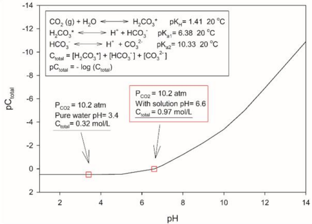
Figure 4-8. Total carbon dioxide concentration changes under 10.2 atm partial pressure.
