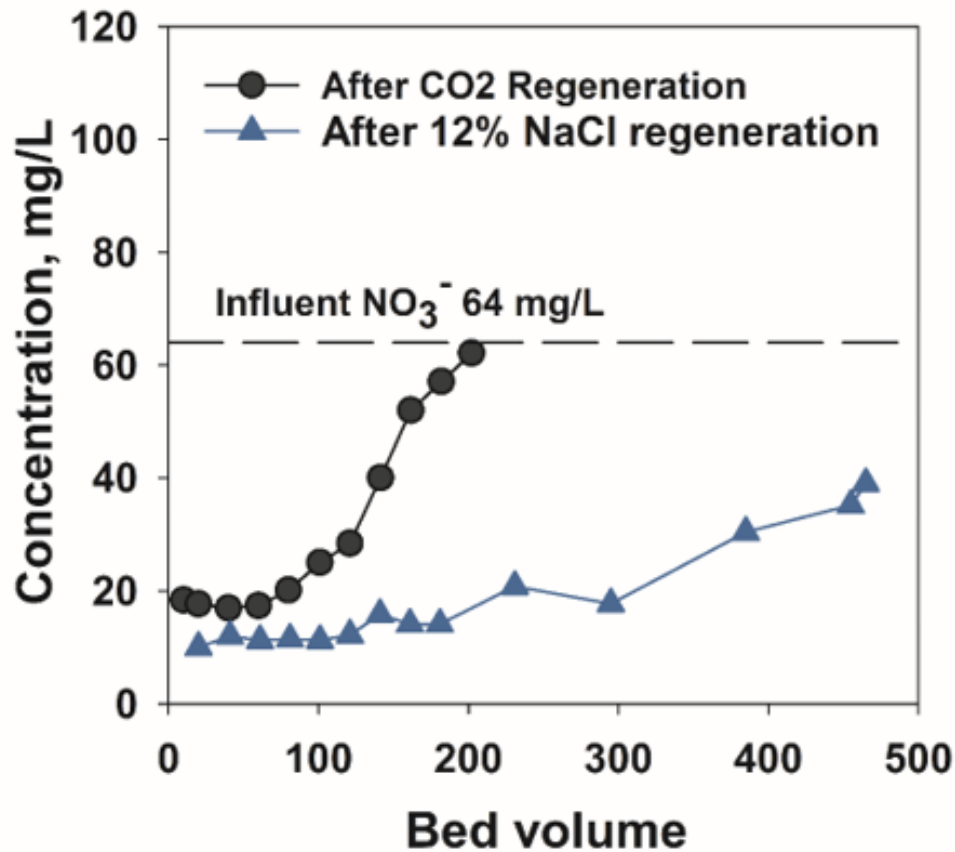
Figure 5-5. Comparison of treatment between proposed carbon dioxide sustained process and typical 12% NaCl regeneration cycles. Influent composition and operation conditions: 64 mg/L \text{NO}_3^- , 5.4 mg/L \text{F}^- , 40 mg/L \text{Cl}^- , 60 mg/L \text{SO}_4^{2-} , 274 mg/L \text{HCO}_3^- , 90 mg/L \text{Ca}^{2+} , 70 mg/L \text{Na}^+ , conductivity 791 \mu\text{s}/\text{cm} , pH 7, SLV 1.4 m/h, EBCT 3.3 min.
