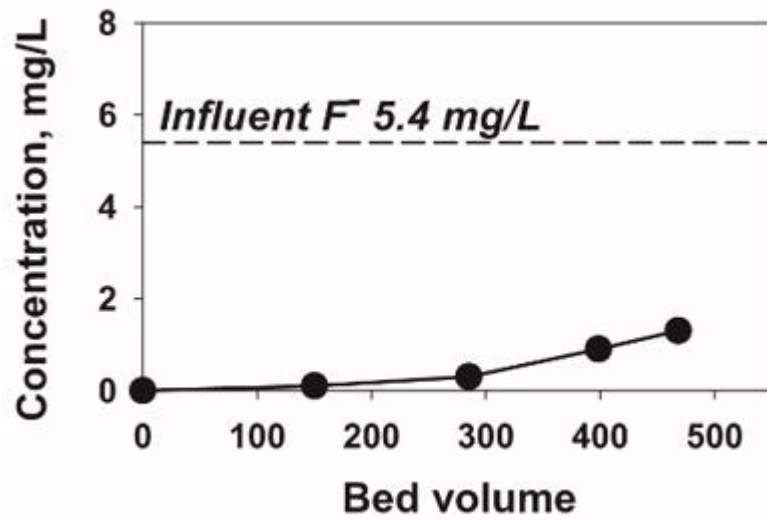
Figure 5-2. Fluoride removal. Influent composition and operation conditions: 64 mg/L \text{NO}_3^- , 5.4 mg/L \text{F}^- , 40 mg/L \text{Cl}^- , 60 mg/L \text{SO}_4^{2-} , 274 mg/L \text{HCO}_3^- , 90 mg/L \text{Ca}^{2+} , 70 mg/L \text{Na}^+ , conductivity 791 \mu\text{s}/\text{cm} , pH 7, SLV 1.4 m/h, EBCT 3.3 min.
