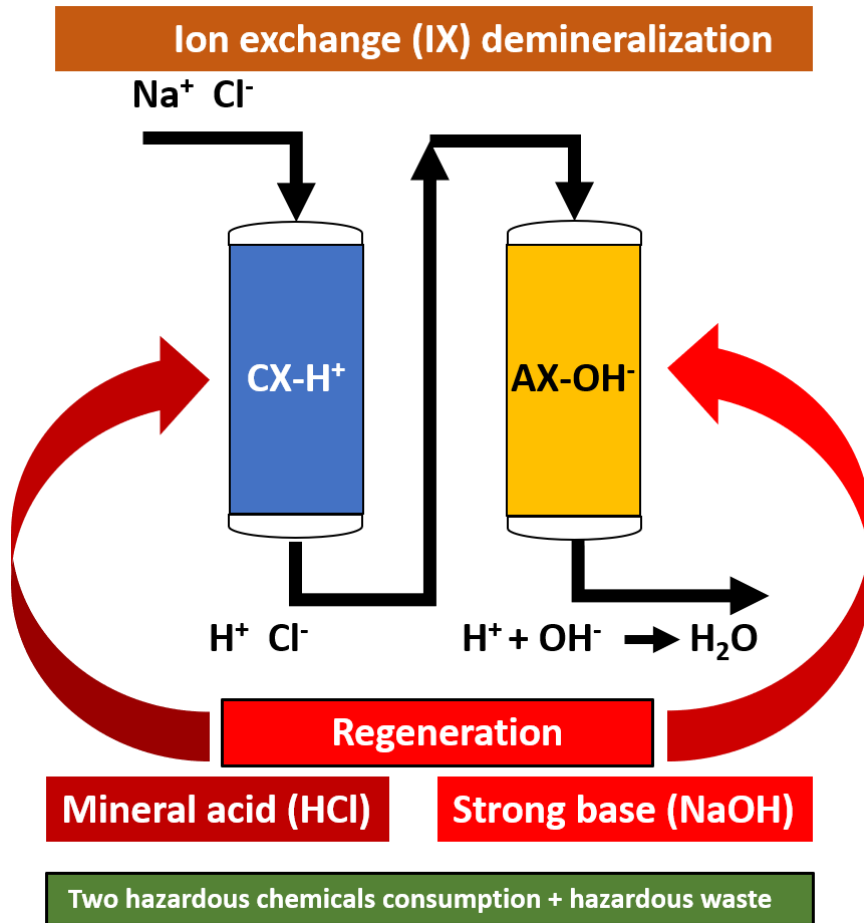
Figure 1-9. A schematic describes conventional ion exchange demineralization using two hazardous chemicals and producing hazardous waste.
