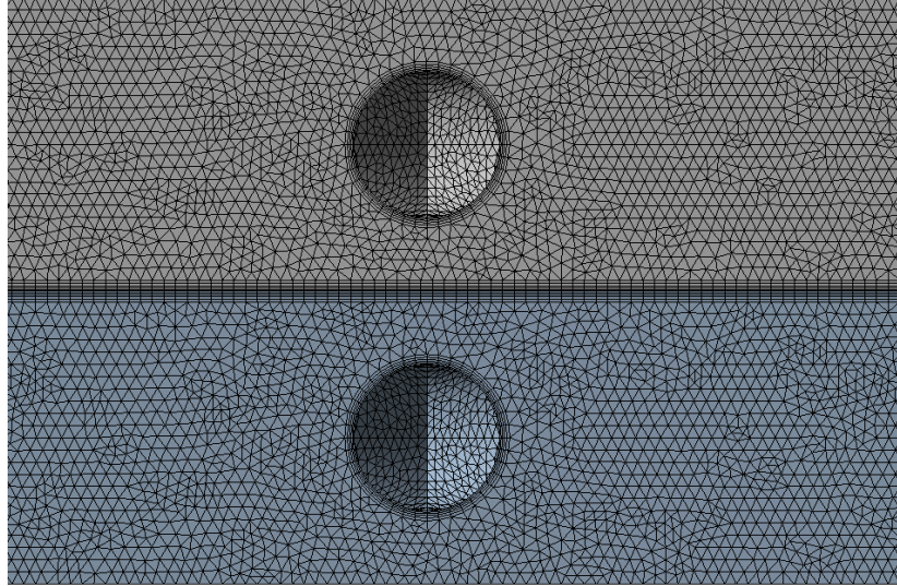
Figure 10. A sample of the unstructured mesh for the geometry with net-type spacers.
