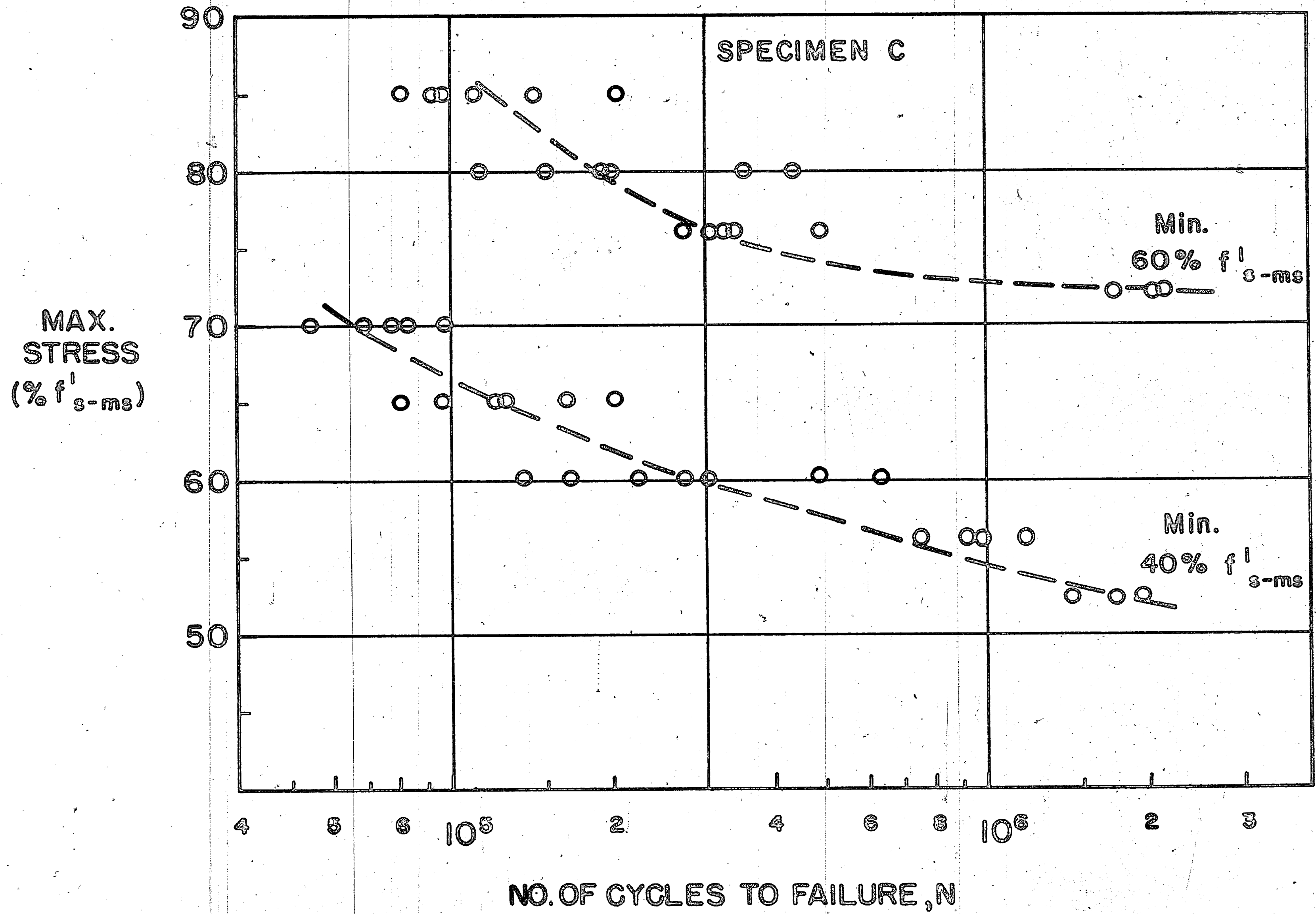
Fig. 15 Maximum Stress Level vs. Fatigue Life, Specimen C
