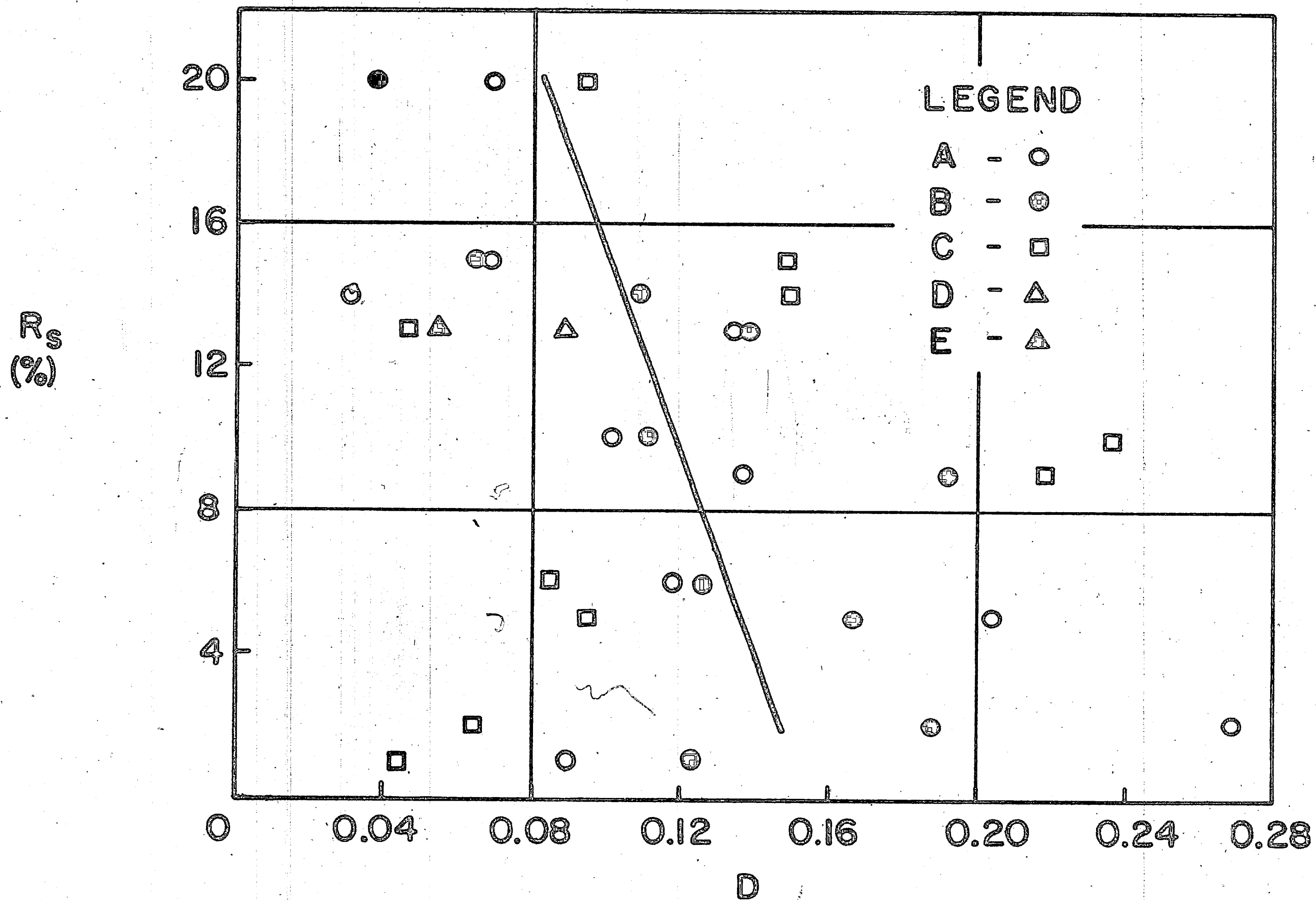
Fig. 21 Standard Deviation D vs. Load Range R_s
