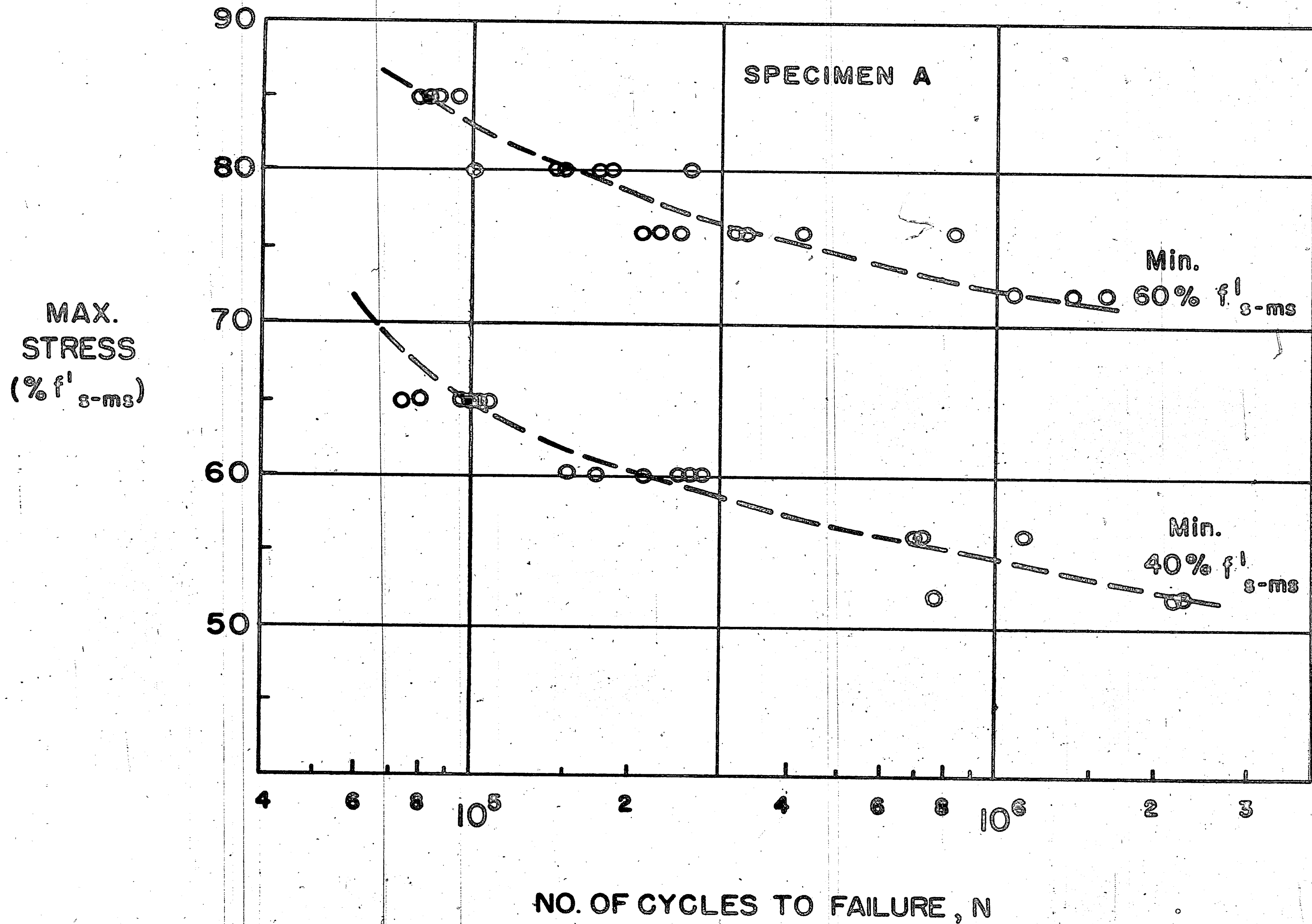
Fig. 13 Maximum Stress Level vs. Fatigue Life, Specimen A
