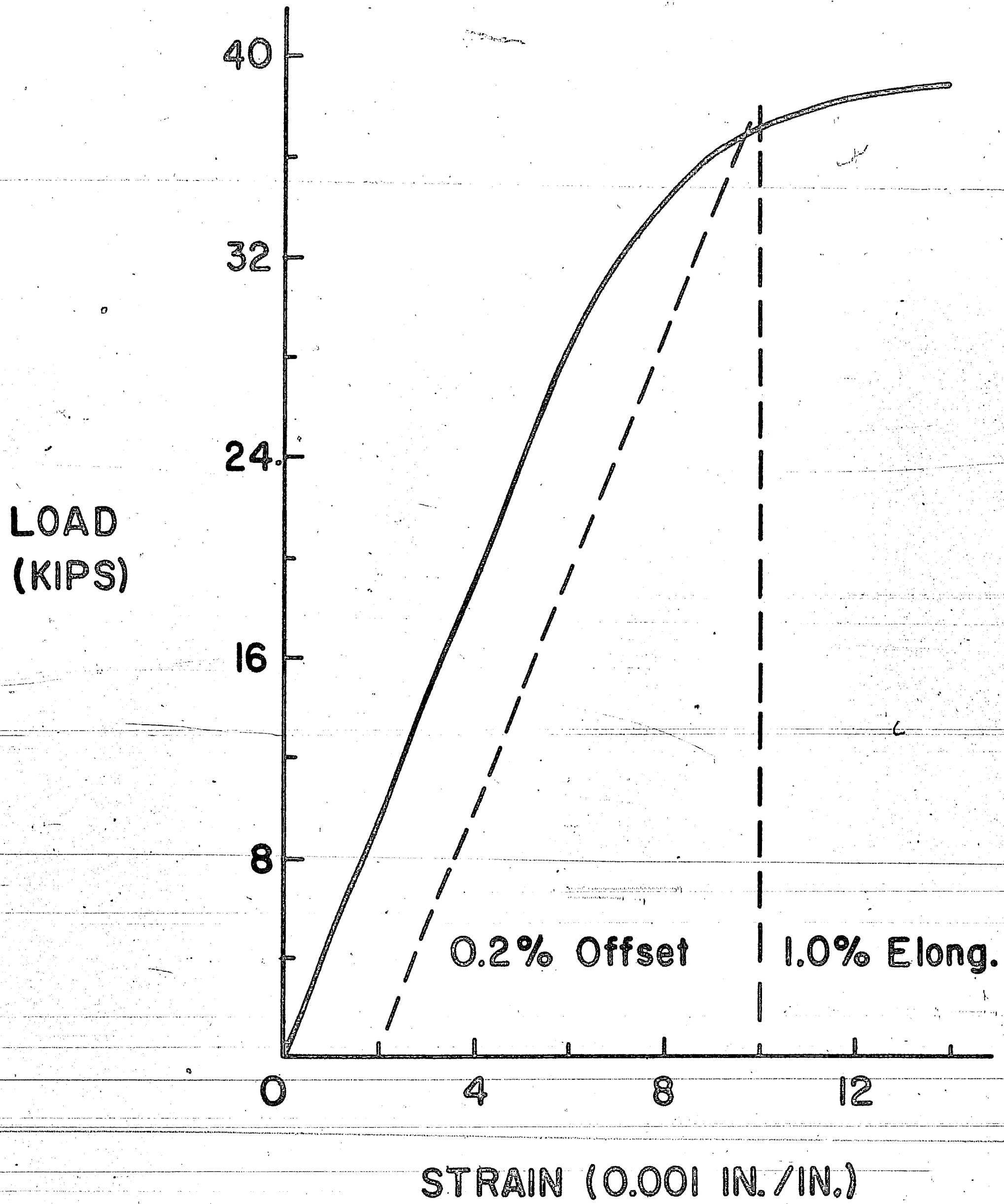
Fig. 2 Yield Strength for Prestressing Strand
