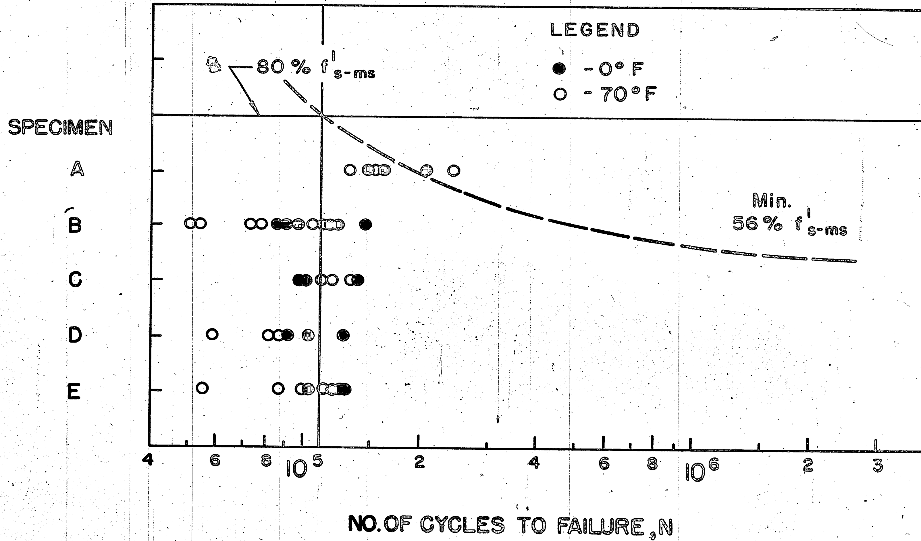
Fig. 18 Effect of Lowering Temperature on Fatigue Life
