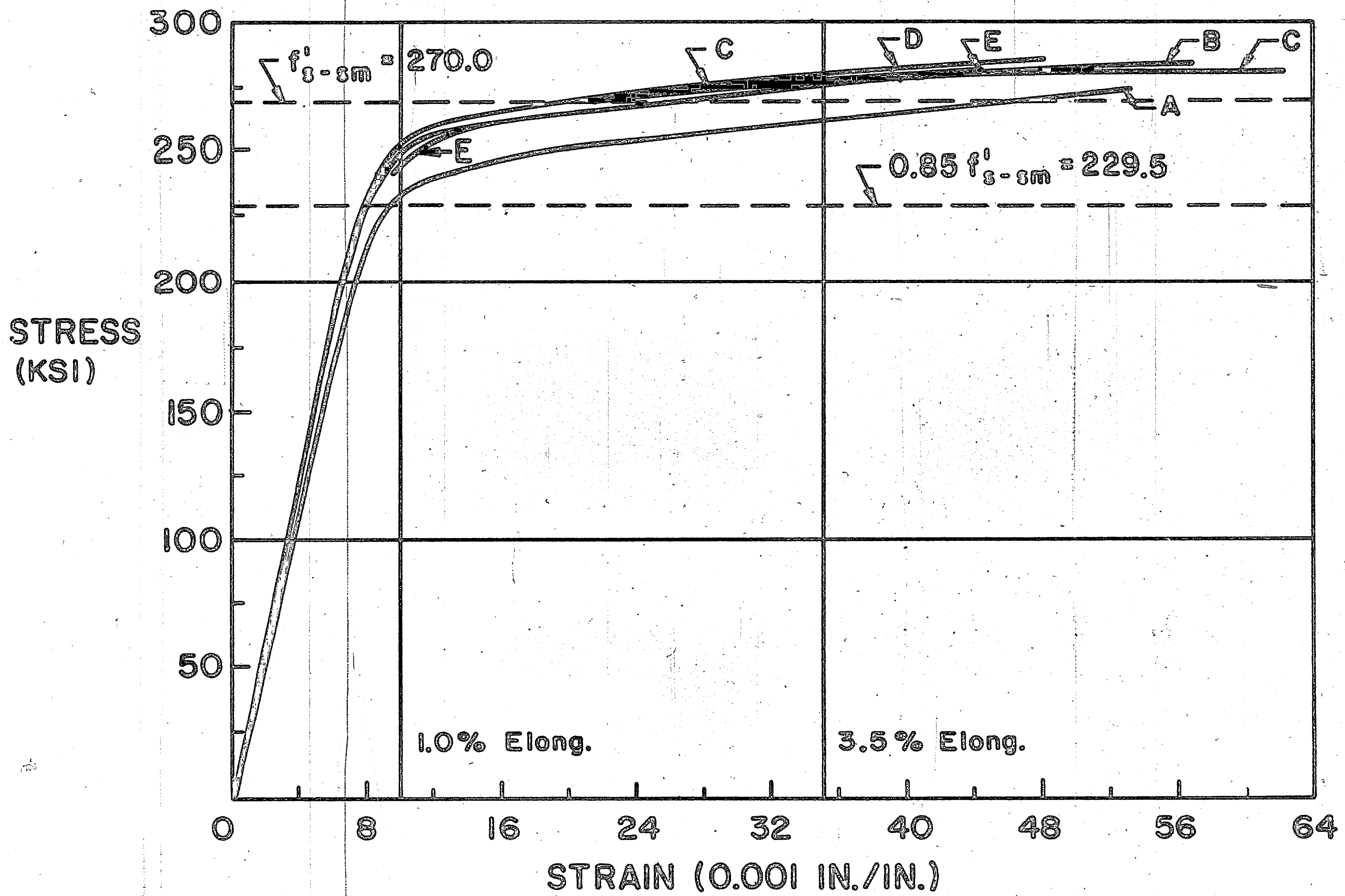
Fig. 8 Typical Stress-Strain Relationships for Prestressing Strand
