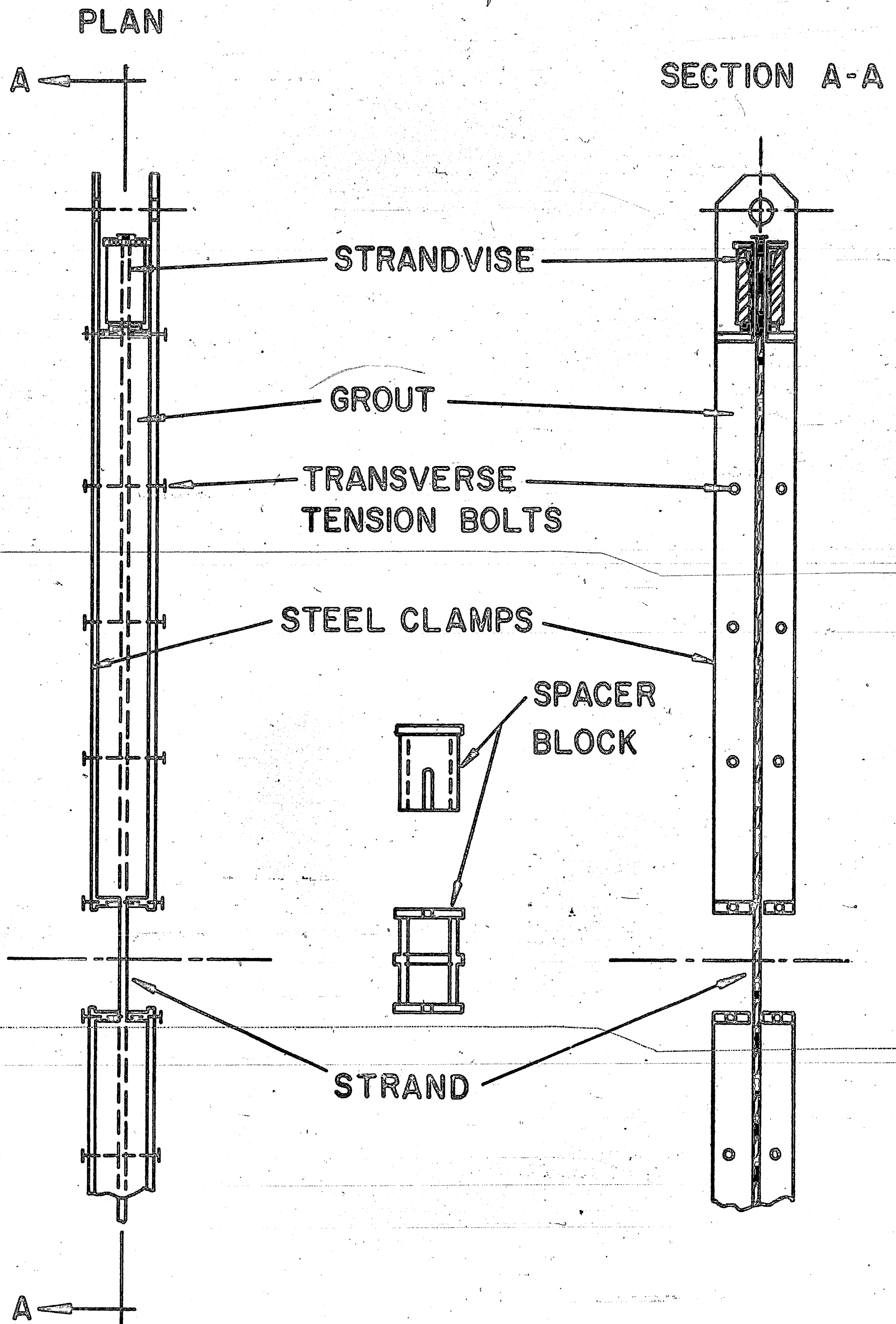
Fig. 9 Fatigue Test Specimens
