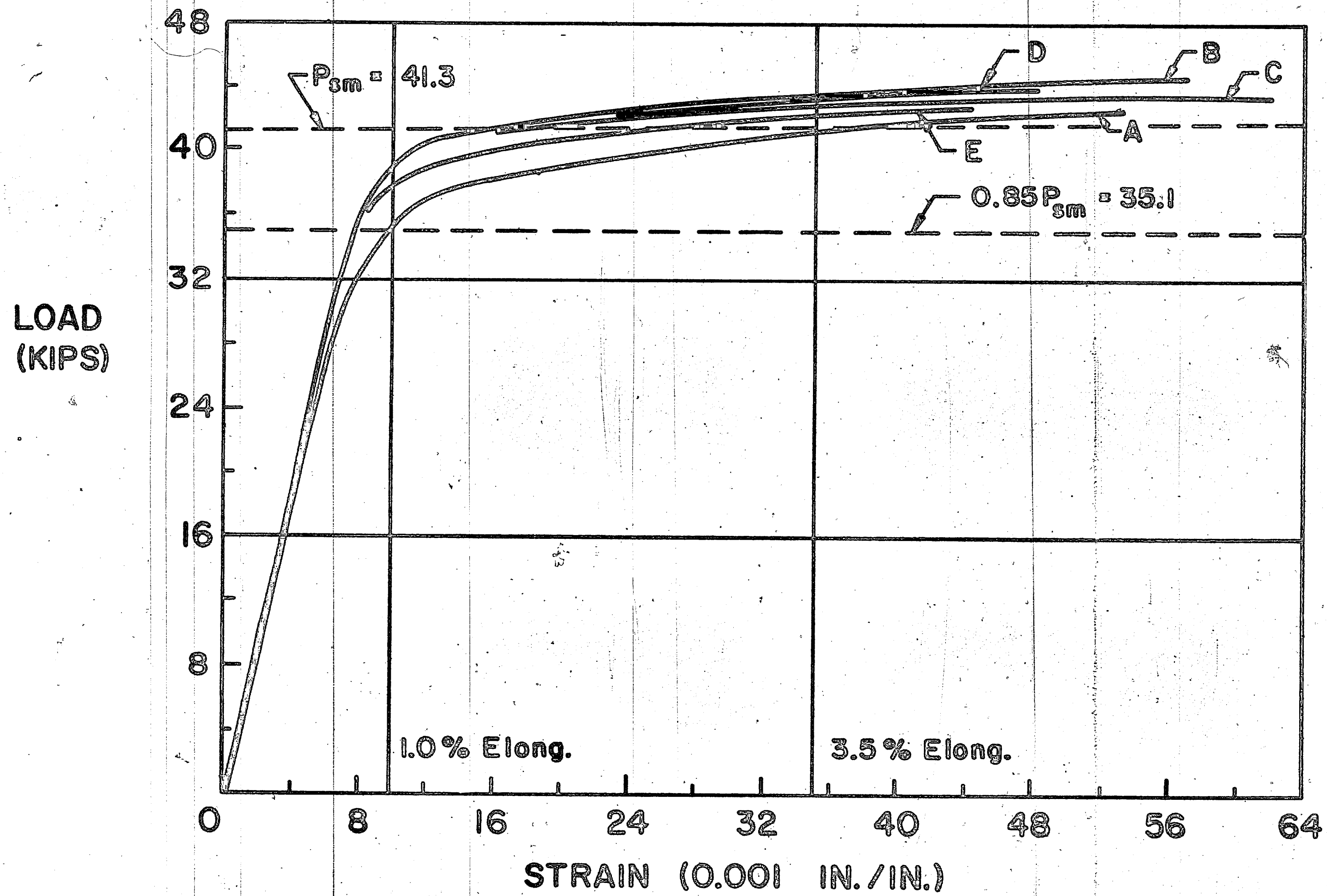
Fig. 7 Typical Load-Strain Relationships for Prestressing Strand
