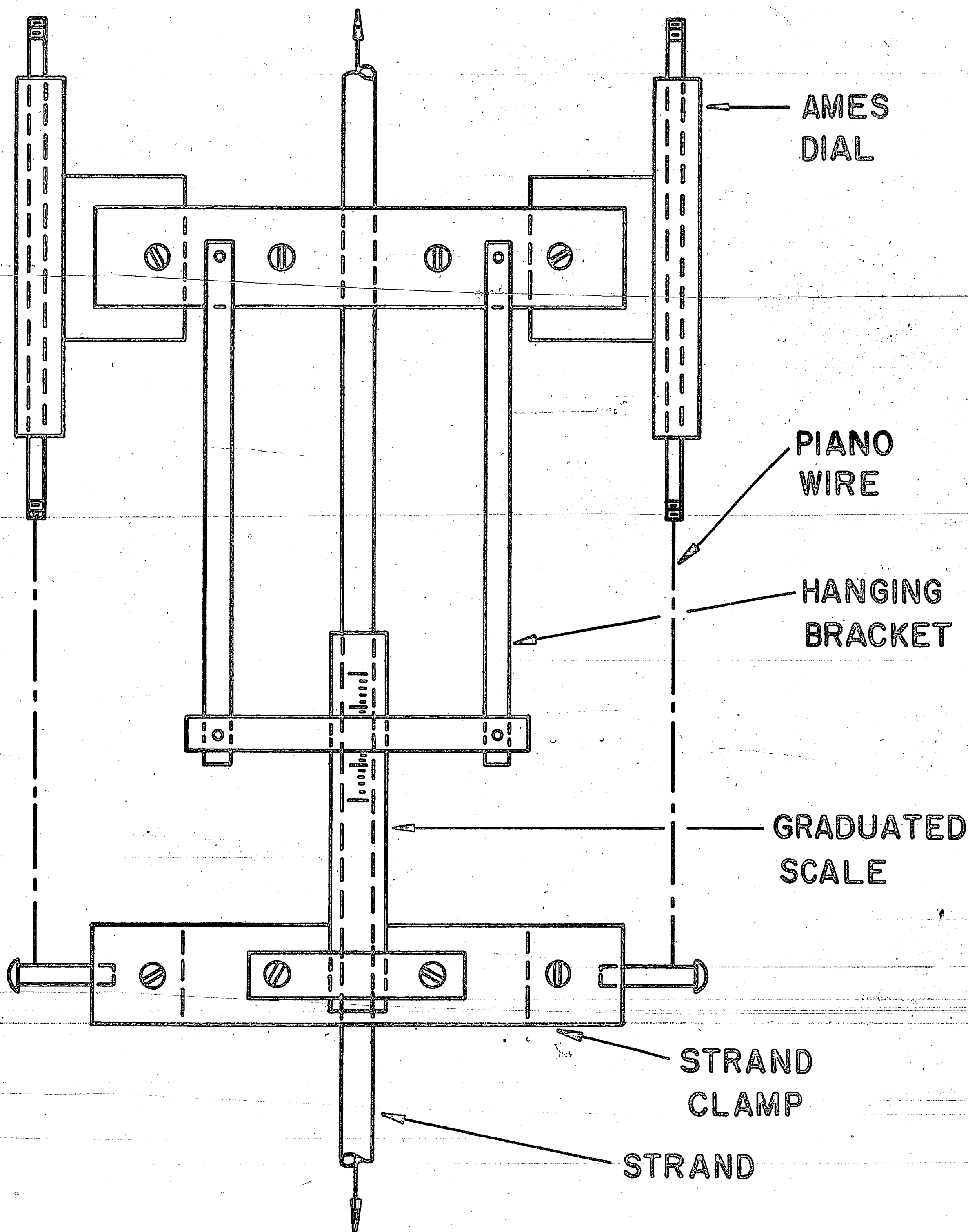
Fig. 5 Extensometer - Static Tests
