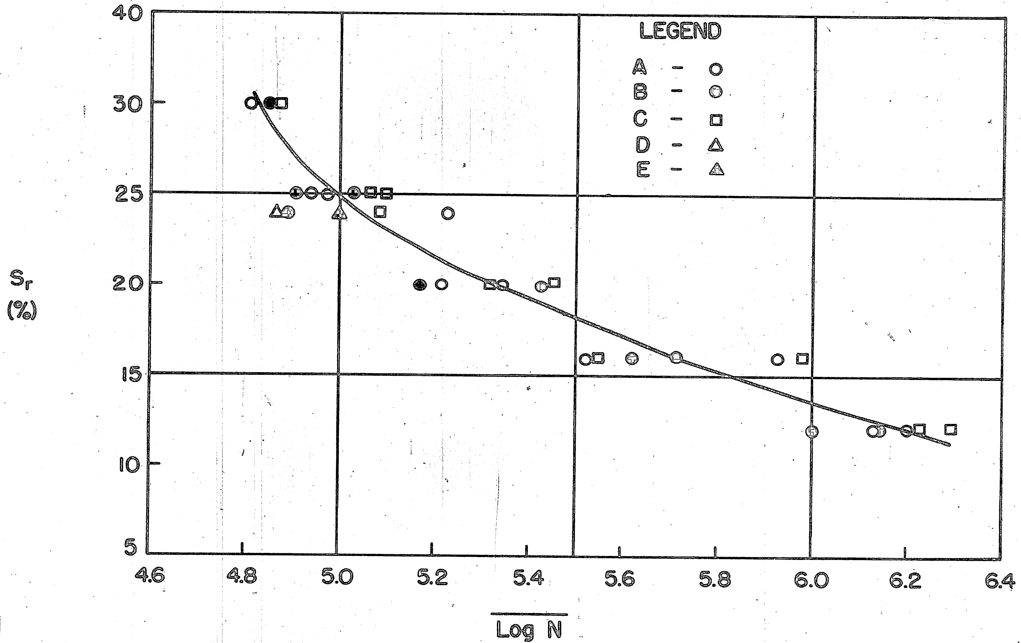
Fig. 20 \overline{\text{Log N}} vs. Load Range R_s
