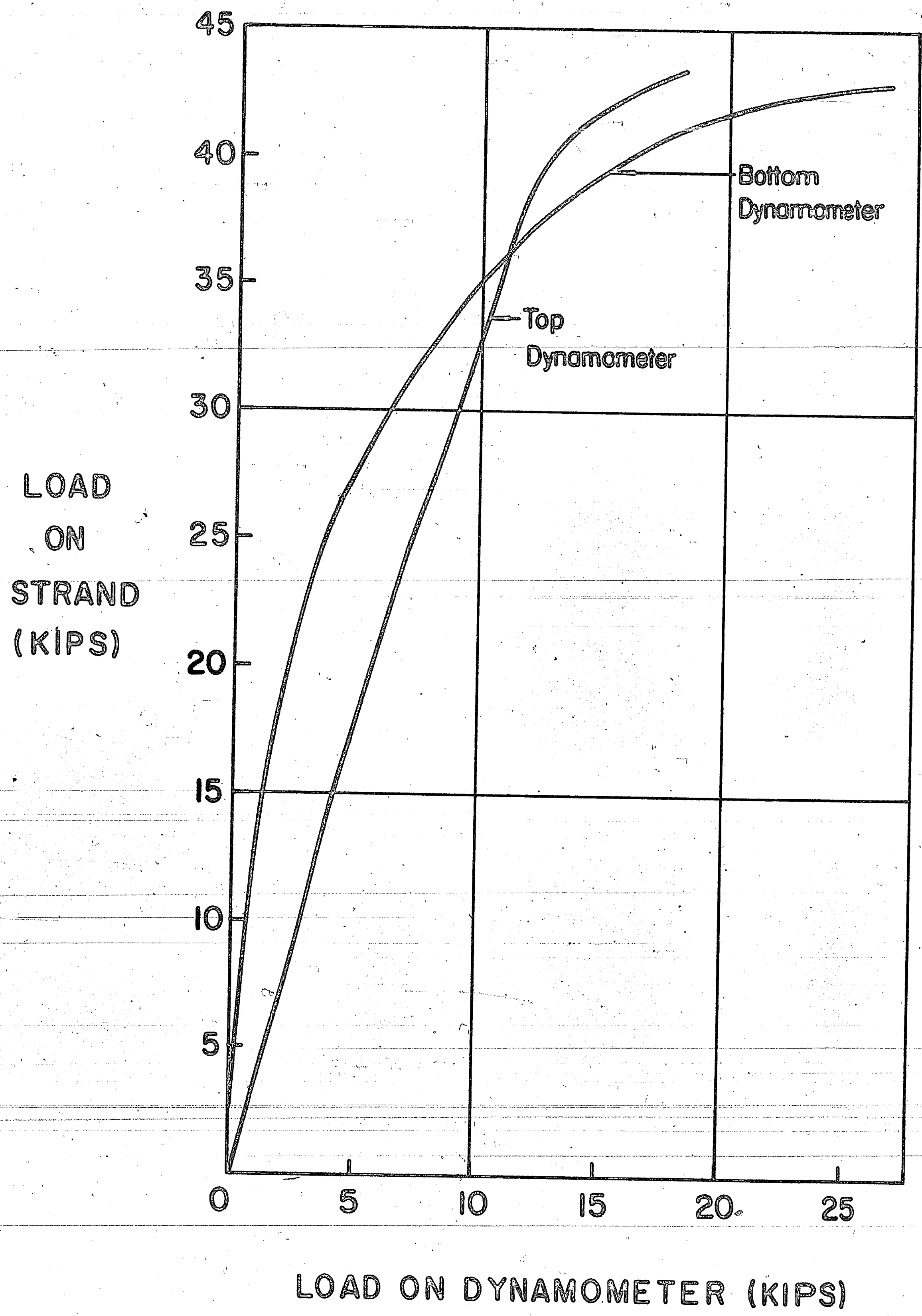
Fig. 4 Effectiveness of the Copper Grips
