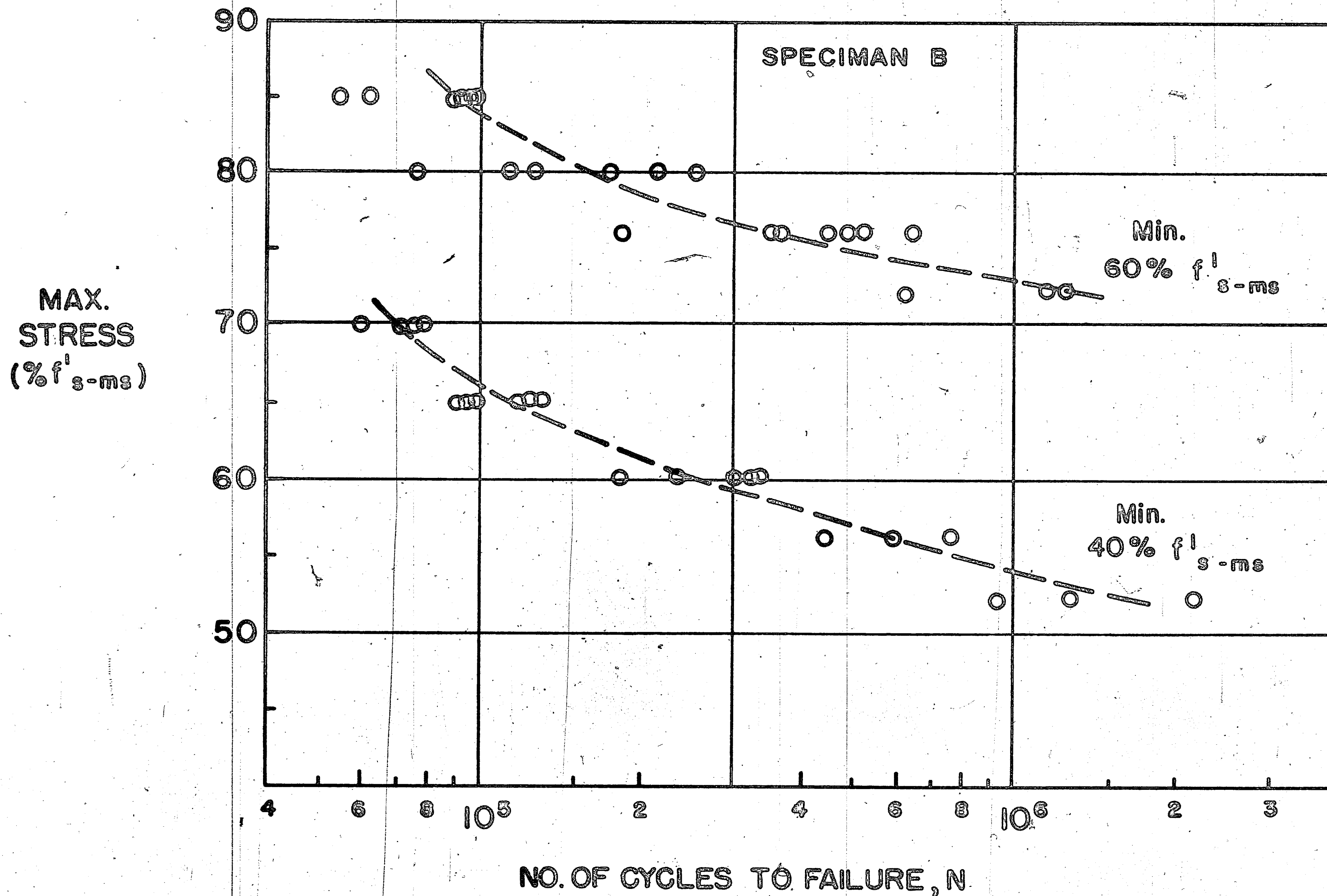
Fig. 14 Maximum Stress Level vs. Fatigue Life, Specimen B
