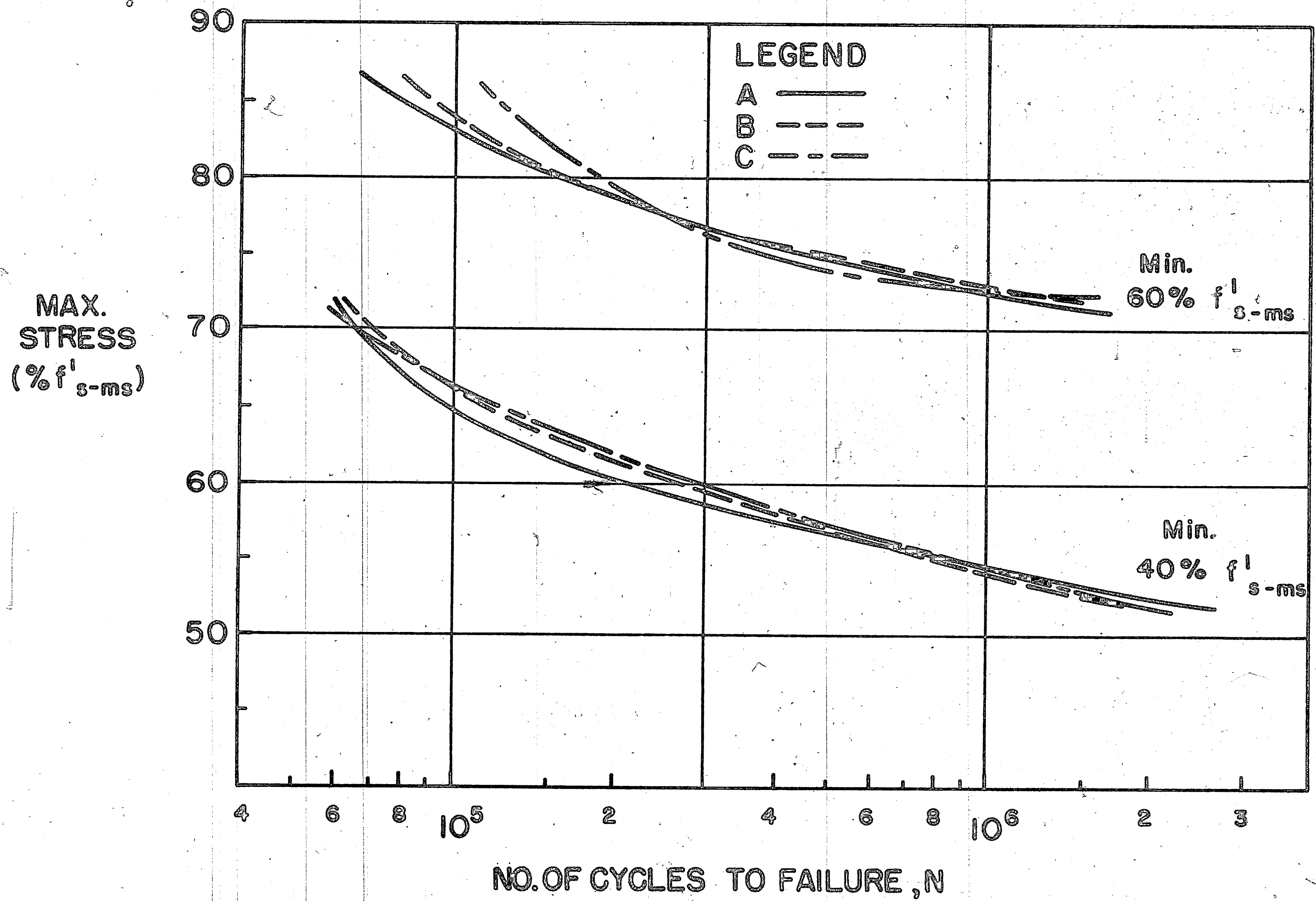
Fig. 16 Comparison of Fatigue Life of Various Manufacturers
