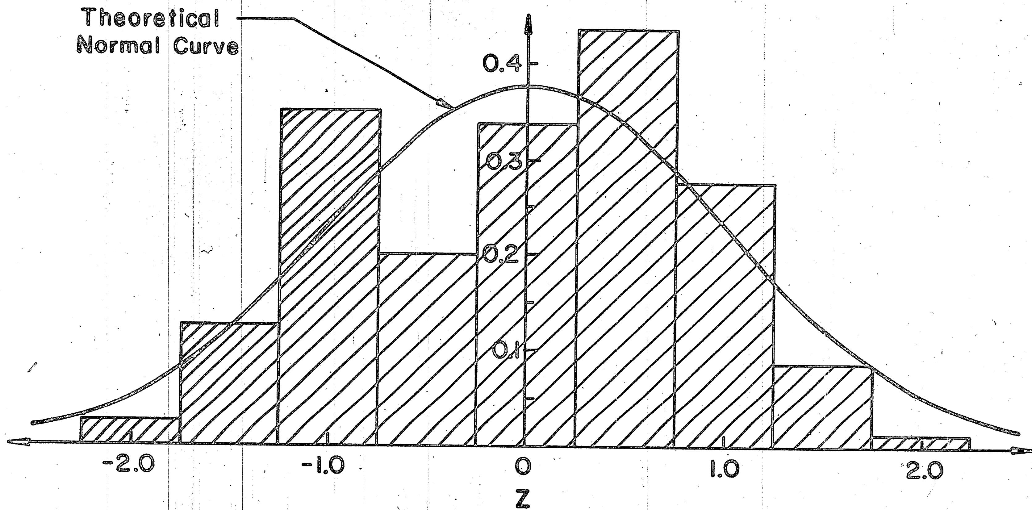
Fig. 19 Frequency Distribution of Grouped Constant Cycle Test Data
