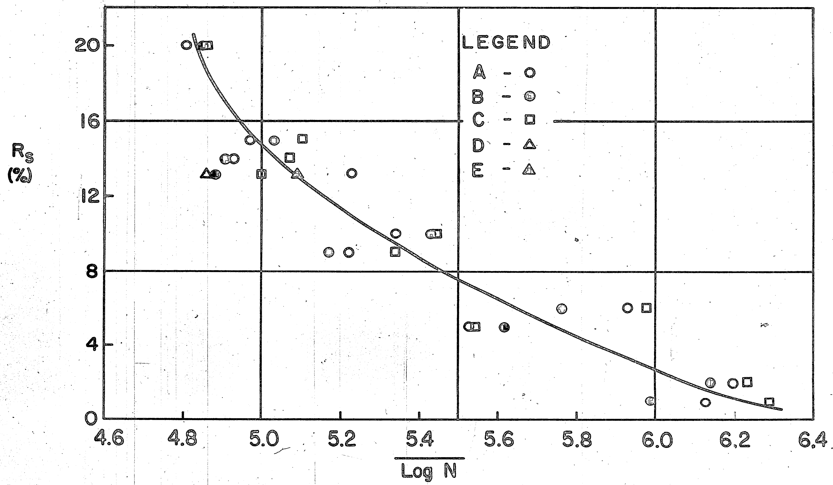
Fig. 22 \overline{\text{Log N}} vs. Stress Range S r
