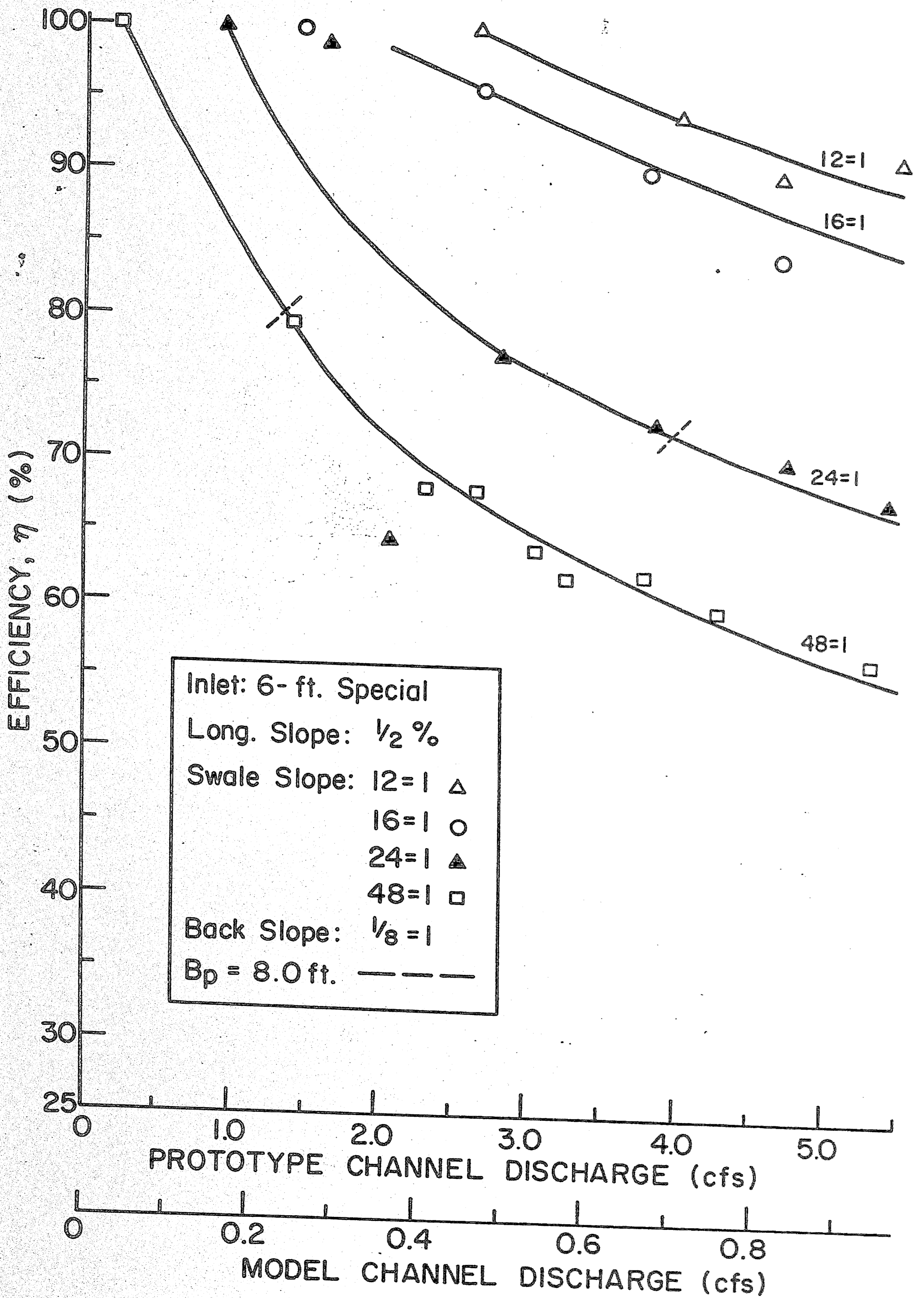
Fig. 4.9 Efficiency Curves; 6-Ft Special (Long. Slope = \frac{1}{2}\% )
