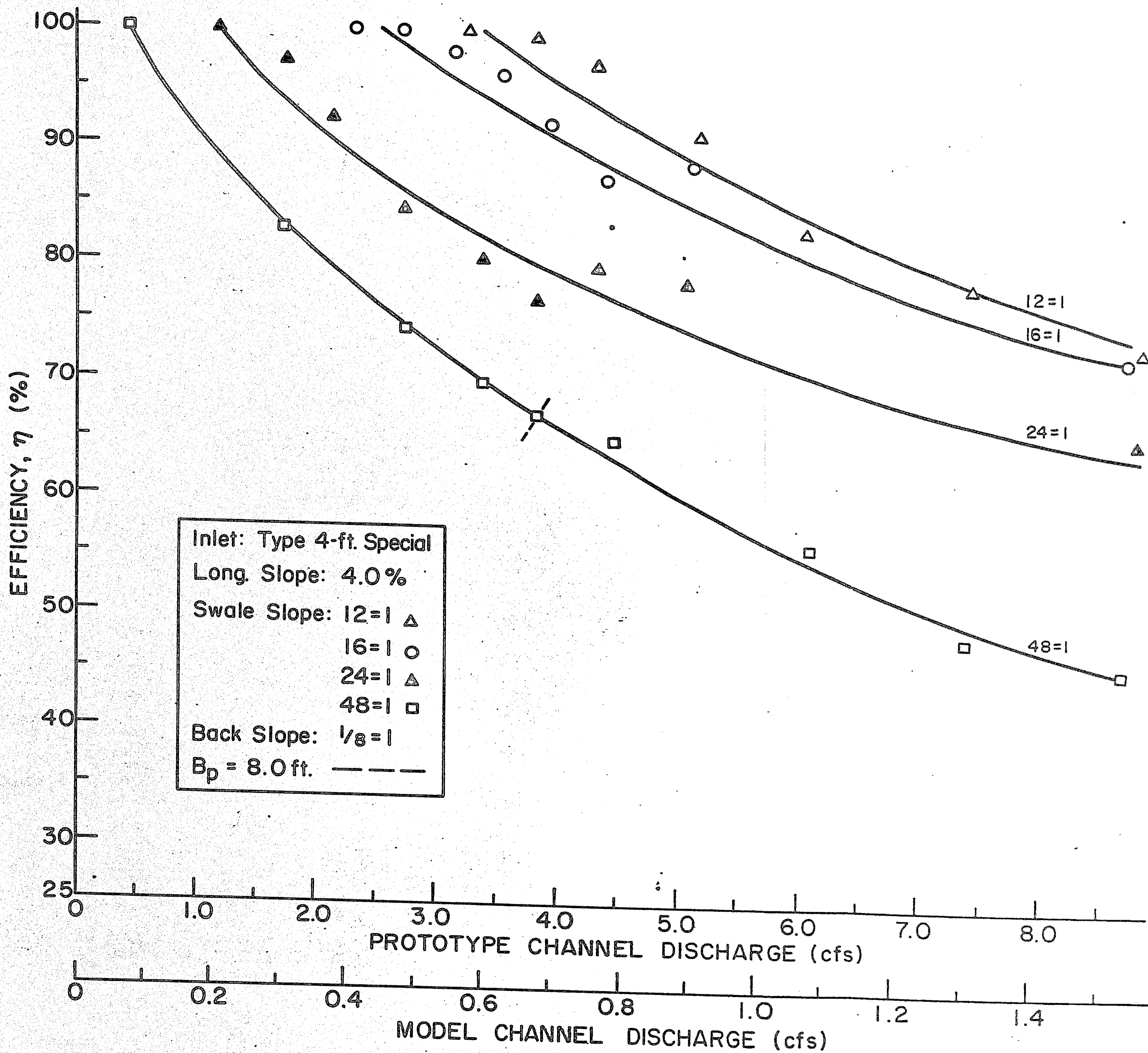
Fig. 4.7 Efficiency Curves; 4-Ft Special (Long. Slope = 4%)
