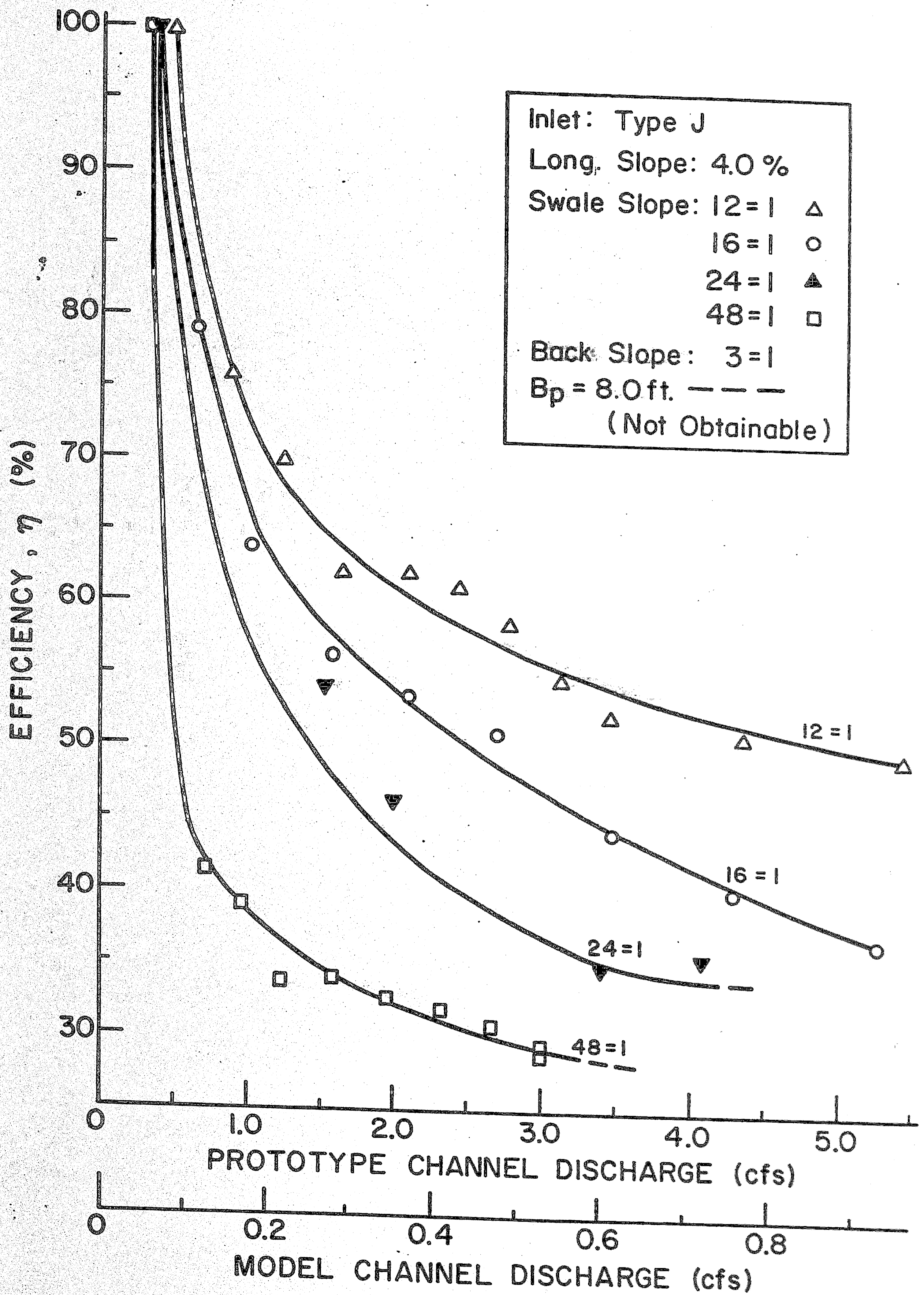
Fig. 4.3 Efficiency Curves; Type J Inlet (Long. Slope = 4%)
