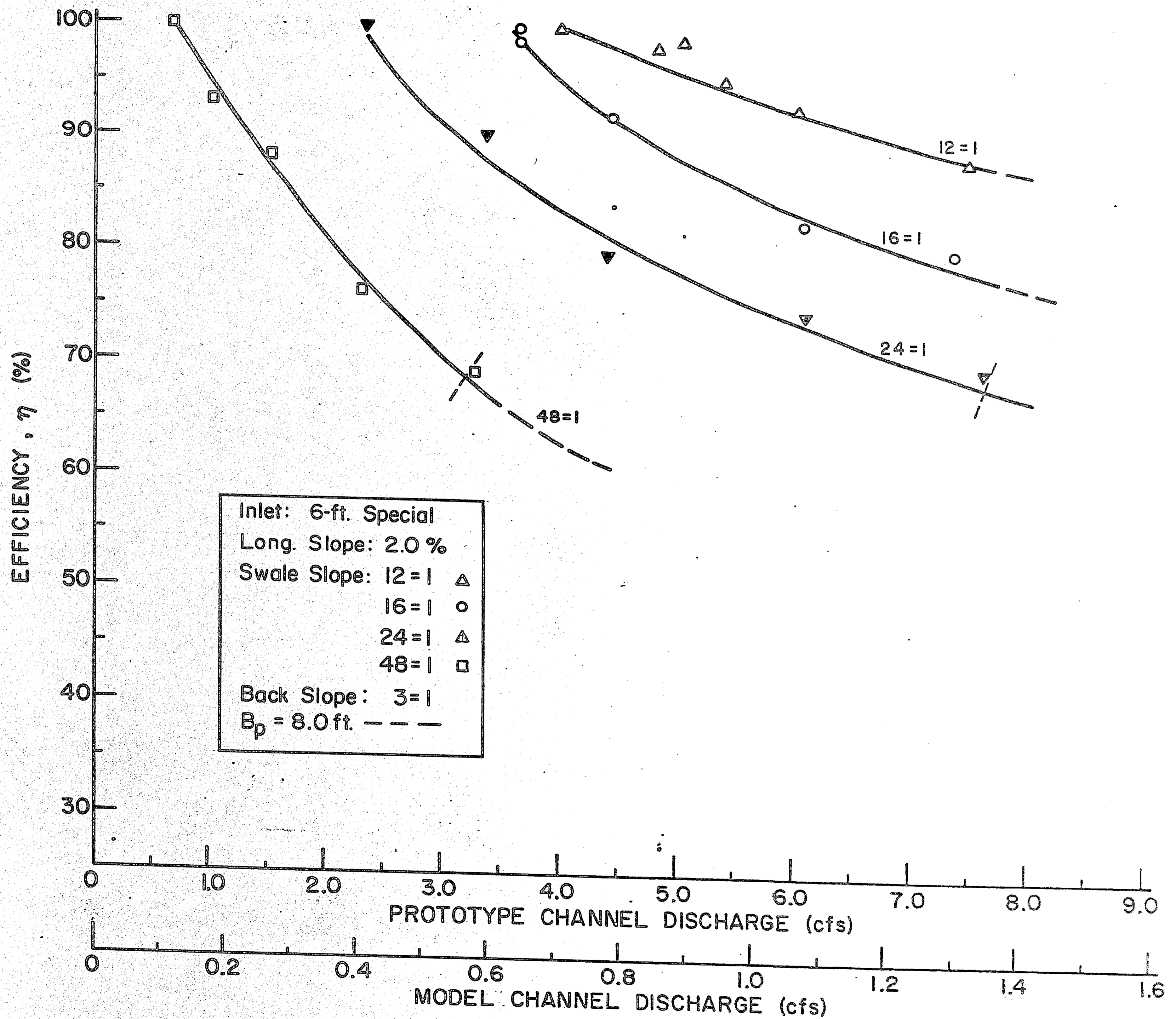
Fig. 4.10 Efficiency Curves; 6-Ft Special (Long. Slope = 2%)
