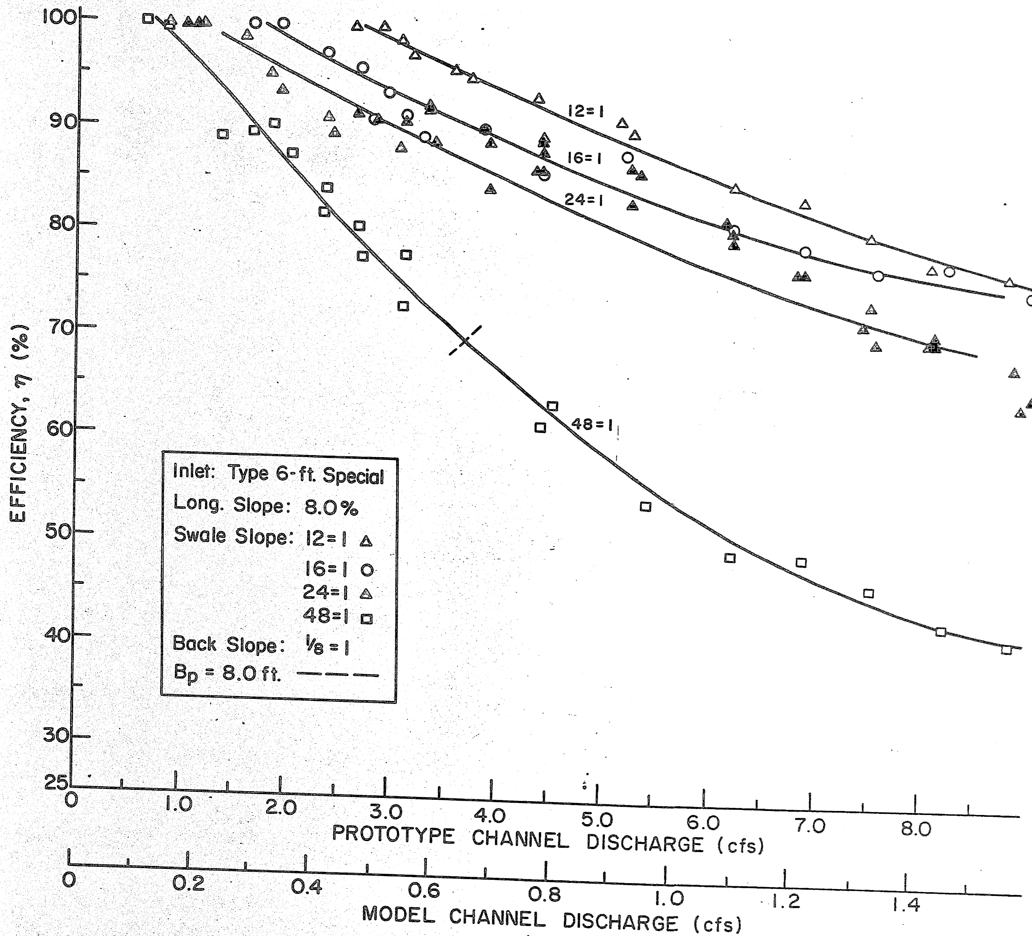
Fig. 4.12 Efficiency Curves; 6-Ft Special (Long. Slope = 8%)
