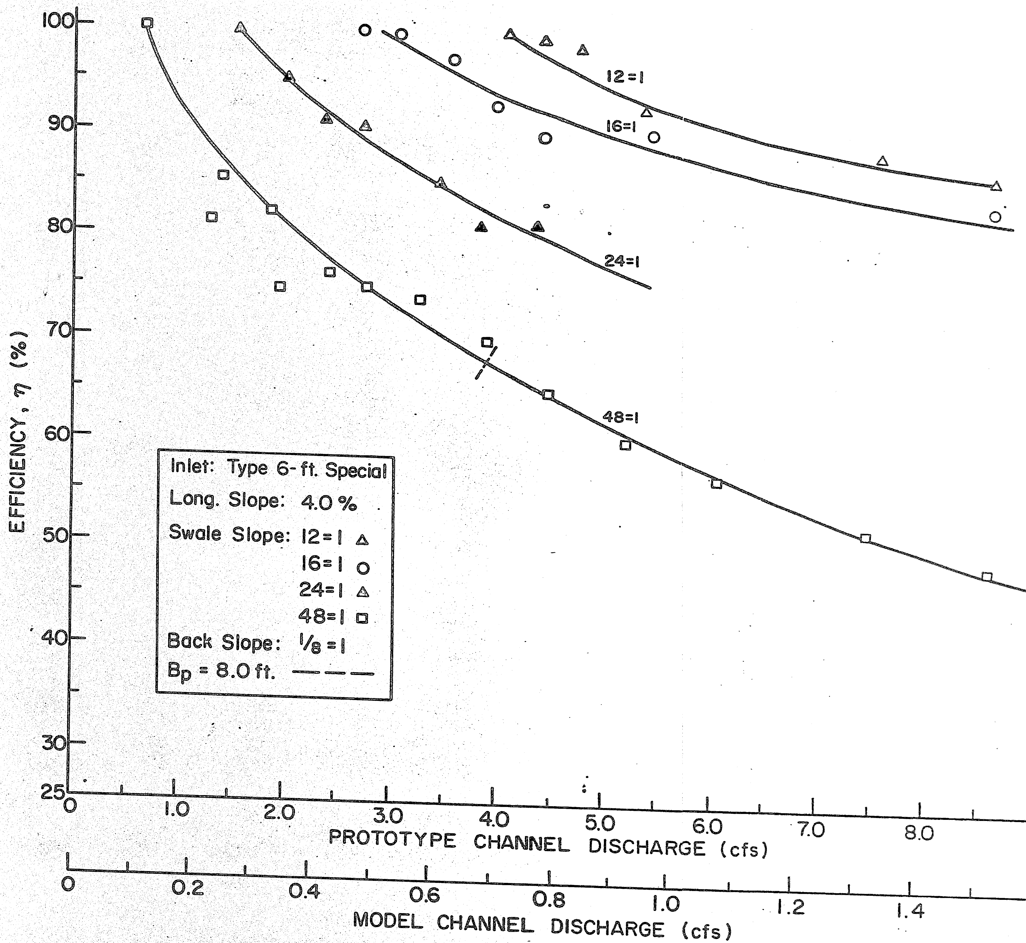
Fig. 4.11 Efficiency Curves; 6-Ft Special (Long. Slope = 4%)
