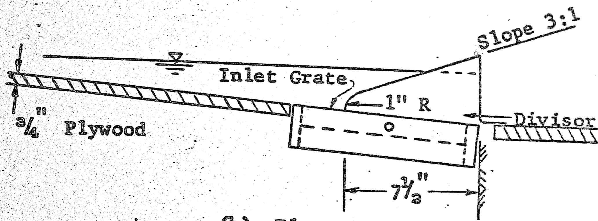
(b) Elevation View
