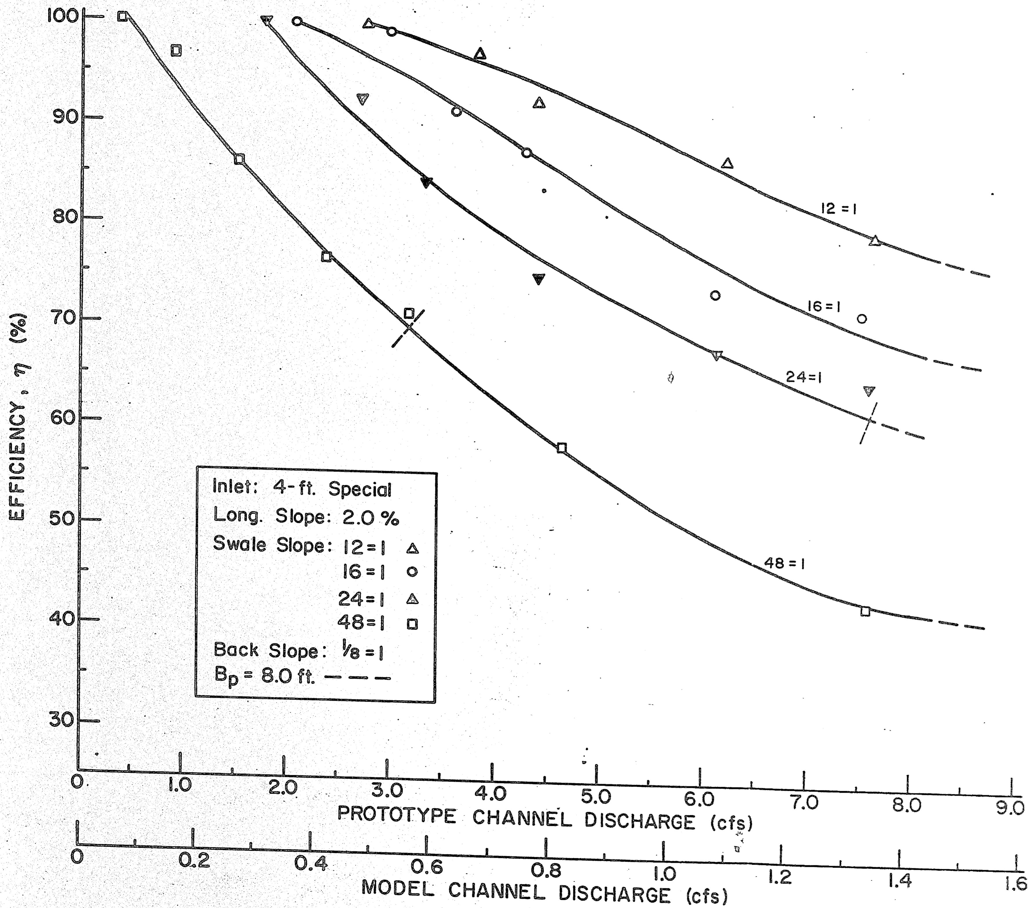
Fig. 4.6 Efficiency Curves; 4-Ft Special (Long. Slope = 2%)
