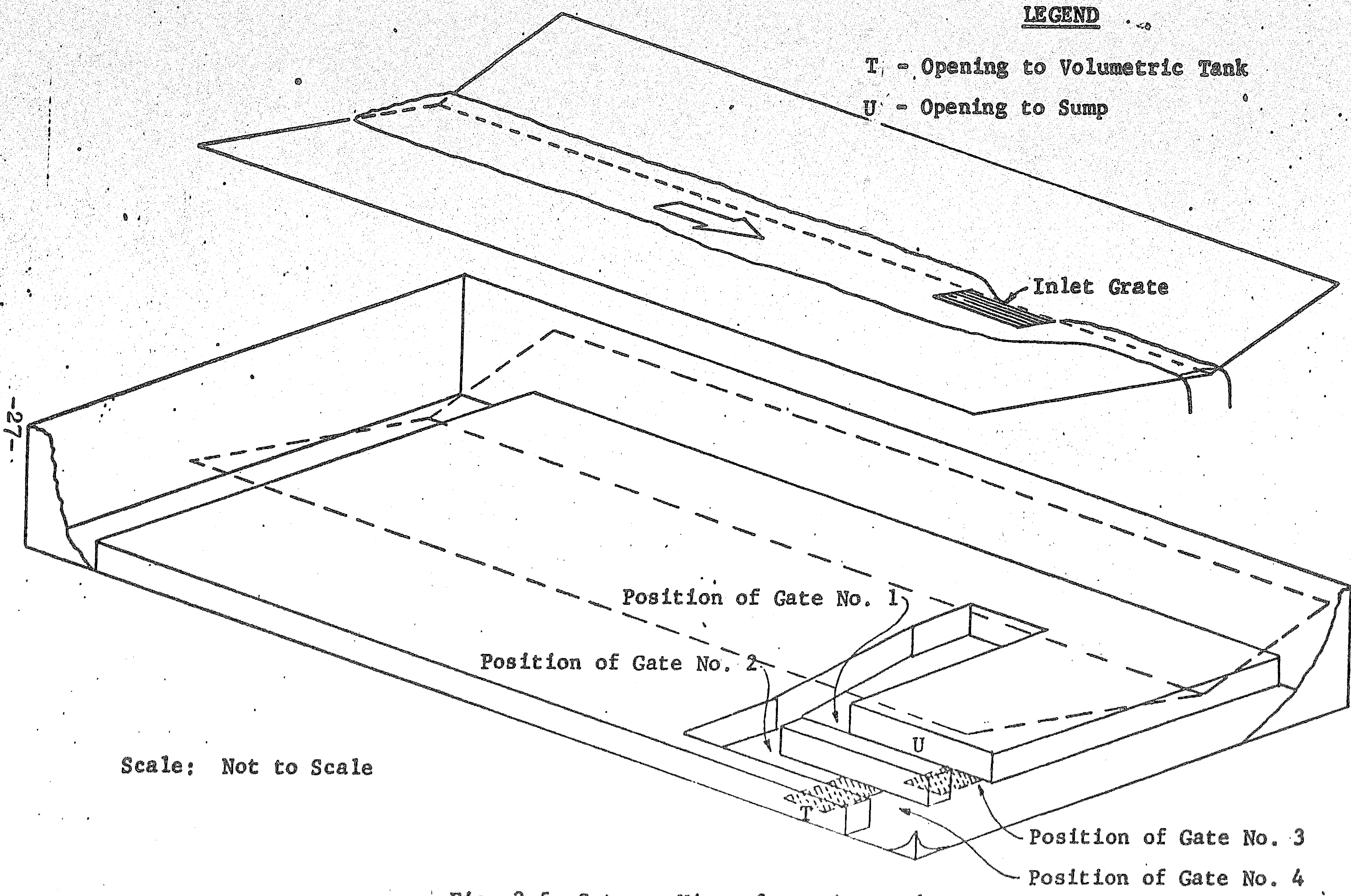
Fig. 3.5 Cutaway View of Testing Tank
