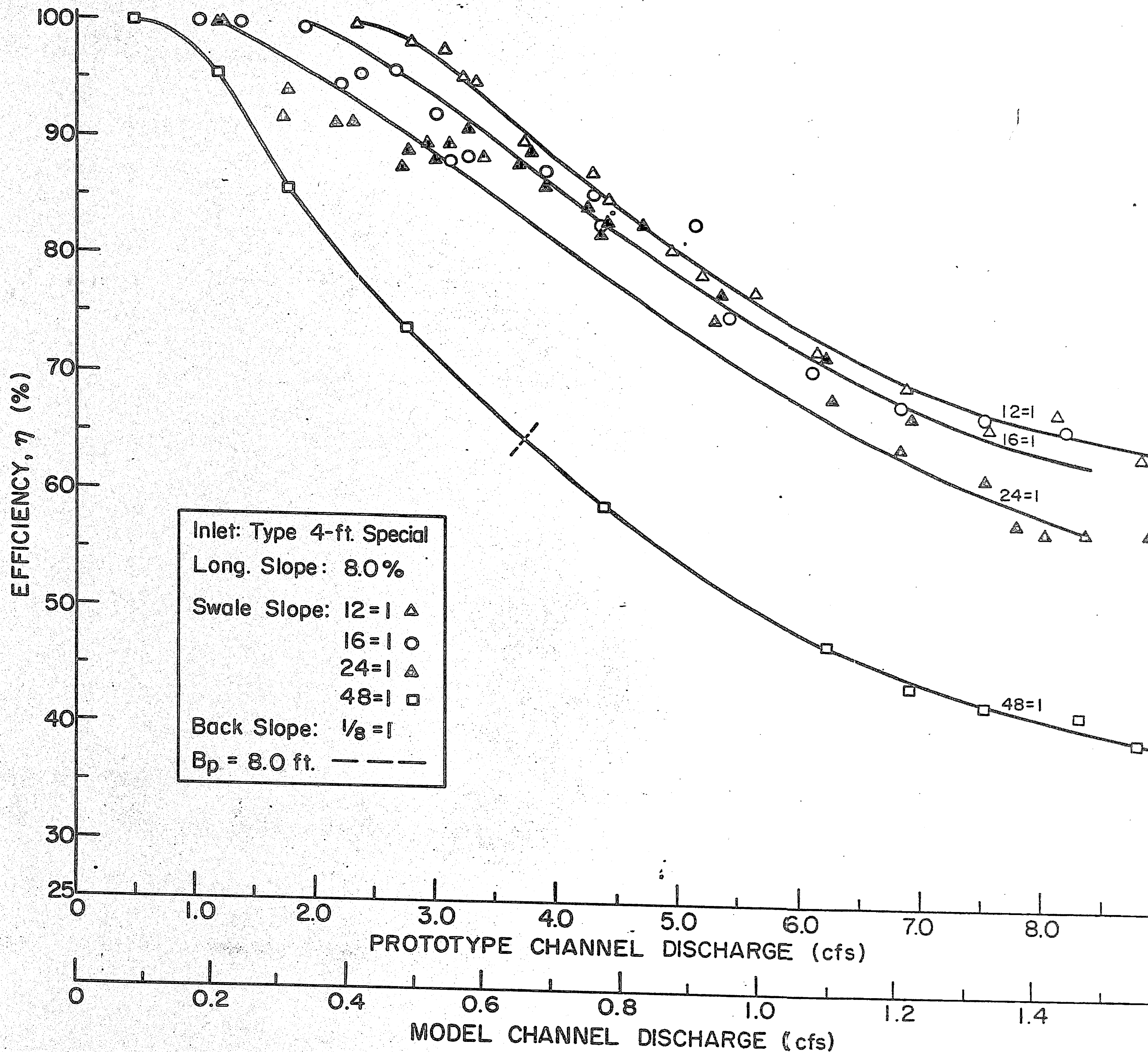
Fig. 4.8 Efficiency Curves; 4-Ft Special (Long. Slope = 8%)
