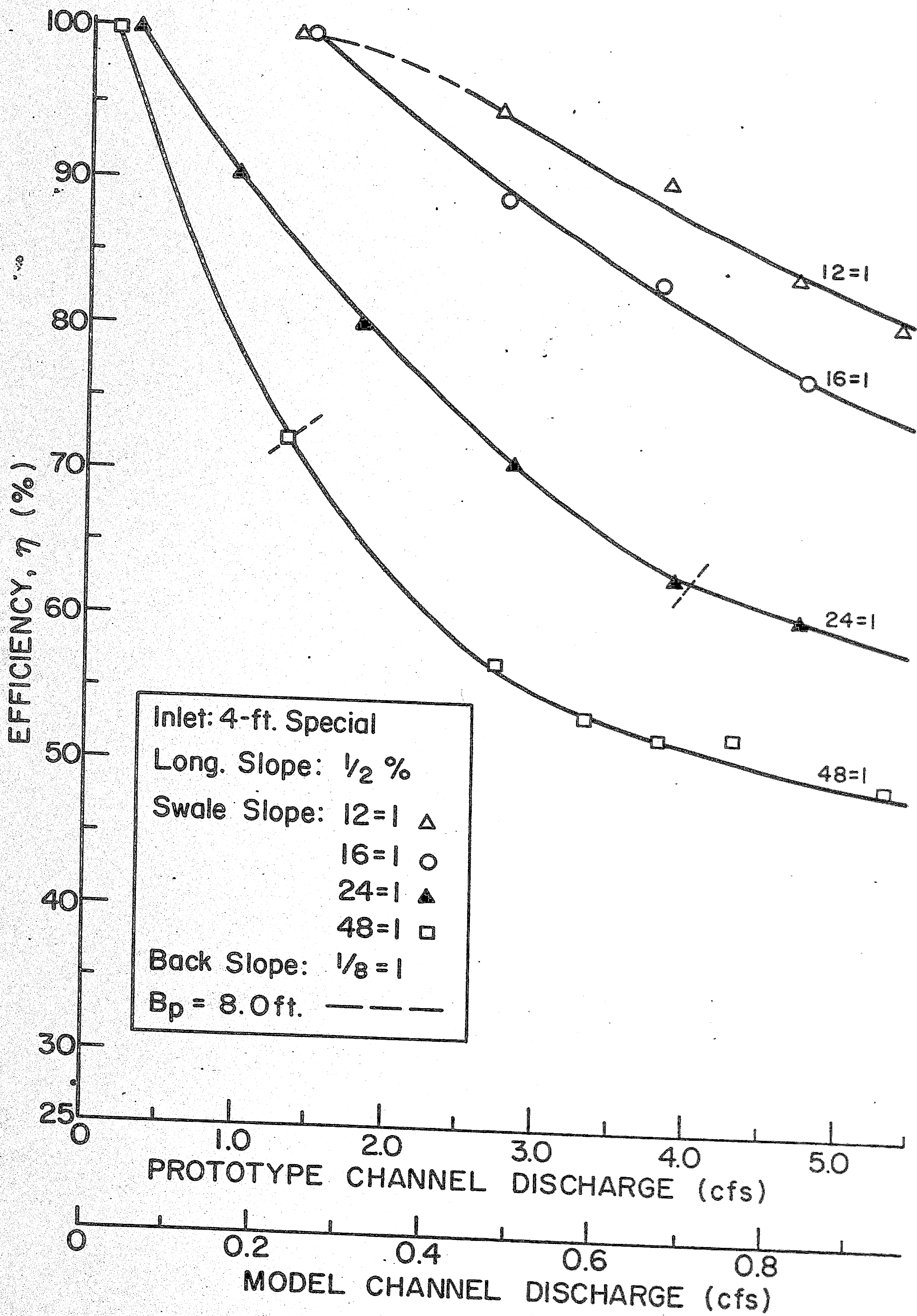
Fig. 4.5 Efficiency Curves; 4-Ft Special (Long. Slope = \frac{1}{2}\% )
