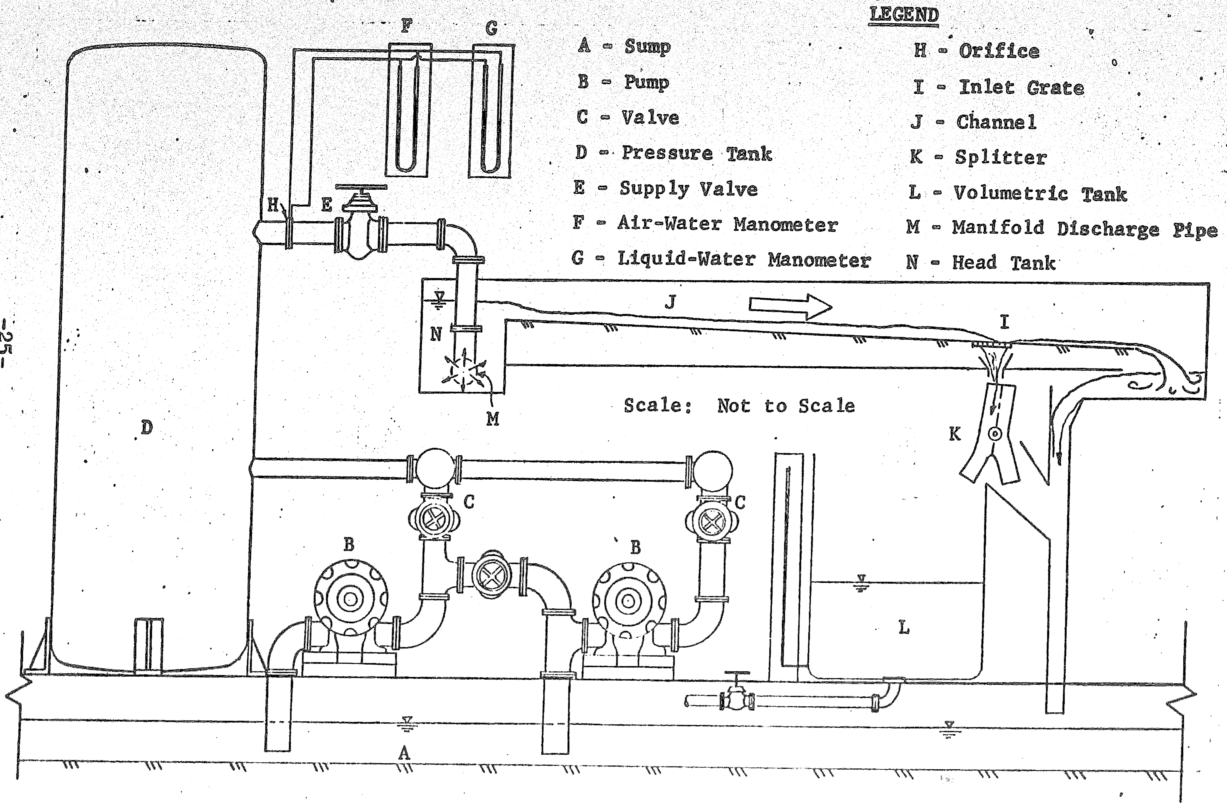
Fig. 3.4 Schematic Diagram
