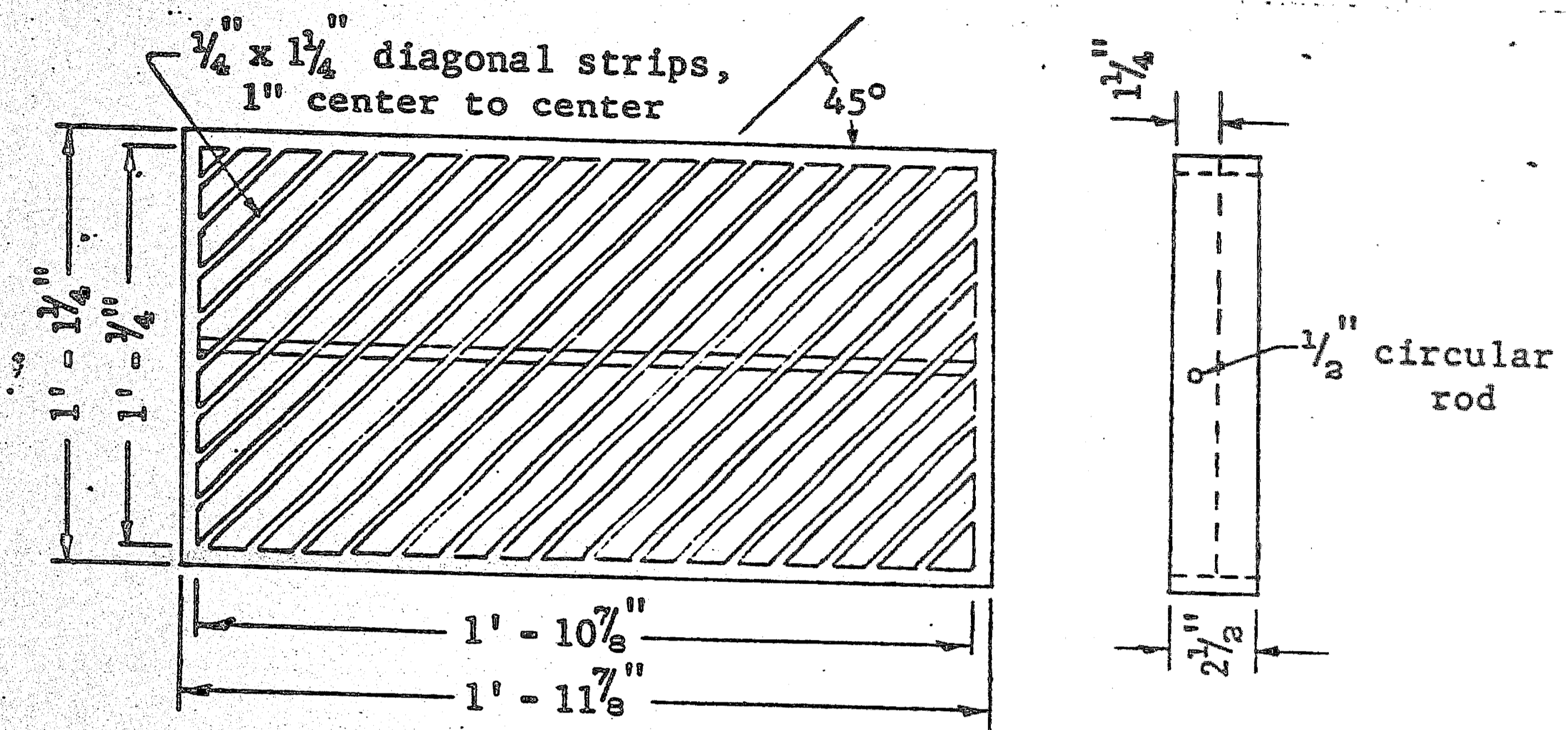
(a) Type 4-Ft Special Inlet
