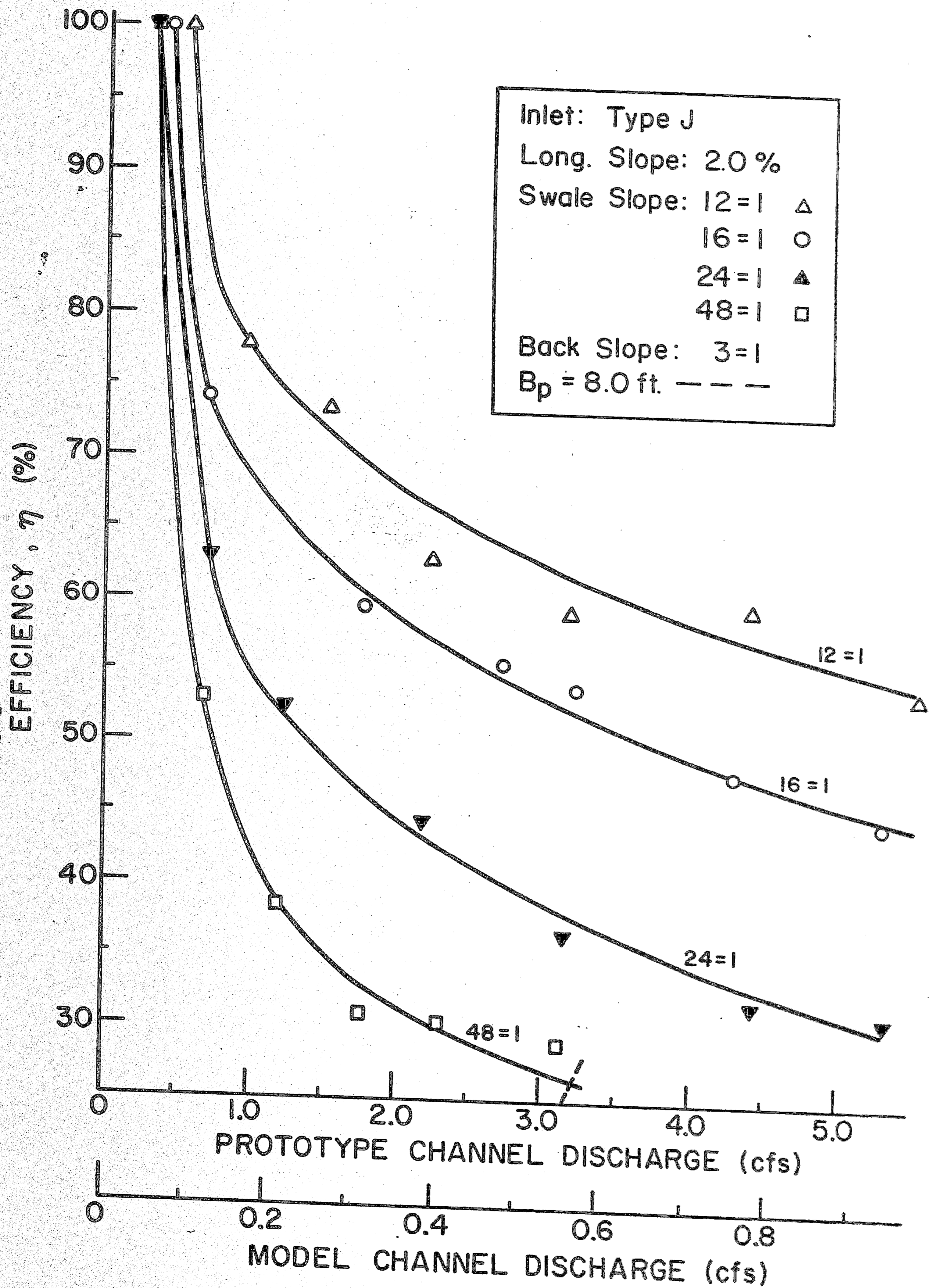
Fig. 4.2 Efficiency Curves; Type J Inlet (Long. Slope = 2%)
