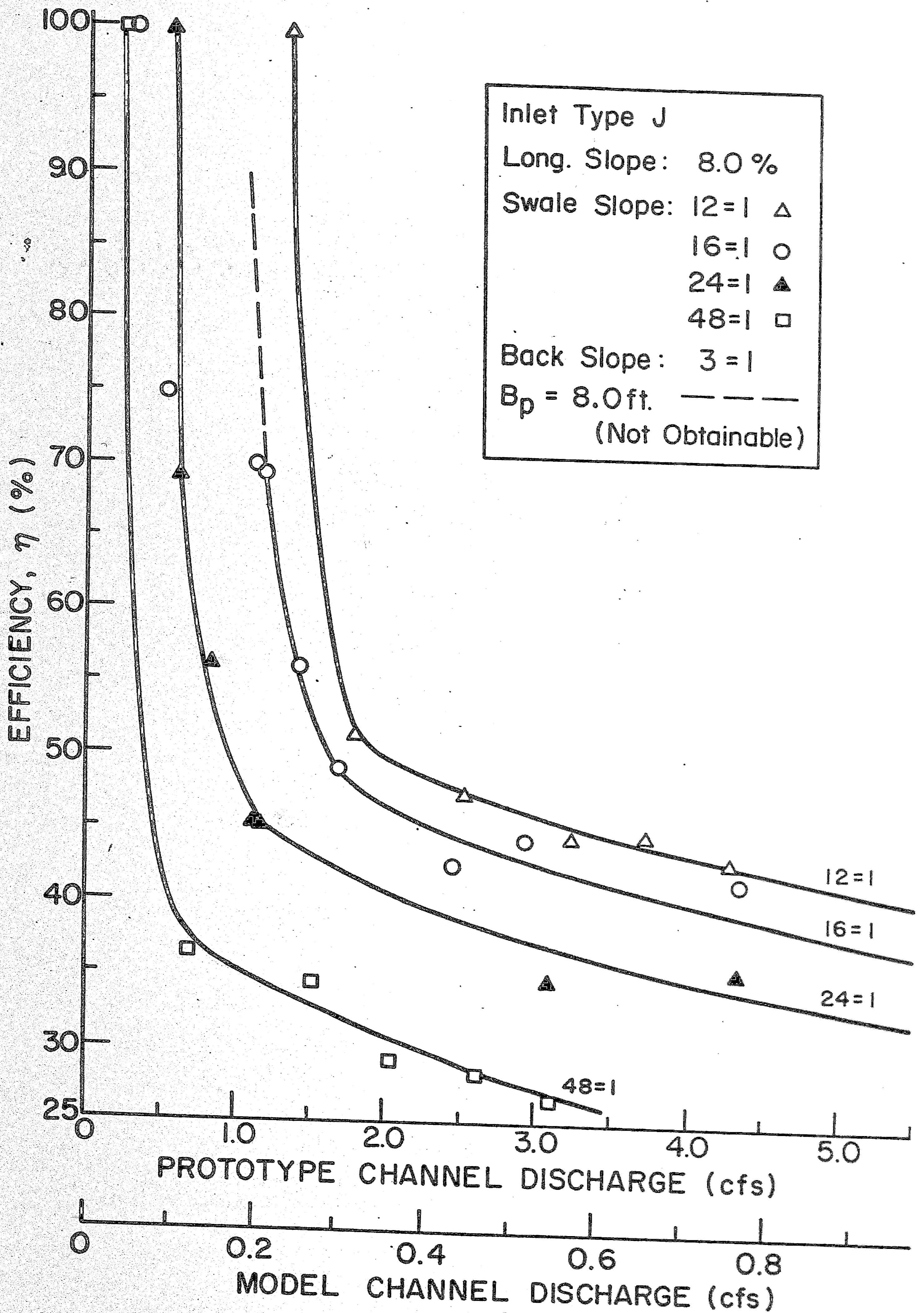
Fig. 4.4 Efficiency Curves; Type J Inlet (Long. Slope = 8%)
