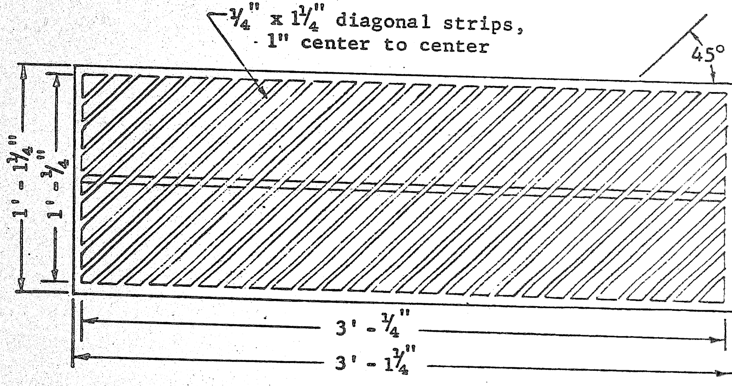
(b) Type 6-Ft Special Inlet
