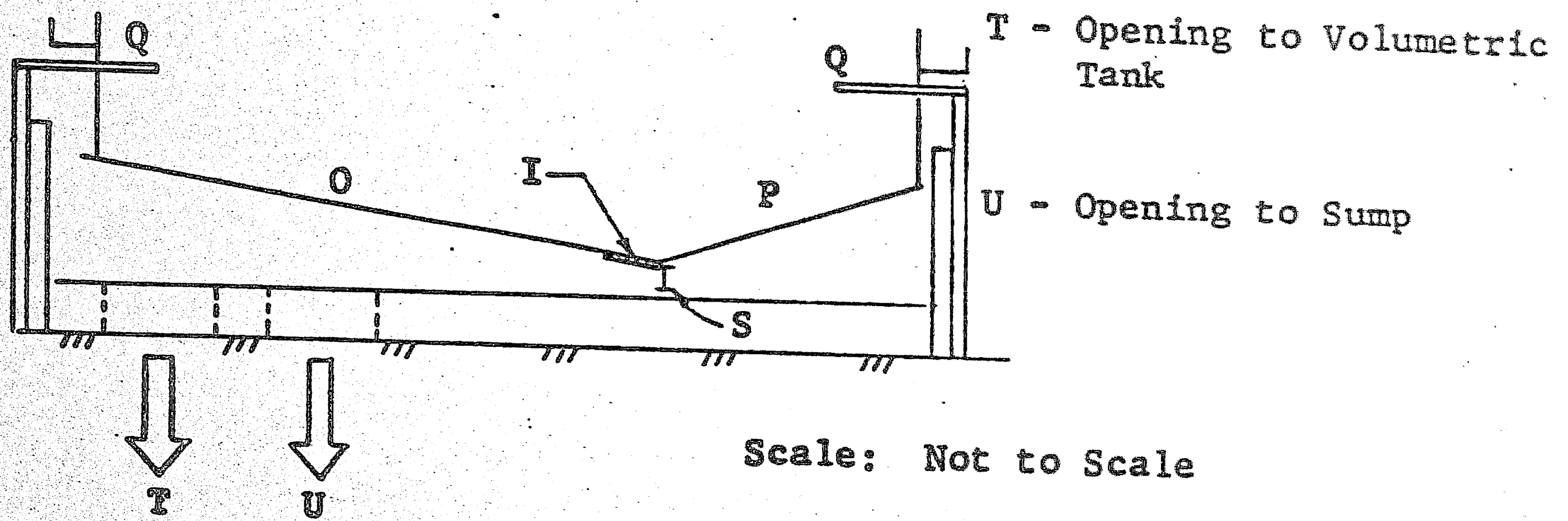
(b) Elevation View
